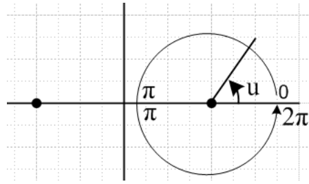
Our bipolar coordinate u u = 0 for |x| > a , increases CCW
