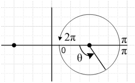
Morse & Feshbach bipolar coordinate \theta \theta = 0 between foci, increases CCW
