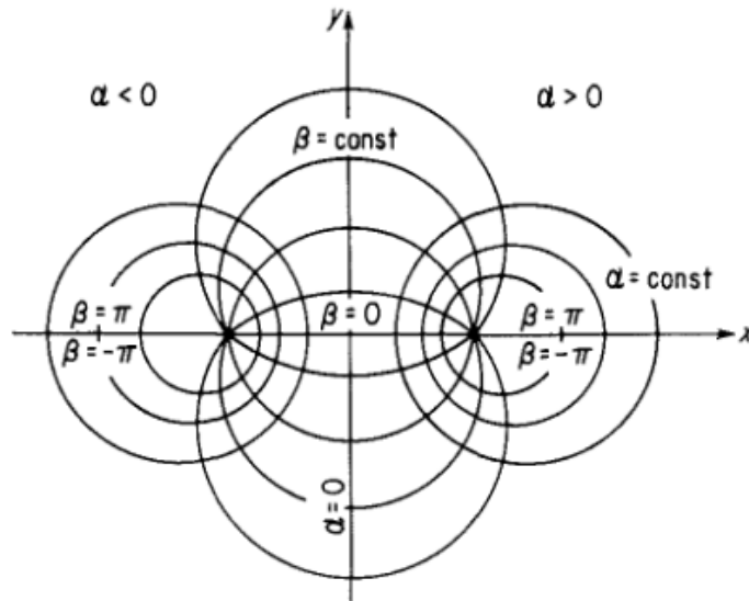
Lebedev et al. bipolar coordinates \alpha and \beta
