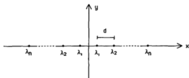
Fig. 16. Array of 2n parallel wires with equal spacing.
