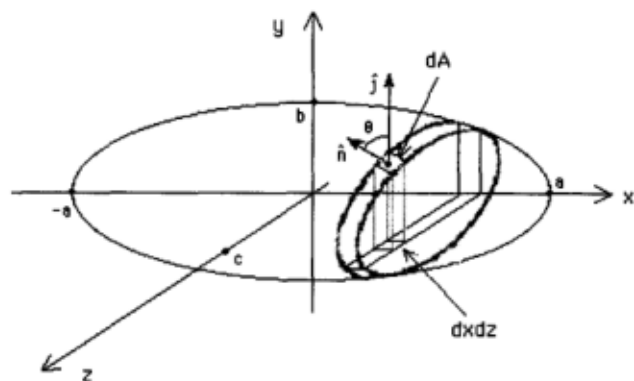
Fig. 2. Conducting ellipsoid.
