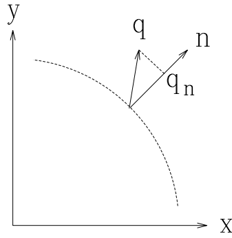
Figure 6.3: Flux vector
