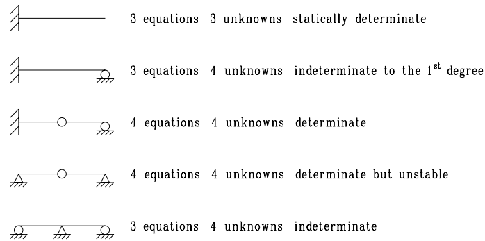
Figure 12.3: Examples of Static Determinate and Indeterminate Structures
