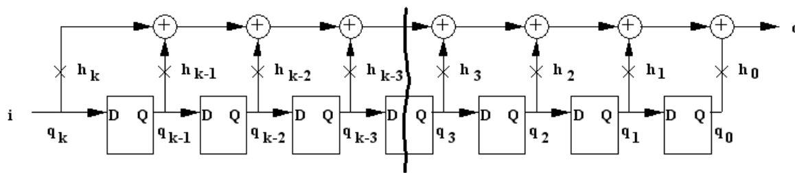
Figure 7: A polynomial multiplier circuit.
