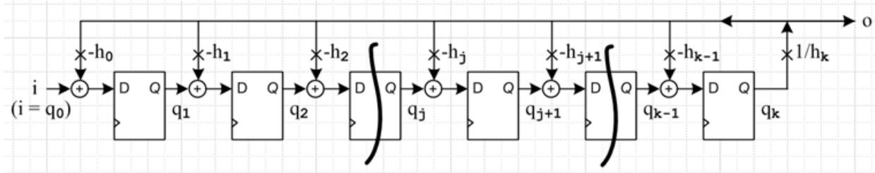
Figure 1.5. Type B polynomial divider.
