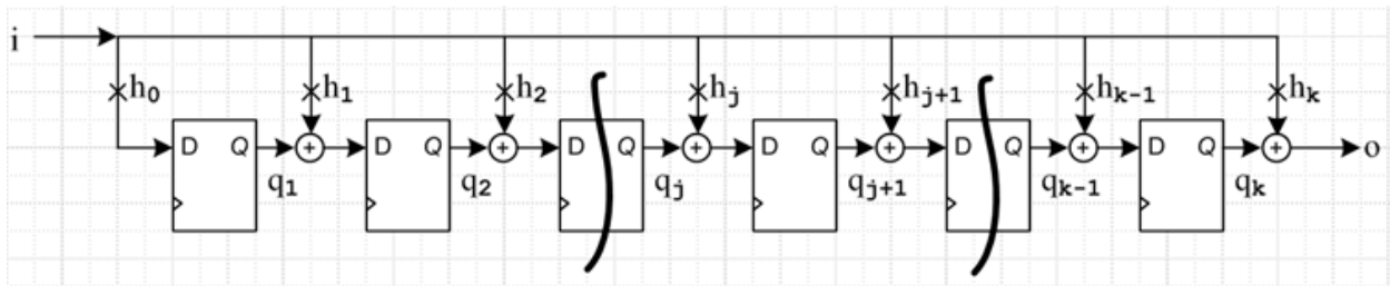
Figure 1.10: Type B polynomial multiplier.
