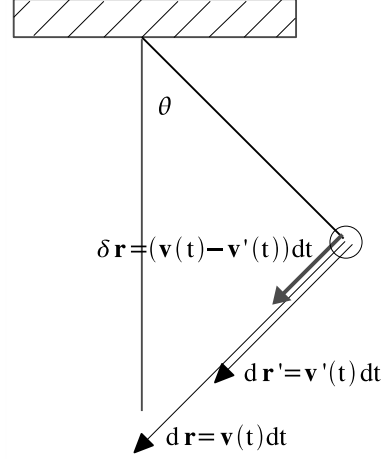
FIG. 4: Allowed and virtual displacements of a pendulum with stationary support
