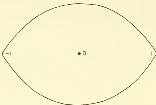
Fig. 24. The domain in which |J_n(nz)| certainly does not exceed unity.
