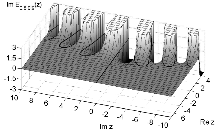
Fig. 1.2 Same as Fig. 1.1 for the imaginary part of E_{0.8,0.9}(z) . The solid line is \operatorname{Im} E_{0.8,0.9}(z) = 0 .
