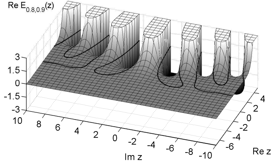
Fig. 1.1 Truncated real part of the generalized Mittag-Leffler function -3 \leq \operatorname{Re} E_{0.8,0.9}(z) \leq 3 for z \in \mathbb{C} with -7 \leq \operatorname{Re} z \leq 5 and -10 \leq \operatorname{Im} z \leq 10 . The solid line is defined by \operatorname{Re} E_{0.8,0.9}(z) = 0 .
