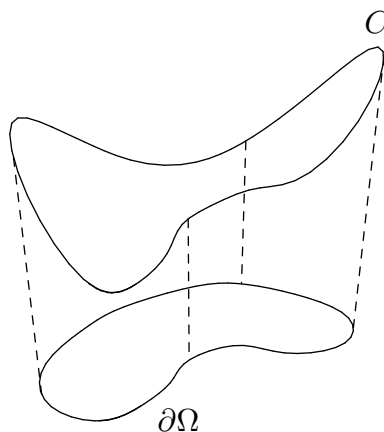
Figure 21.3. Minimal Surface.
