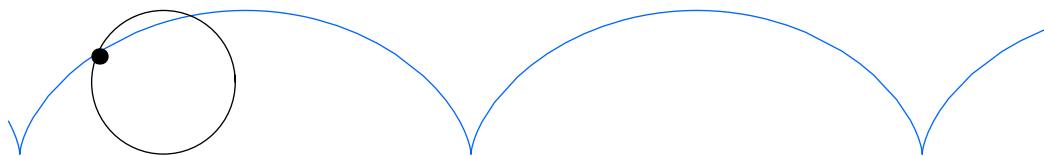
Figure 21.5. A Cycloid.
