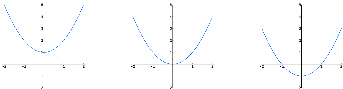
Figure 19.11. Roots of Quadratic Functions.
