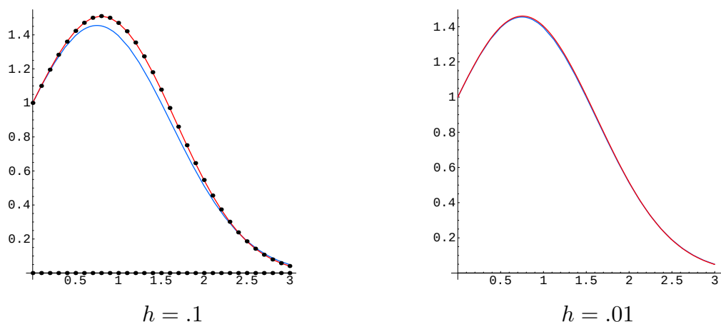
Figure 20.16. Euler's Method for \dot{u} = \left(1 - \frac{4}{3}t\right)u .
