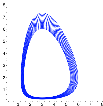
Euler Method, h = .001
