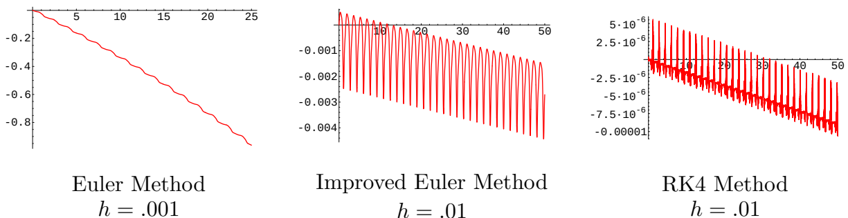
Figure 20.19. Numerical Evaluation of Lotka–Volterra First Integral.
