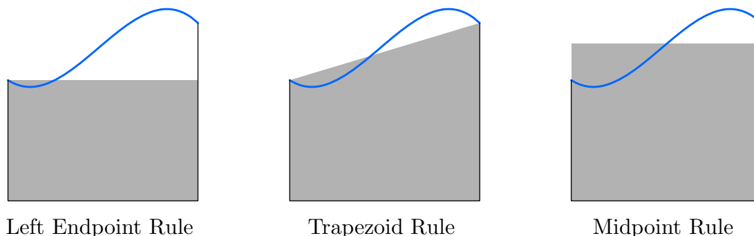
Figure 20.17. Numerical Integration Methods.
