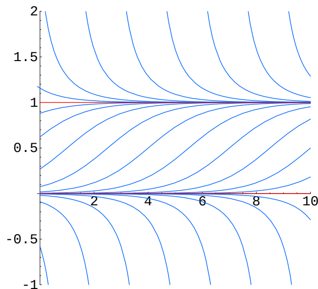
Figure 20.2. Solutions to u' = u(1 - u) .
