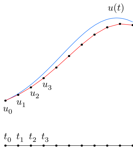
Figure 20.15. Euler's Method.
