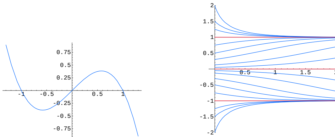
Figure 20.7. Stability of \dot{u} = u - u^3 .
