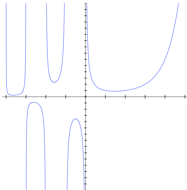
Figure C.1. The Gamma Function.
