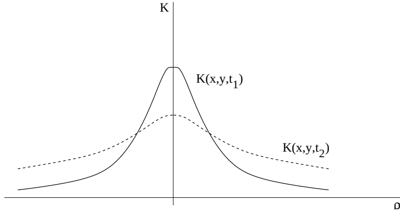
Figure 6.1: Kernel K(x, y, t) , \rho = |x - y| , t_1 < t_2
