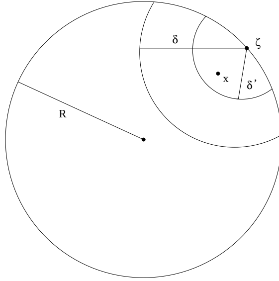
Figure 7.6: Proof of Theorem 7.2
