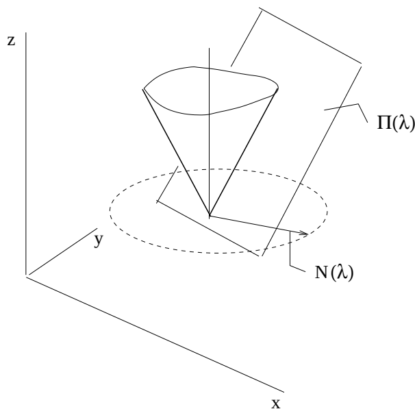
Figure 2.9: Monge cone in an example
