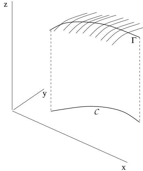
Figure 2.4: Cauchy initial value problem
