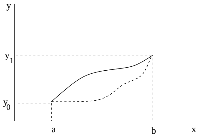
Figure 1.5: Admissible variations
