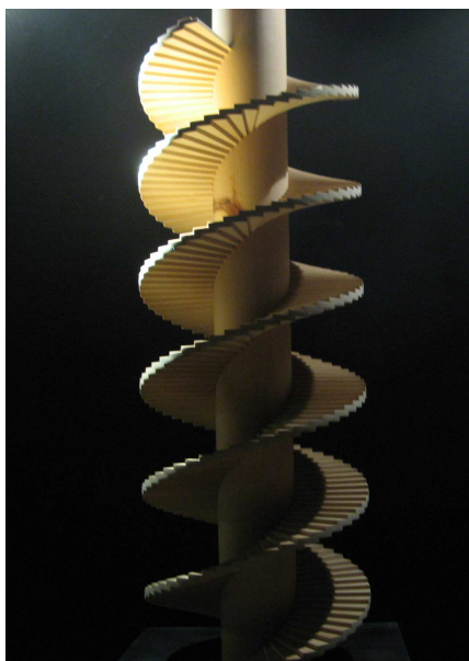
Figure 2.3: Right helicoid, a^2 < x^2 + y^2 < R^2 (Museo Ideale Leonardo da Vinci, Italy)
