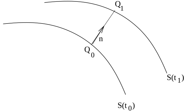
Figure 3.5: Definition of the speed of a surface
