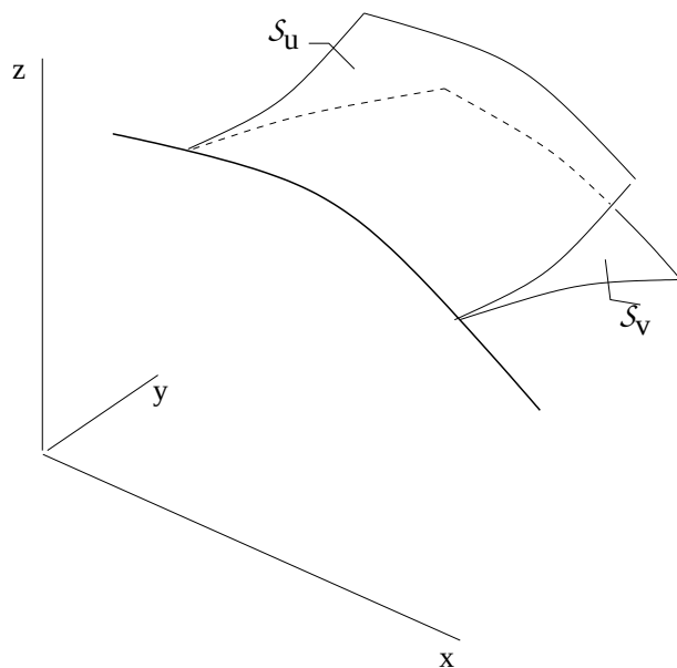
Figure 2.6: Multiple solutions
