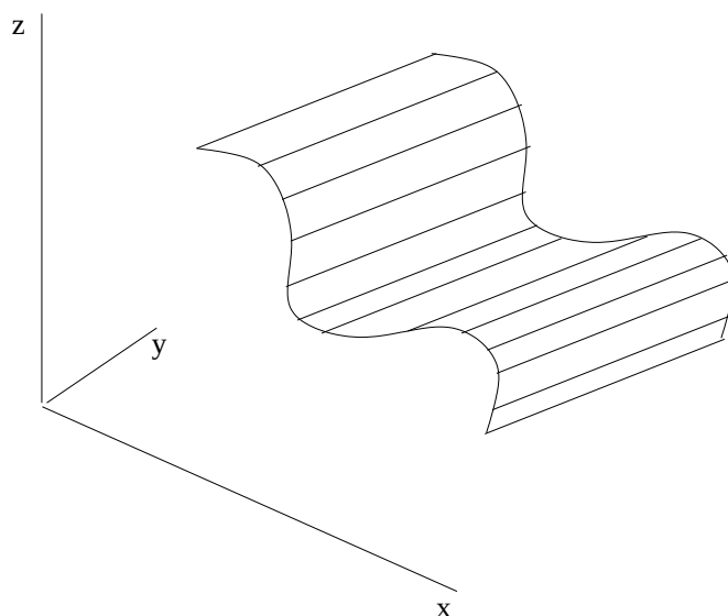
Figure 2.2: Cylinder surfaces
