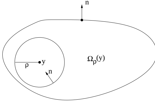
Figure 7.2: Notations to Theorem 7.1
