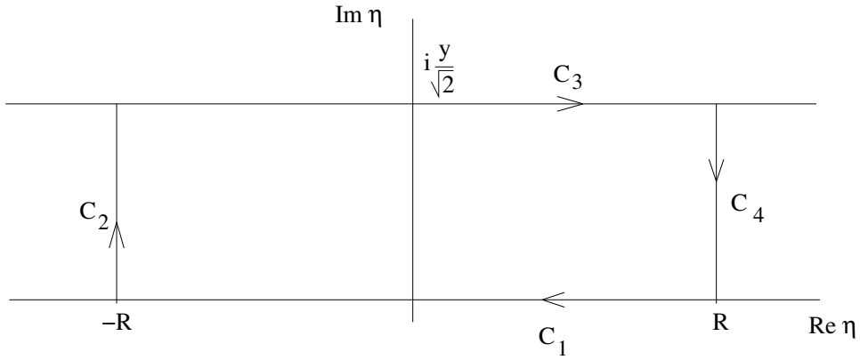
Figure 5.1: Proof of (5.8)
