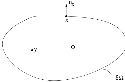
Figure 7.1: Notations to Green's identity
