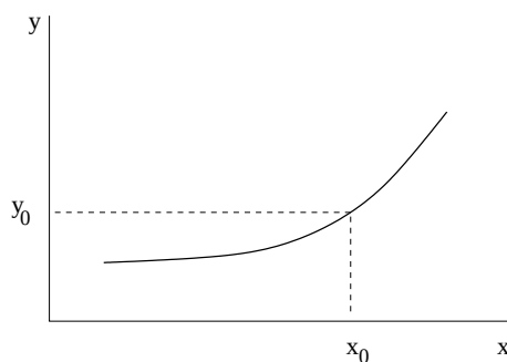
Figure 1.1: Initial value problem
