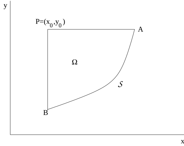
Figure 4.6: Riemann's method, domain of integration
