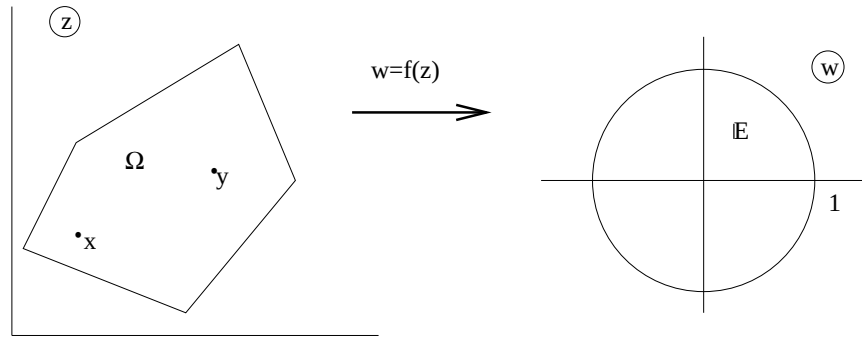
Figure 7.7: Conformal mapping
