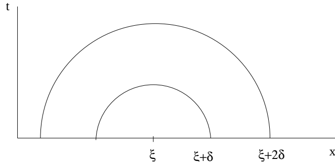
Figure 6.2: Figure to the proof of Theorem 6.1
