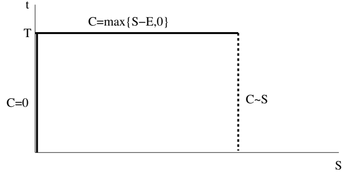
Figure 6.5: Side conditions for a call option
