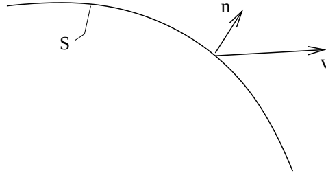
Figure 3.6: Definition of relative speed
