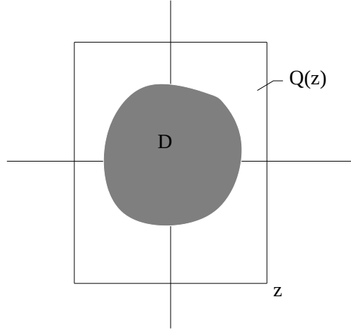
Figure 3.7: Definition of D \in Q(z)
