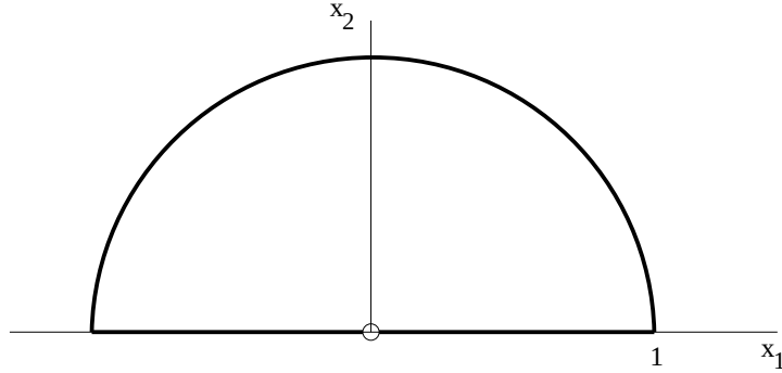
Figure 7.3: Counterexample
