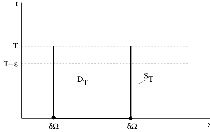
Figure 6.3: Notations to the maximum principle
