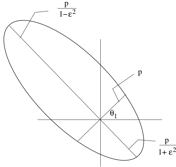
Figure 2.14: The case of an ellipse
