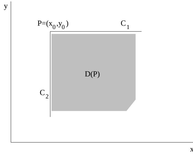
Figure 4.7: Definition of Riemann's function
