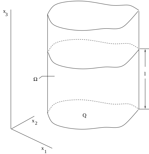
Figure 6.4: Diffusion in a tube
