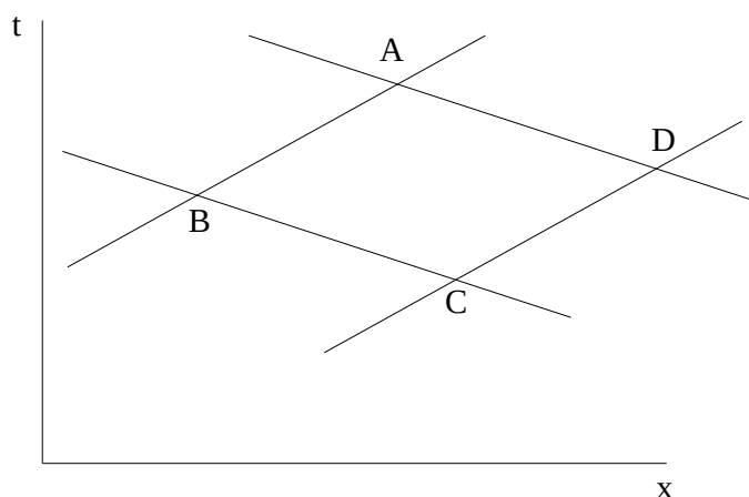
Figure 4.8: Figure to the exercise
