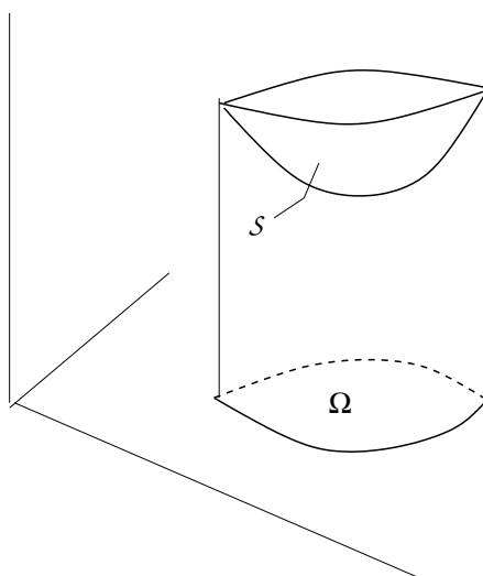
Figure 1.6: Comparison surface
