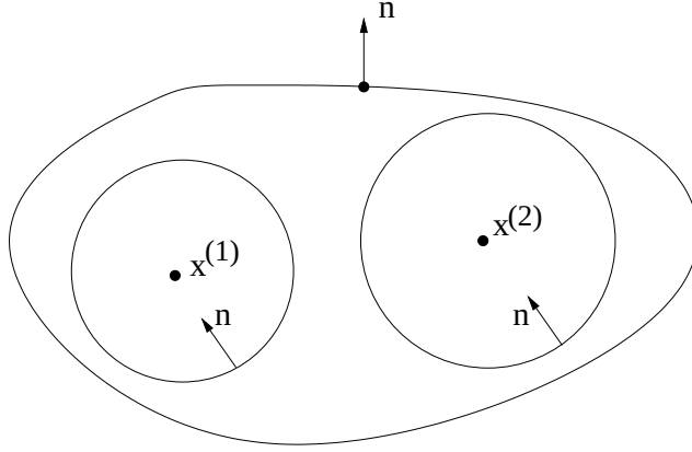
Figure 7.4: Proof of Proposition 7.7
