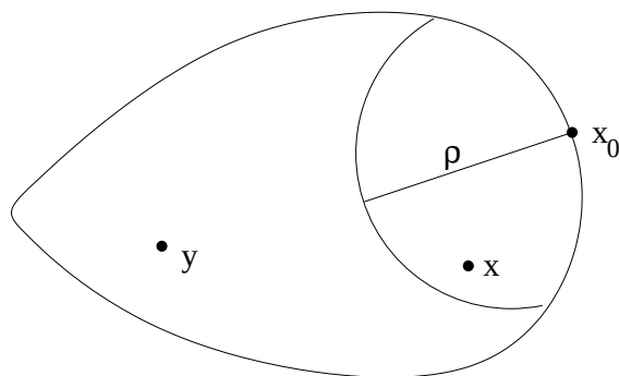
Figure 7.8: Proof of Theorem 7.3
