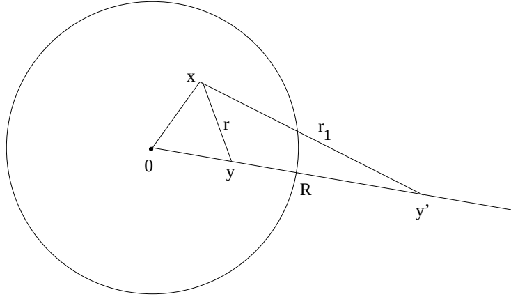
Figure 7.5: Reflection on \partial B_R(0)
