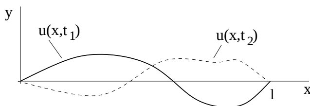
Figure 1.4: Oscillating string
