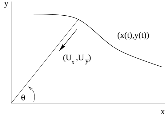
Figure 2.13: Motion in a central field
