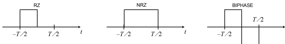
Fig. 19-2. Return-to-zero (RZ), non-return-to-zero (NRZ), and biphaser pulses.
