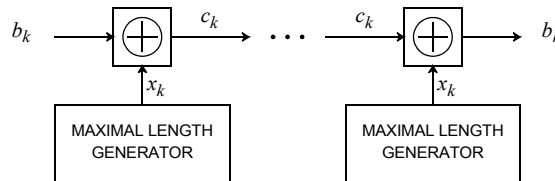
Fig. 19-19. A frame-synchronized scrambler where the maximal-length generator is as in Fig. 19-18.
