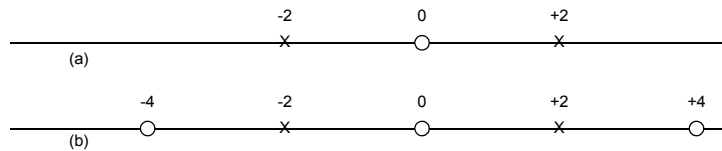
Fig. 19-14. A three-point (a) and five-point (b) signal constellation consisting of even integers. Points in set \Omega_0 are marked “o,” and points in set \Omega_1 are marked “x.”
