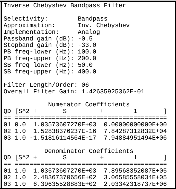
Figure 3.6 Filter coefficients for Example 3.6 from WFilter.
