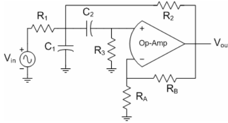
Figure 4.8 Sallen-Key bandpass active filter stage.
