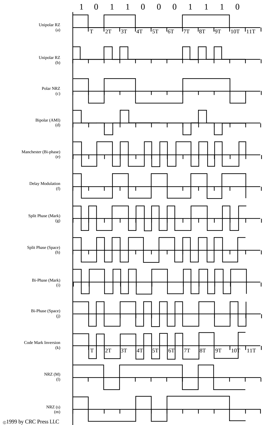
FIGURE 6.1: Waveforms for different line codes.
