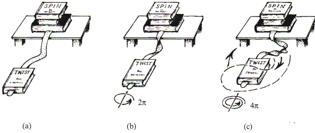
Figure 7. Spinorial Book
