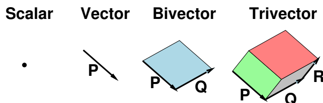
Figure 1: Scalar, Vector, Bivector, and Trivector
