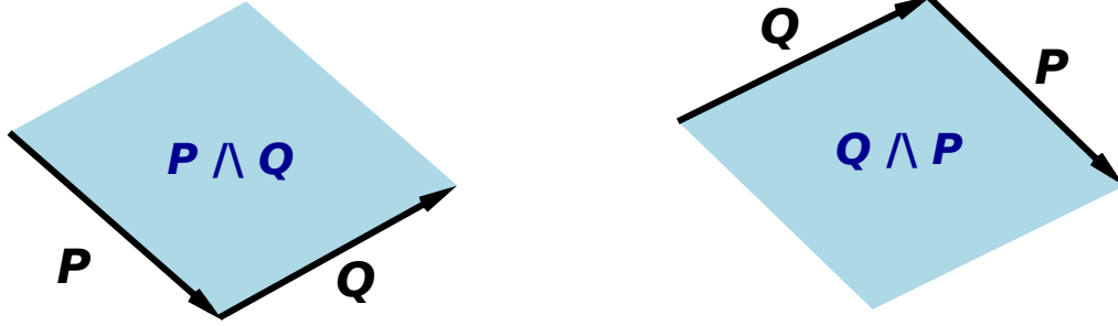
Figure 4: Bivectors: Direction of Circulation
