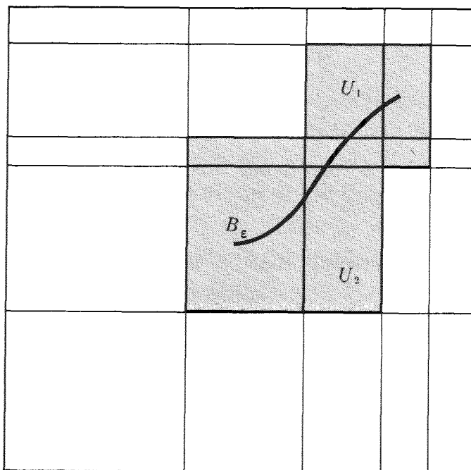
FIGURE 3-1. The shaded rectangles are in S_1 .
