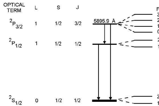
FIG. 11.9. The development of hyperfine lines in an optical spectrum of sodium due to the nuclear spin I , which enters through F = J + I .
