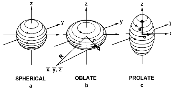
FIG. 11.6. Three nuclear shapes: (a) spherical nucleus, (b) oblate (extended at the equator), and (c) prolate (extended at the poles).
