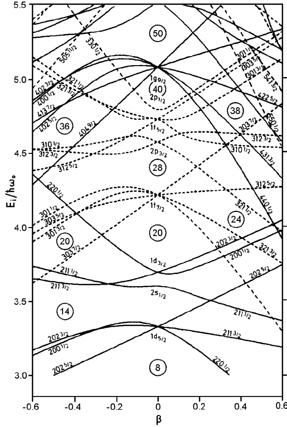
FIG. 11.8. Nilsson diagram of single-particle energy levels for deformed nuclei. The energy scale is in units of \hbar\omega_0 ( \hbar\omega_0 is approximately 41A^{-1/6} MeV). The figures along the center give the neutron or proton numbers and l-j values for the single nucleon. The figure combinations at the end of the lines are approximate quantum numbers; the first figure is the principal quantum number n . Full-drawn lines are for even parity, broken lines for odd. (From Larsson, Leander, Ragnarsson and Alenius.)
