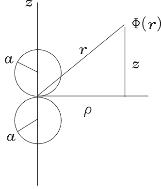
Figure 2-17: Geometry in the original space.
