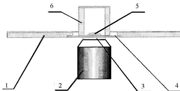
1. Glass coverslip holder 2. Fluorescence objective (40X) 3. Water 4. Glass coverslip 5. Droplet 6. Sealing cylinder cap
