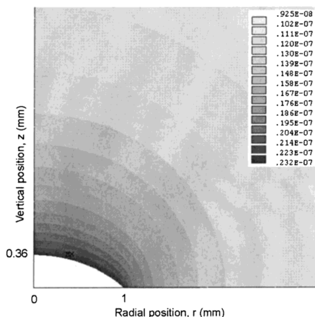
Figure 5. Contour plot of the vapor concentration distribution above a droplet of radius R = 1 mm and height h_0 = 0.364 mm. The parameters used in the FEM method are vapor diffusivity D = 26.1\text{ mm}^2/\text{s} , relative humidity H = 0.40 (i.e., 40%), and saturated vapor concentration on the droplet surface c_v = 2.32 \times 10^{-8}\text{ g/mm}^3 , which is the value obtained from the CRC Handbook 16 at 25\text{ }^\circ\text{C} . These parameter values are also used in Figures 6–10. The gray bars represent the vapor concentration in \text{g/mm}^3 .
