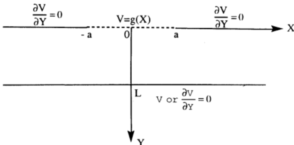
FIG. 1. Physical configuration.
