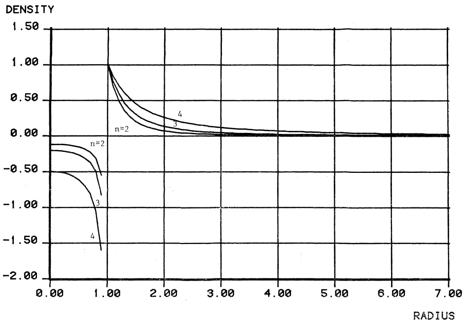
Fig. 4. Charge density for n = 2, 3, 4 ,
