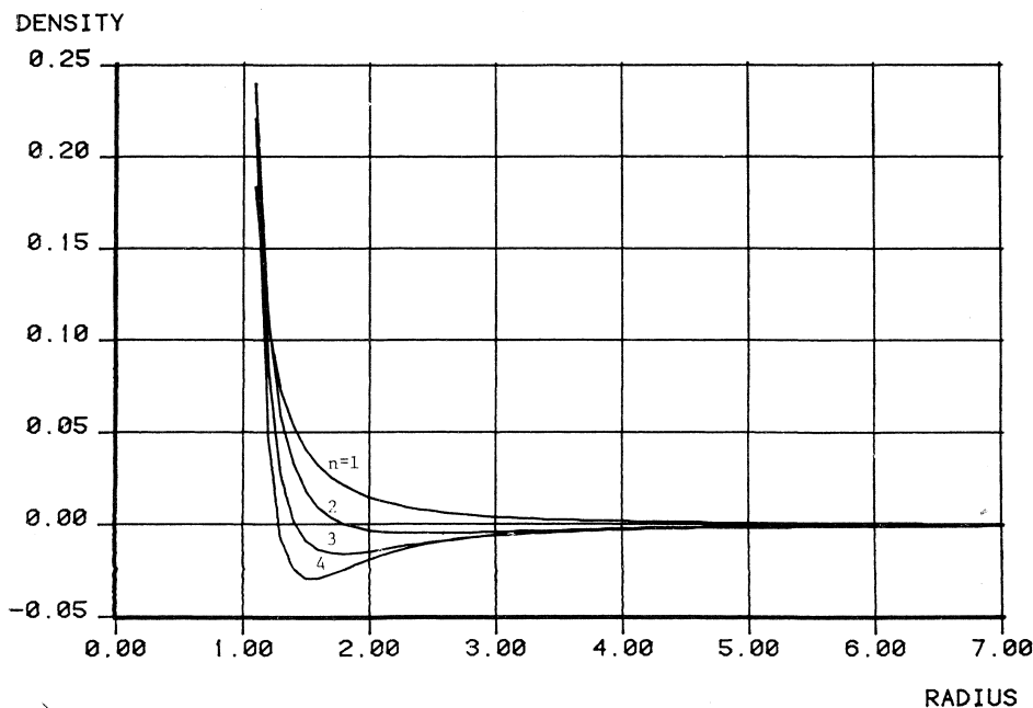
Fig. 1. Charge density for n = 1, 2, 3, 4
