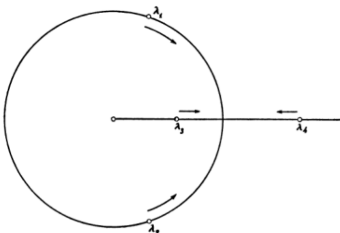
FIG. 1. Position of the characteristic values for the general case a) in the complex plane. In case b), \lambda_3 and \lambda_4 coincide and are equal 1; in case c), \lambda_1 and \lambda_2 coincide and are either +1 or -1. In case d) both pairs \lambda_3 = \lambda_4 = 1 and \lambda_1 = \lambda_2 = \pm 1 coincide.
