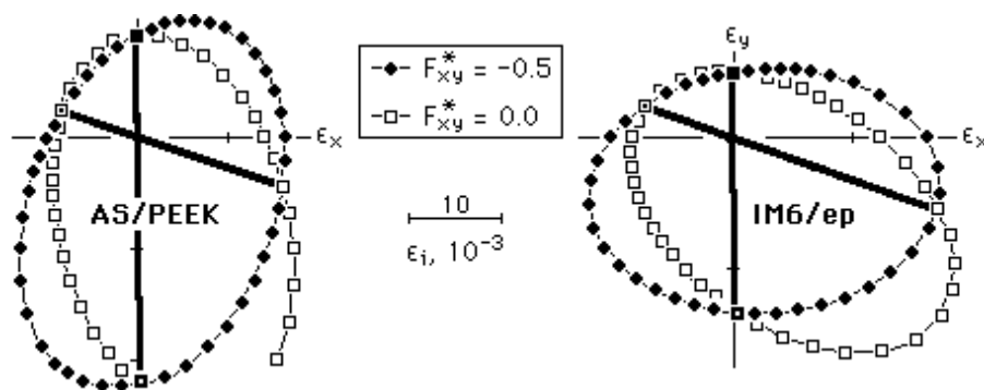
FIGURE 8.23 TSAI-WU ENVELOPES IN STRAIN SPACE FOR AS/PEEK AND IM6/EPOXY COMPOSITES
