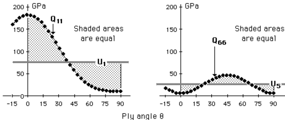
FIGURE 3.14 THE INVARIANTS OF THE "11" AND "66" COMPONENTS
