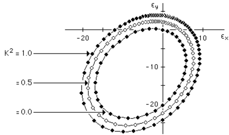
FIGURE 8.31 LOCI OF CONSTANT FEA INDEX IN STRAIN SPACE FOR T300/5208
