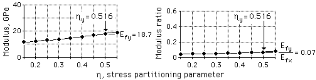
FIGURE 7.5 THE ABSOLUTE AND NORMALIZED TRANSVERSE STIFFNESS OF THE GRAPHITE FIBER IN A T-300/5208 PLY MATERIAL DERIVED FROM THE PARTITIONING PARAMETER
