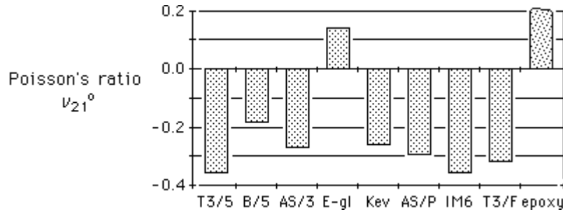
FIGURE 4.17 POISSON'S RATIOS OF [15_2/60]_s LAMINATES
