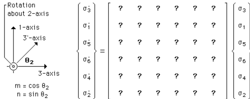
FIGURE 2.20 STRESS TRANSFORMATION BY A ROTATION ABOUT THE 2-AXIS
