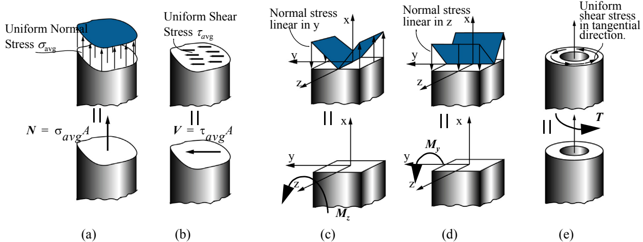
Figure 1.16 Static equivalency.
