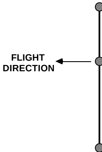
Figure 4.9 Example Configuration of 1-D, Gravity-Gradient-Stabilized, Vertical Constellation
