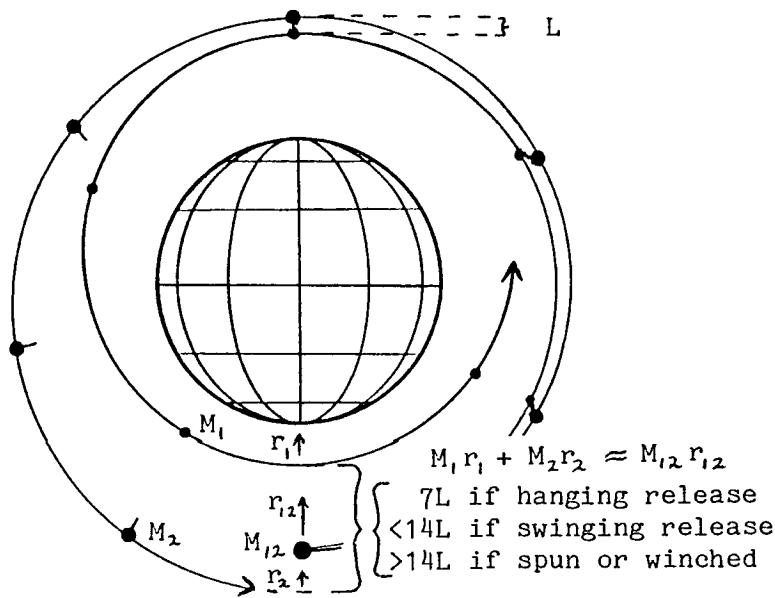
Effects of Tether Deployment and Release
