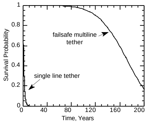
Lifetime comparison of equal-weight single line and failsafe multiline tethers for a low-load mission.
