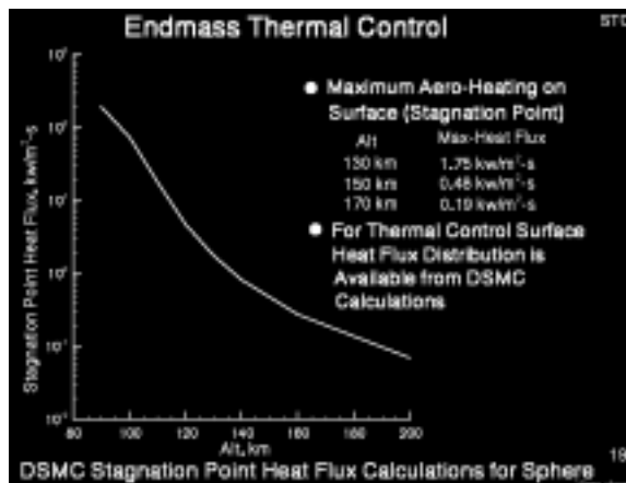
Fig. 8. ATM endmass thermal control
