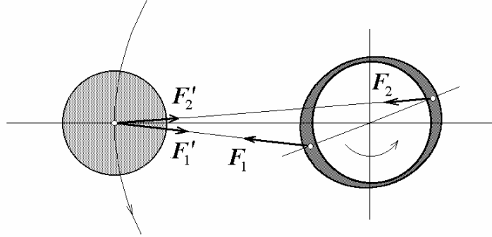
Figure 4. Gravitational interaction between the moon and the tidal bulges.
