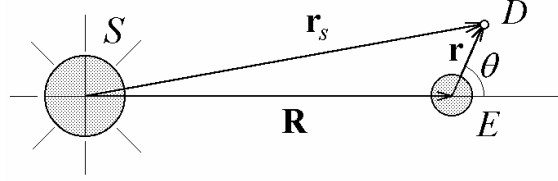
Figure 2. For calculation of the tide-generating force at arbitrary point D .
