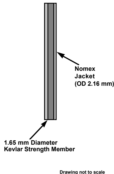
Fig. 9. A magnification of the baseline tether.
