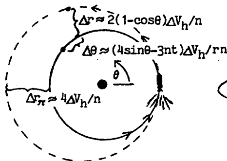
Effects of Small \Delta V s on Near-Circular Orbits
