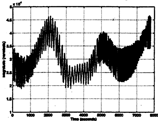
Figure 1.13d. EMP Magnetometer Modulus
