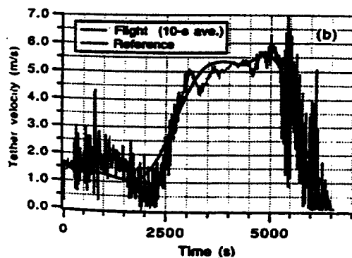
Figure 1.14a. Tether Rate
