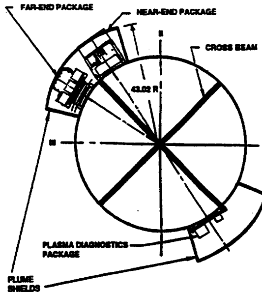
Figure 1.16 PMG Major hardware components
