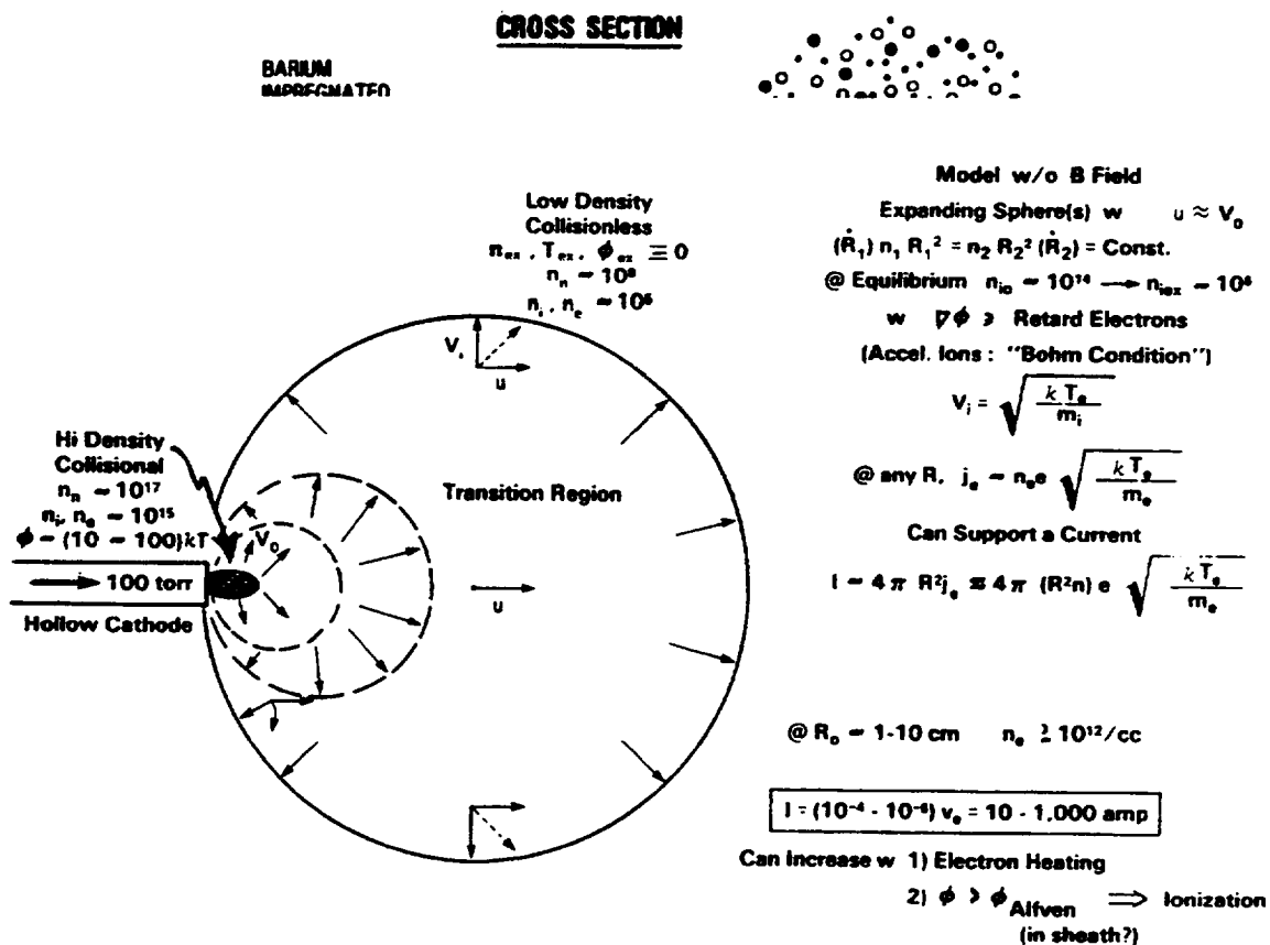
Figure 4.20 Diagrams of a Hollow Cathode Plasma Contactor
