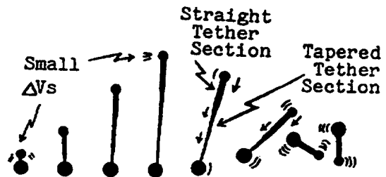
One Spin-Up Technique For Use in Deep Space
