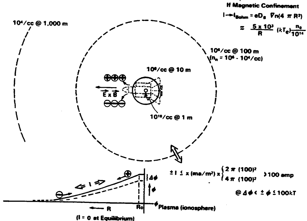
Figure 4.23 Electron Current Flow To/From the Ionosphere for PMG Hollow Cathode Plasma Contactor
