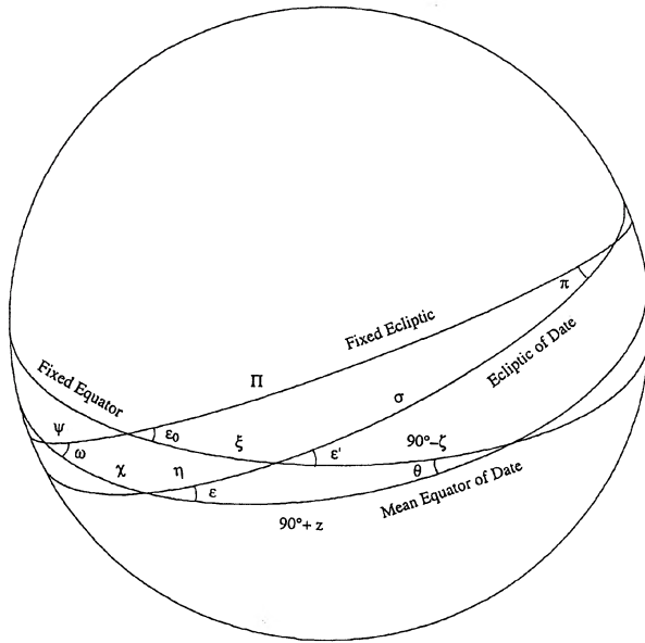
FIG. 1. Relation between the fixed equator (mean equator) and fixed ecliptic of J2000 and the moving (mean of date) equator and ecliptic. The arc from the moving equinox to the node of the moving ecliptic on the fixed ecliptic is \Lambda_A = \Pi_A + p_A = \sigma_A + \eta_A . The subscript A is not used with symbols in the figure.
