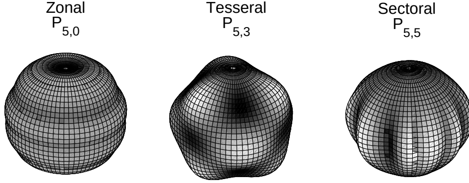
Figure 2.15: Zonal, tesseral and sectoral spherical harmonics.
