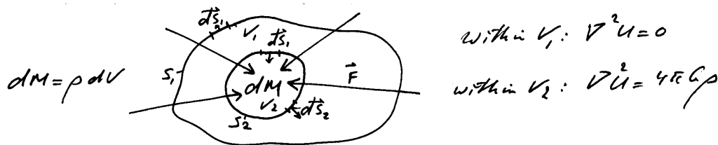
Figure 2.11: Applicability of Poisson's and Laplace's equations.
