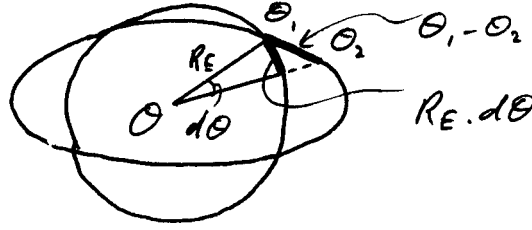
Figure 2.5: Ellipticity of the Earth measured by the distance between latitudes of the Earth and a sphere.
