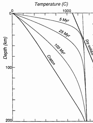
Figure 2. Representative geotherms, illustrating the cool thermal boundary layer at the earth's surface. Three oceanic geotherms are included, corresponding to sea-floor ages of 5, 25, and 100 Ma. The "craton" geotherm represents relatively thick continental lithosphere. A dry mantle solidus (McKenzie and Bickle 1988) is included, along with the extrapolation of the adiabat (gradient 0.3^\circ\text{K/km} ) to the surface.
