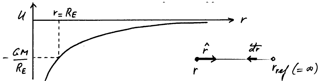
Figure 2.3: By definition, the potential is zero at infinity and decreases towards the mass.
