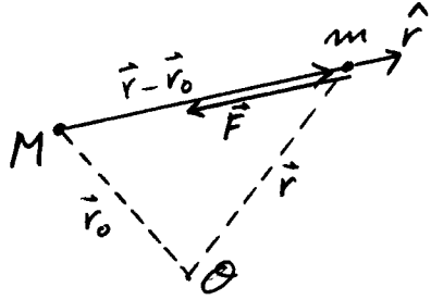
Figure 2.1: Vector diagram showing the geometry of the gravitational attraction.
