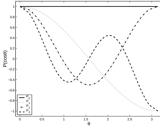
Figure 2.13: Legendre polynomials.
