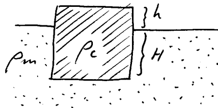
Figure 2.19: Airy isostasy.
