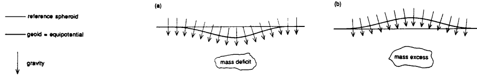
Figure 2.16: Mass deficit leads to geoid undulation.
