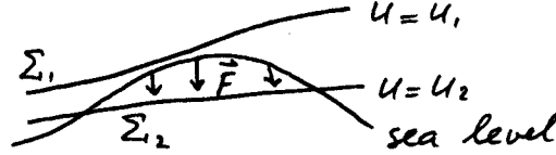
Figure 2.4: F = -m\nabla U provides the restoring force that levels the sea surface along an equipotential surface.
