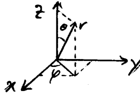
Figure 2.12: Definition of r , \theta and \varphi in the spherical coordinate system.
