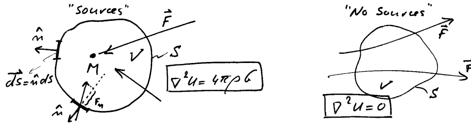
Figure 2.10: Poisson's and Laplace's equations.
