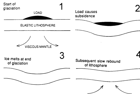
Figure 5.16. The deformation and uplift which occur as a result of loading and unloading of an elastic lithospheric plate overlying a viscous mantle.
