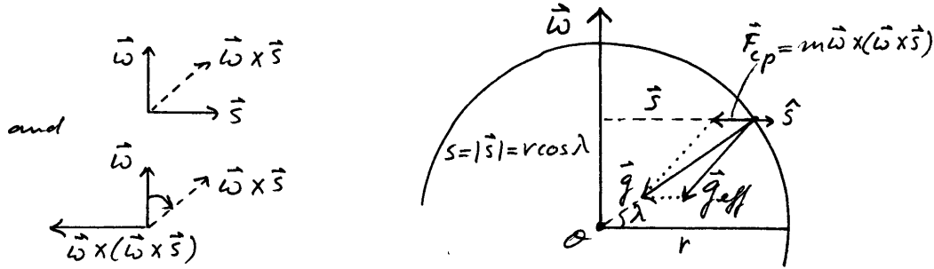
Figure 2.8: The gravitational attraction delivers the centripetal force needed to sustain the rotation of the Earth.
