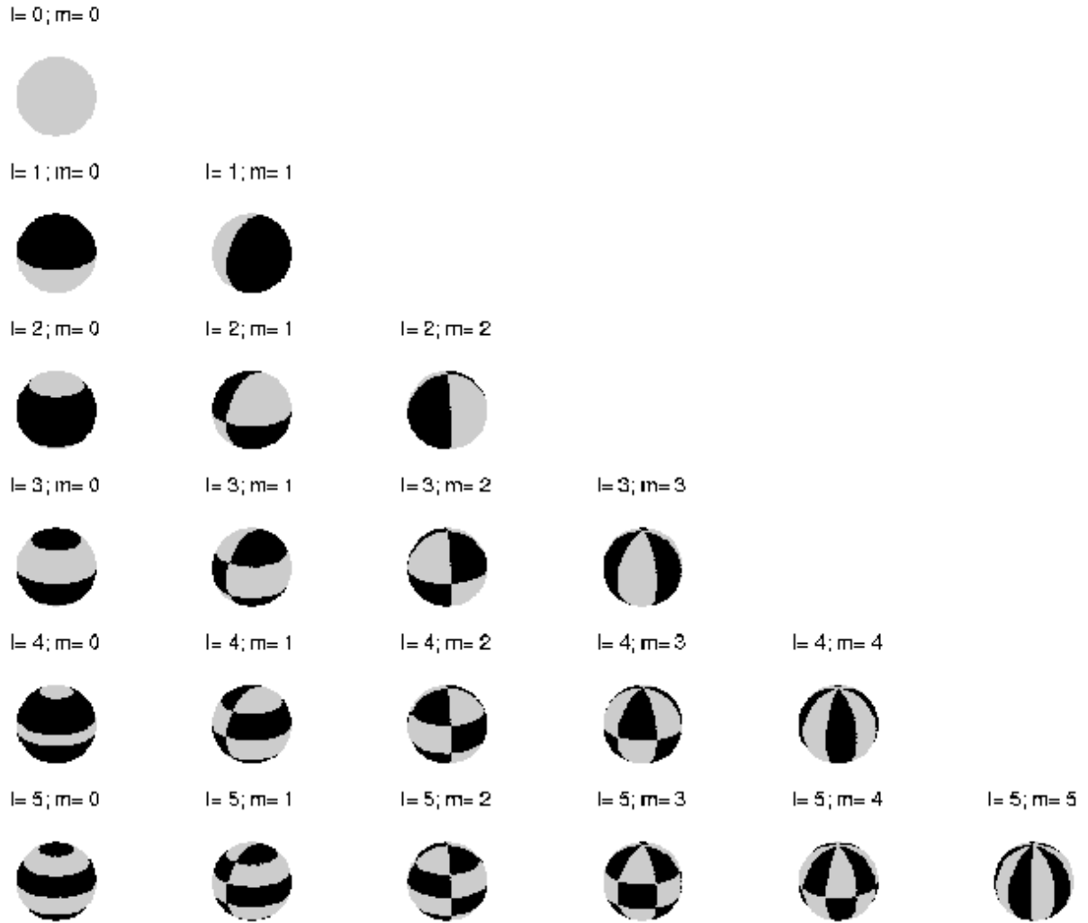
Figure 2.14: Some spherical harmonics.
