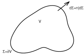
Figure 2.9: Surface enclosing a volume. Unit normal vector.
