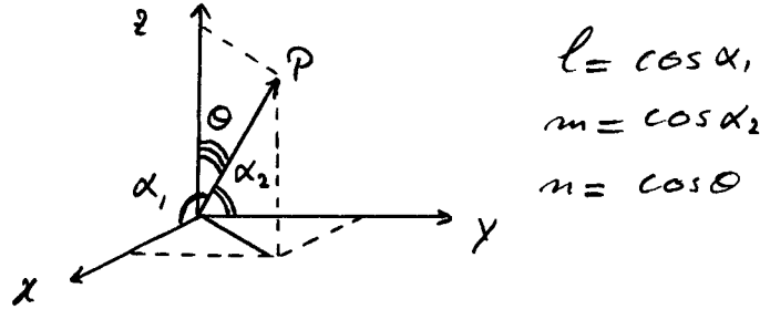
Figure 2.7: Definition of direction cosines.
