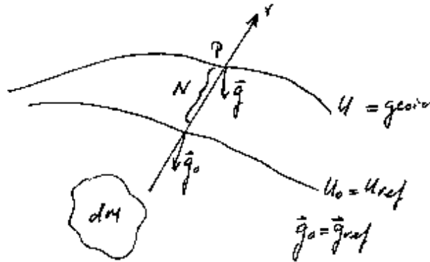
Figure 2.17: Derivation. Note that in this figure, the sign convention for the gravity is reversed; we have used and are using that the gravity is the negative gradient of the potential.
