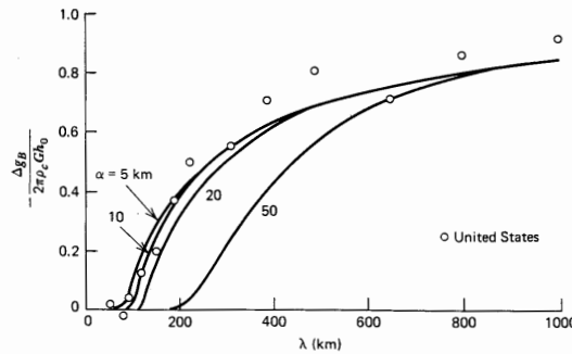
Figure 5-17 Correlation of Bouguer gravity anomalies with topography for the United States (after L. M. Dorman and B. T. R. Lewis, J. Geophys. Res. , 77 , 3068–3077, 1972) compared with Equation (5-130).
