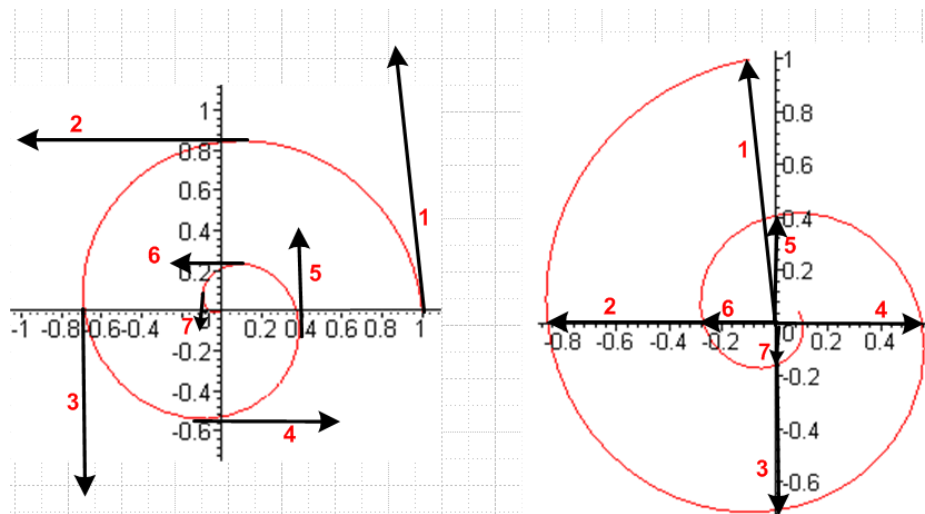
\omega = 1 plot of \mathbf{r}(t)
