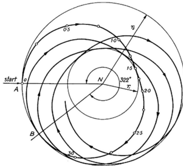
Fig. 6.4. Herpolhode for body of moments of inertia A = 50 , B = 31 , C = 16 . Initial conditions h^2 = 3860 , 2T = 135 ( h^2 < 2BT ). Figures on curve indicate time in seconds.
