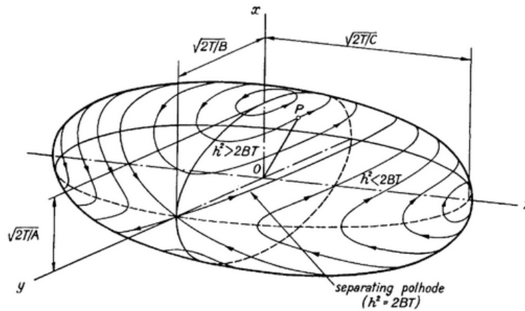
Fig. 6.3. Poinsot's ellipsoid, showing polhodes for different initial conditions of motions ( A > B > C ).
