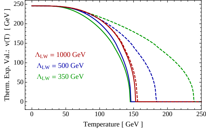
Figure 2. The electroweak symmetry-breaking order parameter v(T) for the case of \sigma = +1 (dashed) and \sigma = -1 (solid). The phase transition temperature is generally higher in the former case due to the cancellation of the leading O(T^2) temperature dependence discussed in the text.
