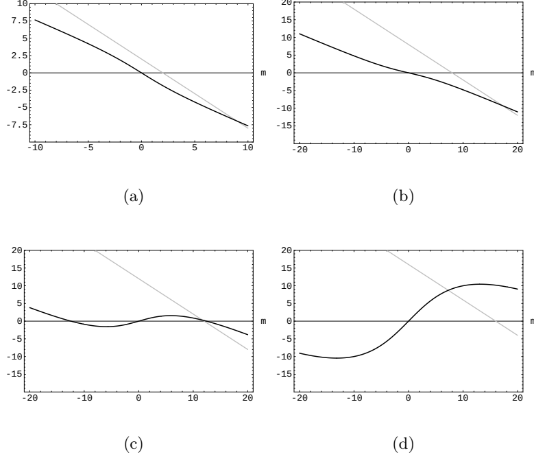
Figure 3.6: Plots of the left-hand side (in gray) and right-hand side (in black) of equation Eq. (3.25). For all of them \alpha \equiv \frac{g}{2\pi^2} = 0.01 . (a) \Lambda = m_0 = 2 . (b) \Lambda = m_0 = 8 . (c) \Lambda = m_0 = 12 . (d) \Lambda = m_0 = 16 .
