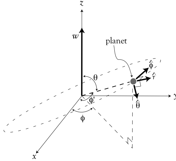
Figure 4.1: Diagram of a planet moving in a circular orbit of radius r around the sun (located at the origin), whose velocity with respect to the preferred frame is \mathbf{w} . The inclination between the plane of the orbit and the axis of \mathbf{w} is \theta_0 (the minimum value of the polar angle \theta during the planet's orbit).
