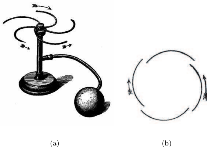
Figure 6.8: Illustrations from Ernst Mach’s Mechanik ([137]): (a) Figure 153 a in the original. (b) Figure 154 in the original. (Images in the public domain, copied from the English edition of 1893.)
