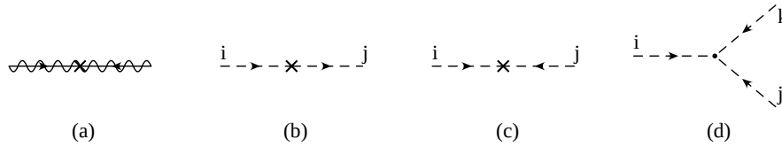
Figure 6: Soft supersymmetry-breaking terms: (a) Gaugino mass insertion M_\lambda ; (b) non-analytic scalar (\text{mass})^2 (m^2)_j^i ; (c) analytic scalar (\text{mass})^2 b^{ij} ; (d) (\text{scalar})^3 coupling a^{ijk} .
