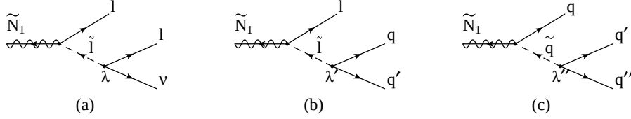
Figure 20: Decays of the \tilde{N}_1 LSP in models with R -parity violation [see eqs. (5.7) and (5.8)].
