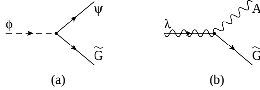
Figure 15: Goldstino/gravitino interactions with superpartner pairs (\phi, \psi) and (\lambda^a, A^a) .
