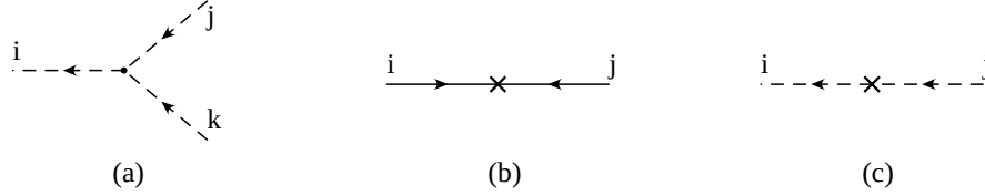
Figure 4: Supersymmetric dimensionful couplings: (a) (scalar) 3 interaction vertex M_{in}^*y^{jkn} , (b) fermion mass term M^{ij} , (c) scalar (mass) 2 term M_{ik}^*M^{kj} .
