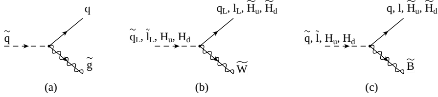
Figure 9: Couplings of the gluino, wino, and bino to MSSM (scalar, fermion) pairs.
