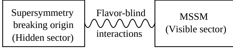
Figure 14: The presumed schematic structure for supersymmetry breaking.
