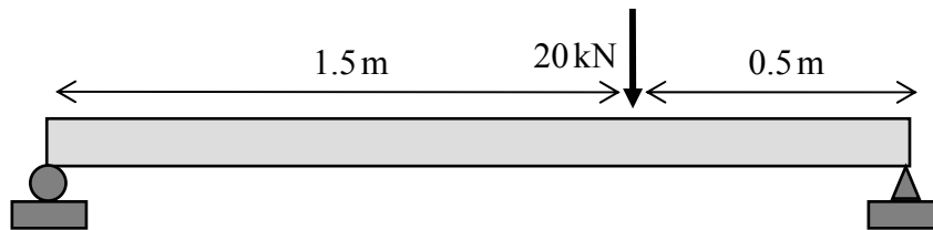
Figure 4.6.26: a simply supported beam
