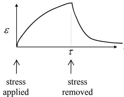
Figure 7.3.7: Creep-Recovery Response of the Kelvin (Voigt) Model
