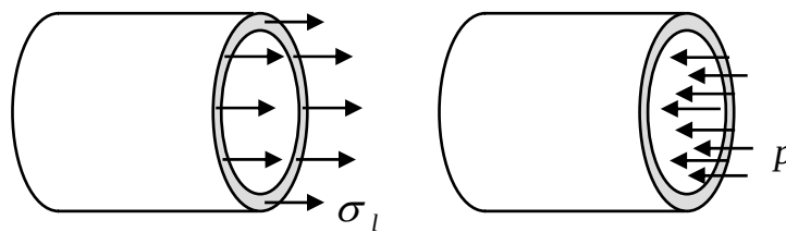
Figure 4.5.9: free body diagram of a cylindrical pressure vessel
