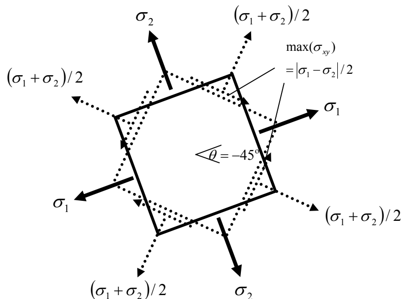
Figure 3.5.17: principal stresses and maximum shear stress
