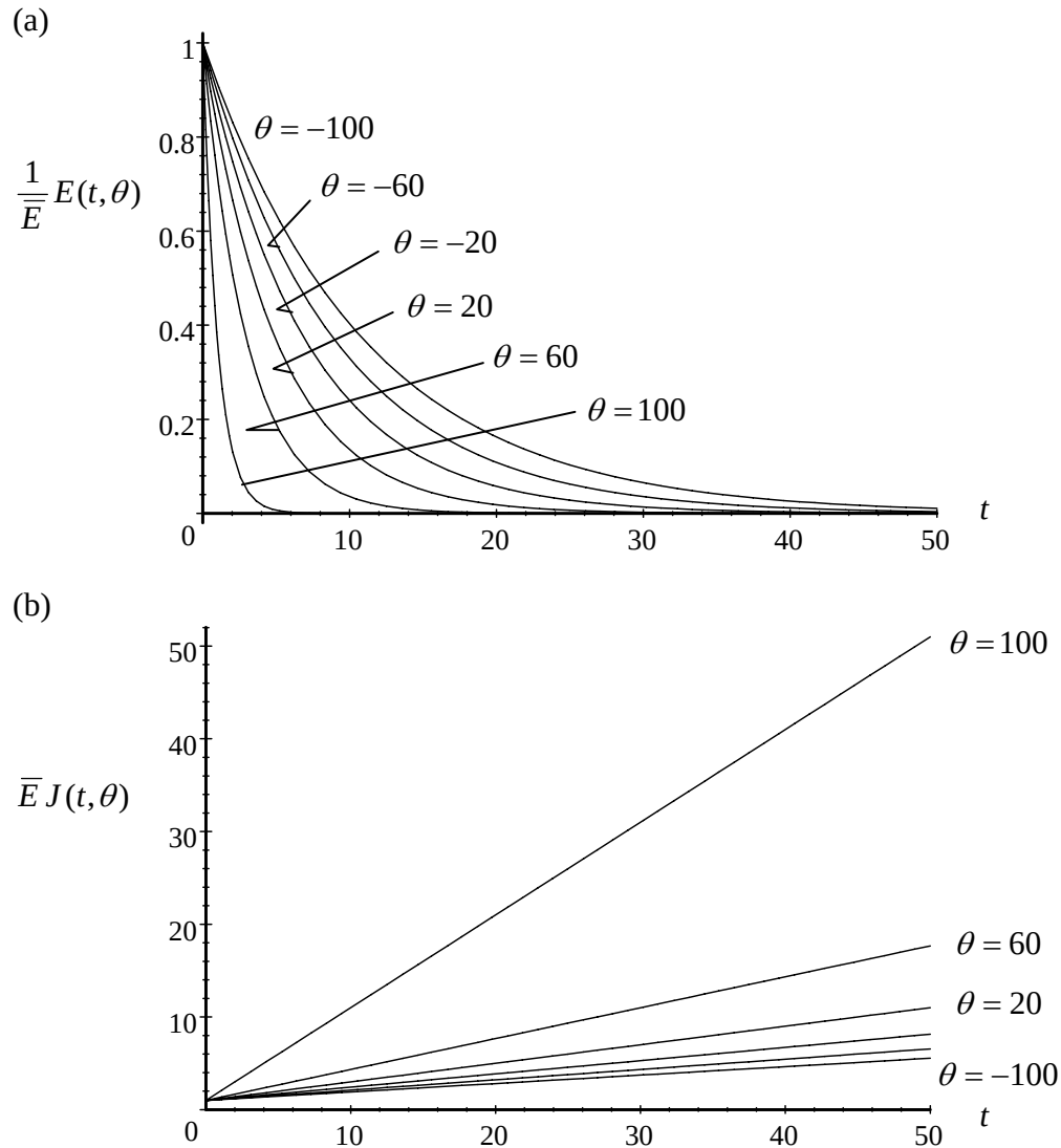
Figure 7.7.2: temperature-dependent functions; (a) relaxation modulus, (b) creep compliance
