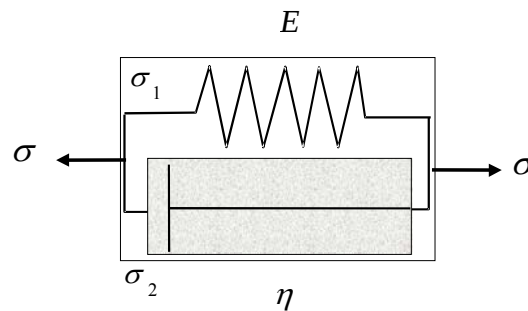
Figure 7.3.6: the Kelvin (Voigt) Model
