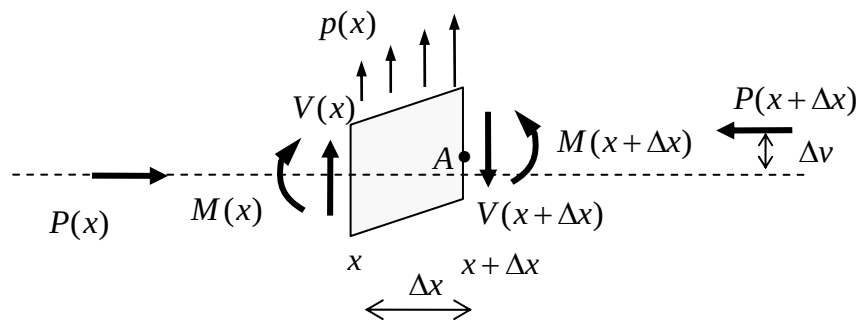
Figure 6.1.3: forces and moments acting on a column
