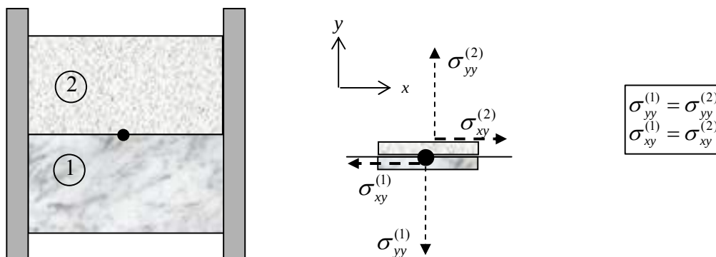
Figure 3.5.3: normal and shear stress continuous across an interface between two different materials, material '1' and material '2'
