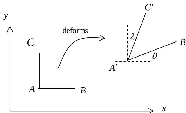
Figure 3.6.2: strain at a point A
