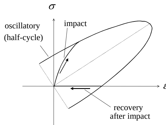
Figure 7.6.4: Impact approximated as a half-cycle of oscillatory stress and strain
