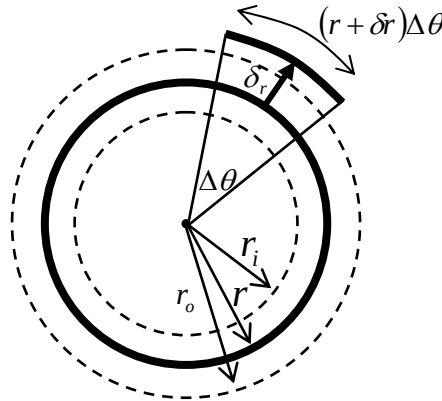
Figure 4.5.7: Deformation in the thin-walled sphere as it expands
