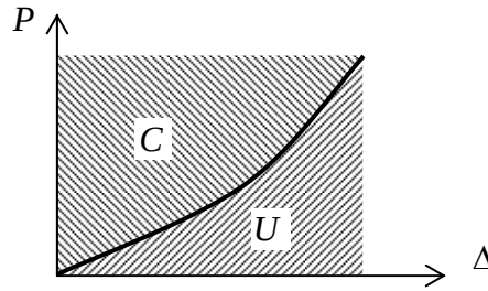
Figure 5.3.2: strain energy and complementary energy for an elastic material
