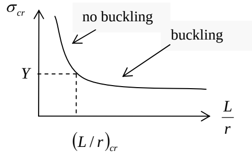
Fig. 6.1.2: critical values of the slenderness ratio
