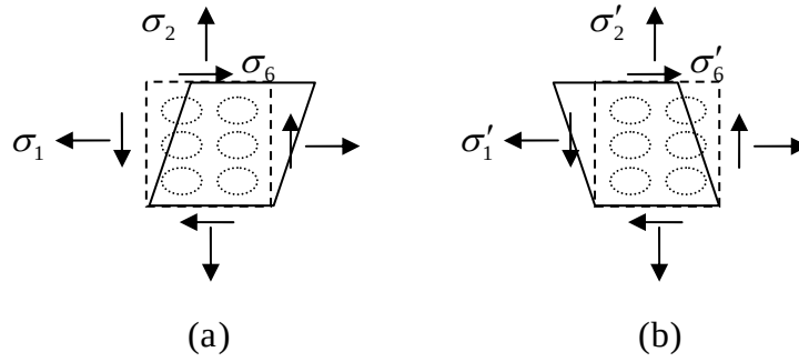
Figure 6.2.4: an element of orthotropic material undergoing shear strain; (a) positive strain, (b) negative strain
