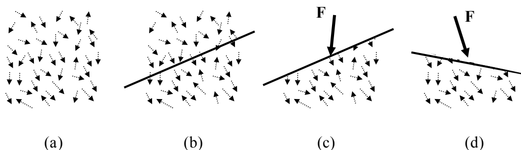
Figure 3.3.4: a multitude of molecular forces represented by a single force
