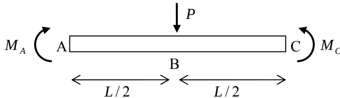
Figure 5.2.12: a statically indeterminate beam
