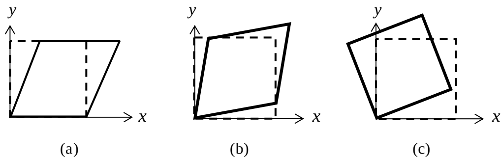
Figure 3.6.9: (a) simple shear, (b) pure shear, (c) pure rotation
