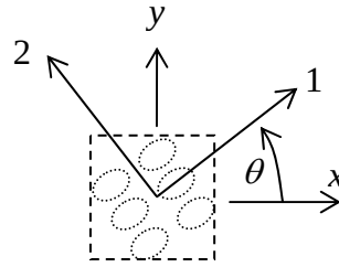
Figure 6.2.5: reference axes not aligned with the material directions
