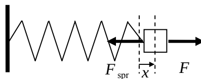
Figure 5.1.2: a force extending an elastic spring
