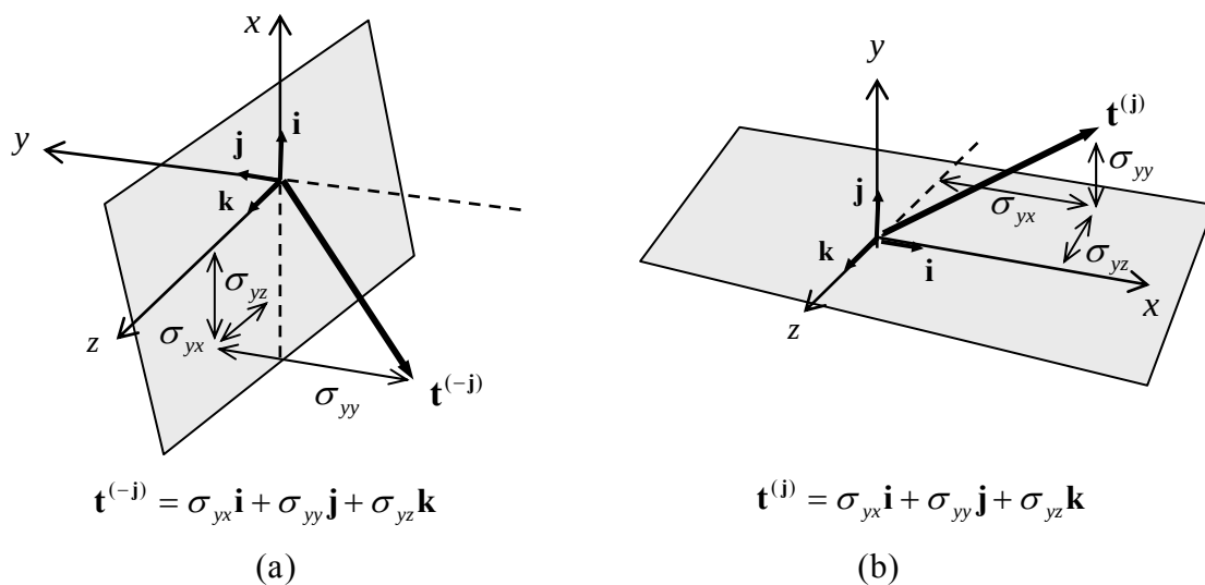
Figure 3.3.10: examples of negative stress components
