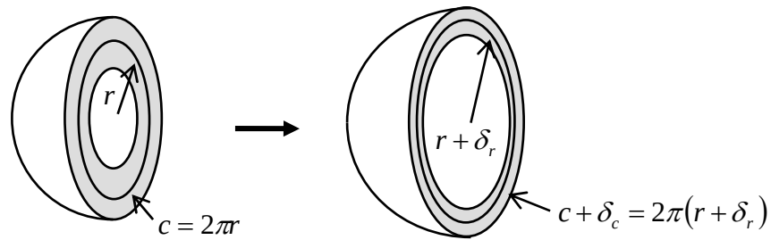
Figure 4.5.8: Increase in circumference length as the vessel expands
