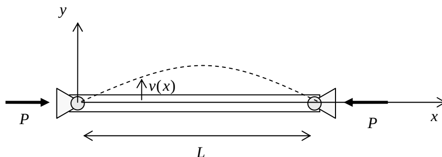
Fig. 6.1.1: a column with deflection v
