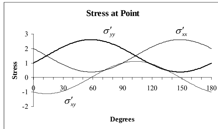
Figure 3.5.14: stresses on different planes through a point
