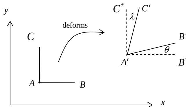
Figure 3.6.5: small deformation
