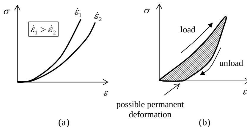
Figure 7.1.1: Response of a Viscoelastic material in the Tension test; (a) different rates of stretching, (b) loading and unloading with possible permanent deformation (non-zero strain at zero stress)
