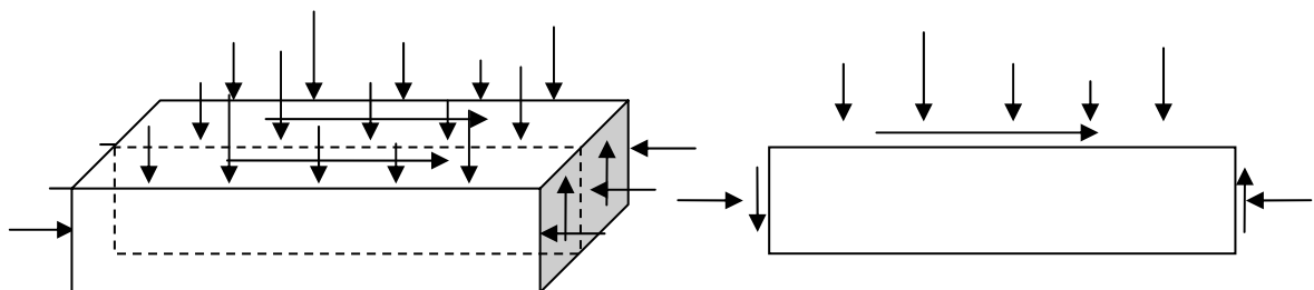
Figure 3.7.4: three dimensional problem reduces to a two dimensional one for the case of plane strain
