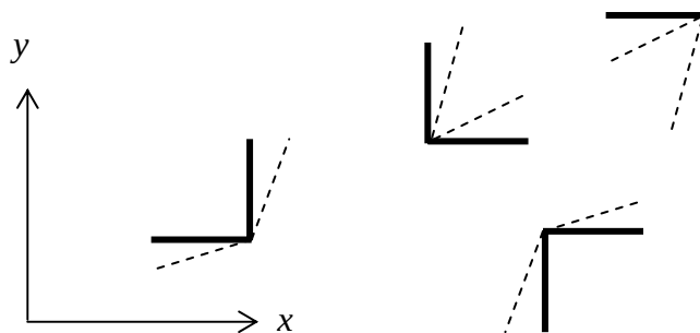
Figure 3.6.6: positive shear strain
