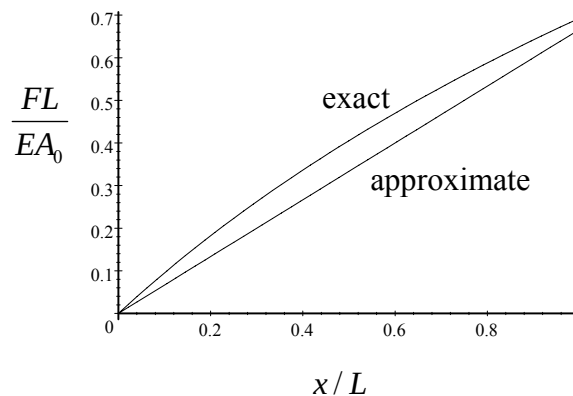
Figure 5.6.3: exact and (Ritz) approximate solution for axial problem
