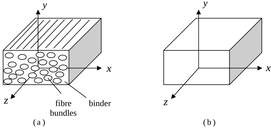
Figure 6.2.2: an orthotropic material; (a) microstructural detail, (b) continuum model
