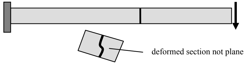
Figure 4.6.28: a cantilevered beam loaded by a force and moment
