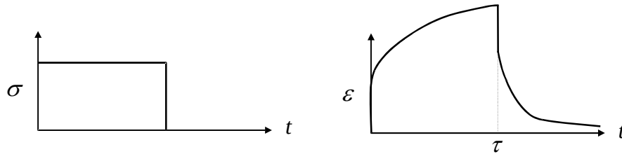
Figure 7.5.2: Creep-recovery response of the standard linear model
