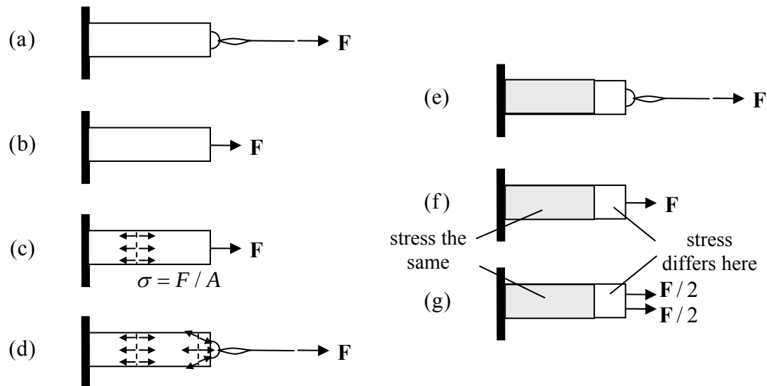
Figure 3.3.11: a block subjected to an external force: (a) real case, (b) ideal model, (c) stress in ideal model, (d) stress in actual material, (e) stress in real material modelled well by either (f) or (g)
