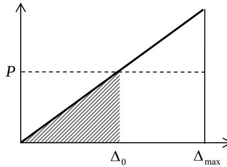
Figure 5.2.14: non-equilibrium loading
