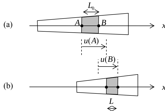
Figure 4.3.2: axial strain; (a) before deformation, (b) after deformation
