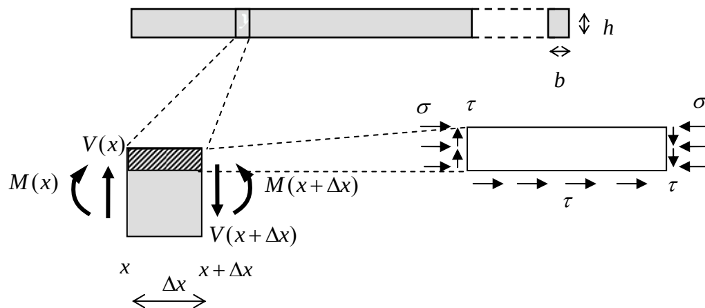
Figure 4.6.25: stresses and forces acting on a small section of material at the surface of a beam
