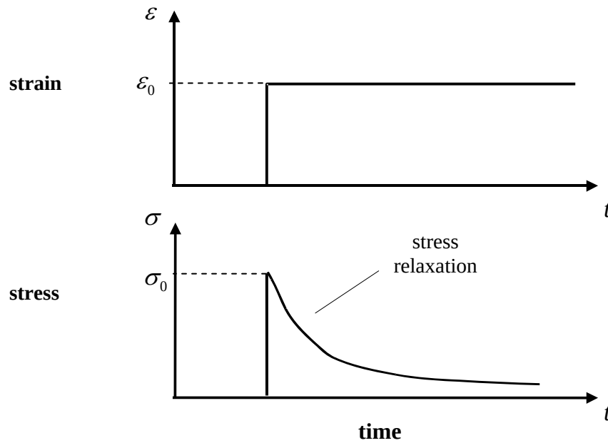
Figure 7.1.4: Stress response to the stress-relaxation test
