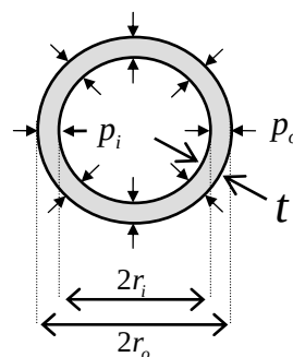
Figure 4.5.11: A pressure vessel subjected to internal and external pressure
