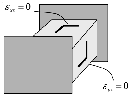
Figure 3.7.3: Line elements etched in a block of material – they remain perpendicular in a state of plane strain
