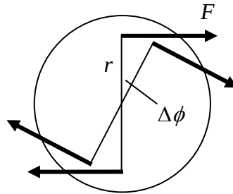
Figure 5.2.3: torque acting on a circular bar
