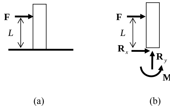
Figure 2.3.9: A loaded cantilevered component; (a) loaded component, (b) free body diagram of the component
