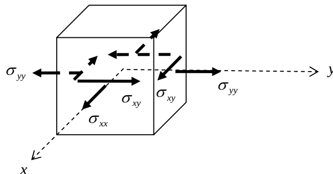
Figure 3.5.10: non-zero stress components acting in the x - y plane
