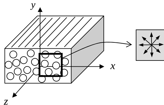
Figure 6.2.6: a transversely isotropic material
