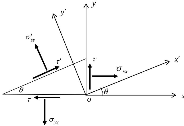
Figure 3.4.7: a free body diagram of a triangular element of material
