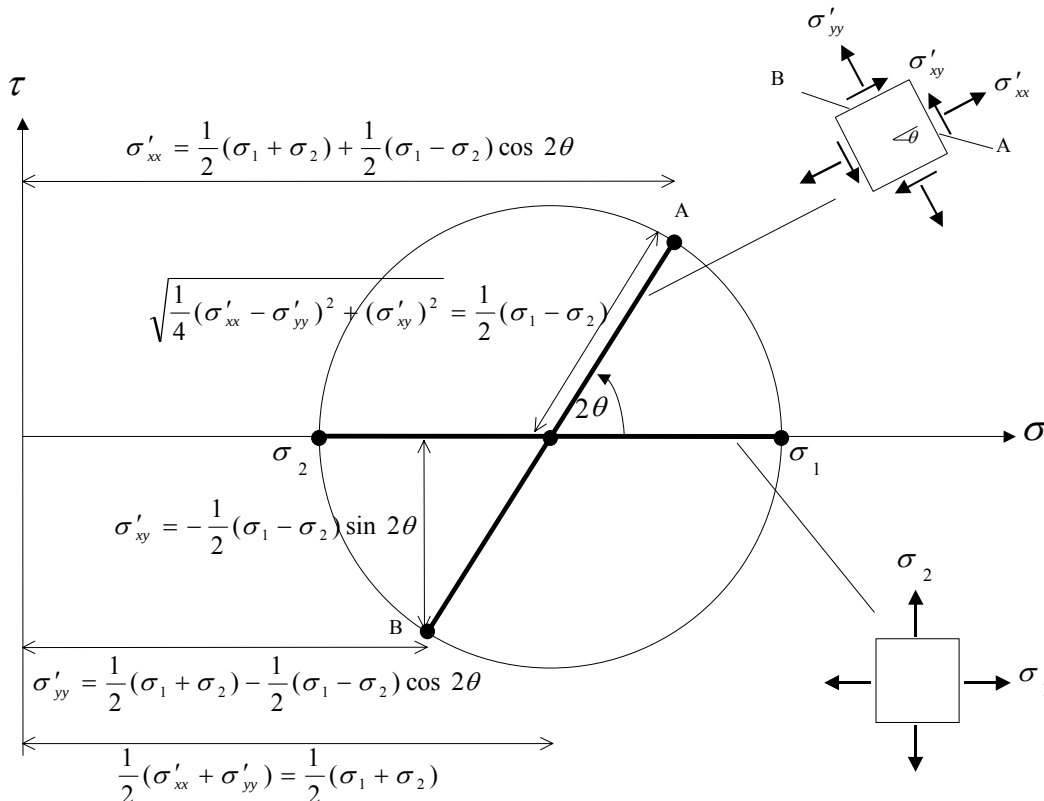
Figure 3.5.18: Mohr's Circle
