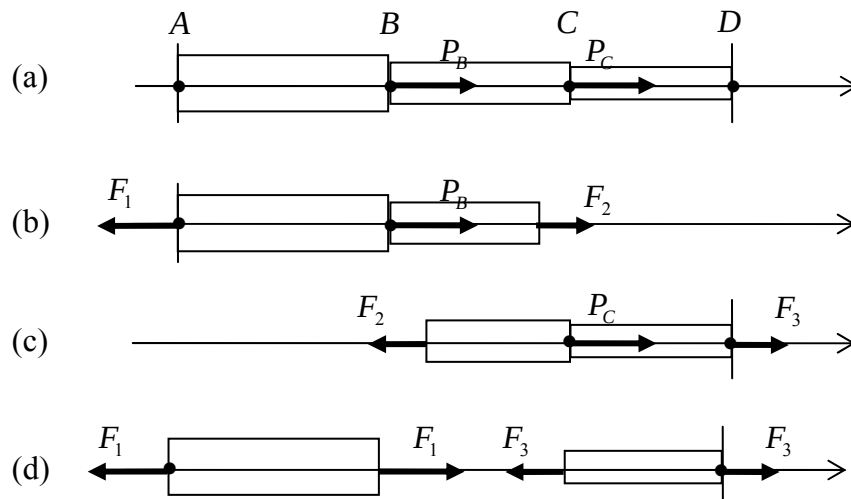
Figure 4.3.7: three bars in series; (a) subjected to external loads, (b,c,d) free-body diagrams
