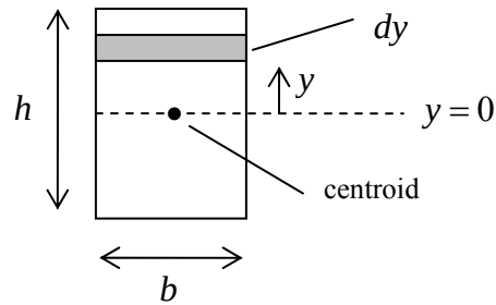
Figure 4.6.22: Evaluation of the moment of inertia for a rectangular cross-section
