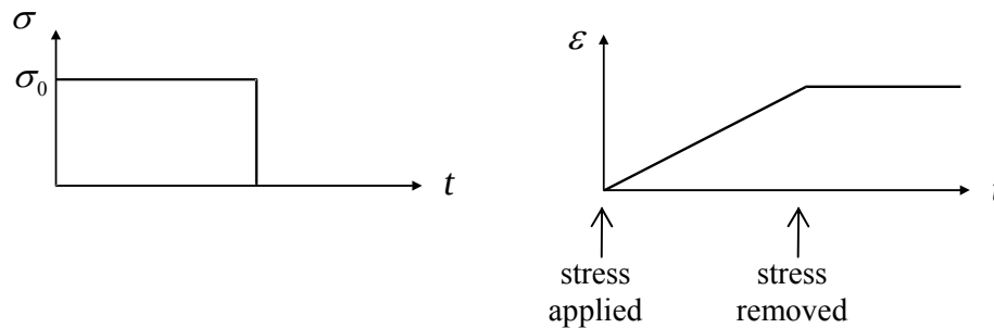
Figure 7.3.3: Creep-Recovery Response of the Dash-pot
