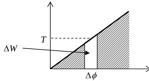
Figure 5.2.4: torque – angle of twist plot for torsion
