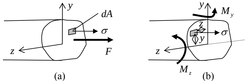
Figure 4.3.9: Resultants on a cross-section; (a) resultant force, (b) resultant moments
