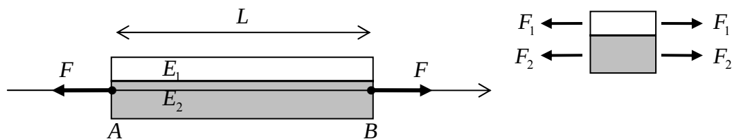
Figure 4.3.8: A bar consisting of two separate materials bonded together
