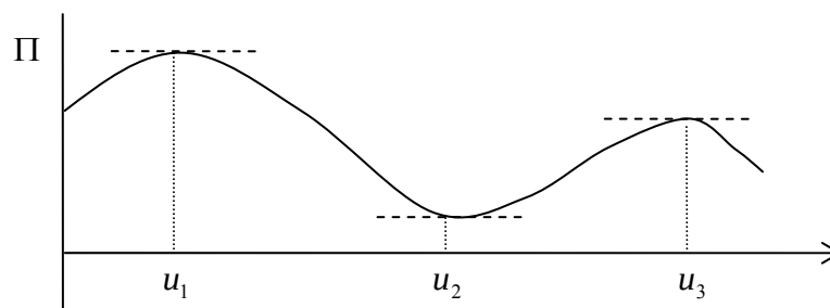
Figure 5.6.2: the total potential energy of a system
