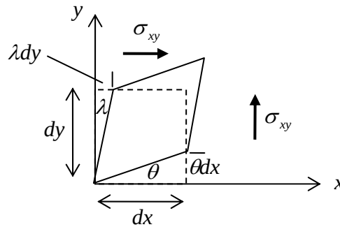
Figure 5.2.10: a volume element under shear stress
