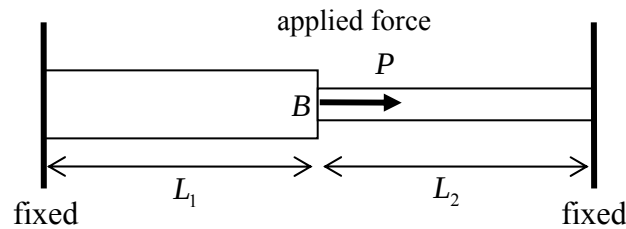
Figure 5.5.5: two rods subjected to a force P
