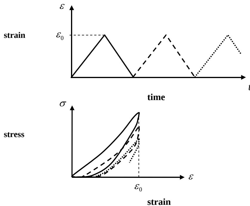
Figure 7.1.5: Typical stress response to the cyclic test
