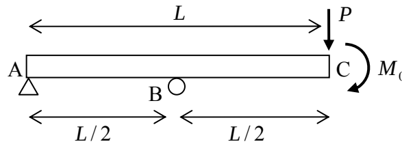
Figure 5.2.11: a beam subjected to a force and moment at C
