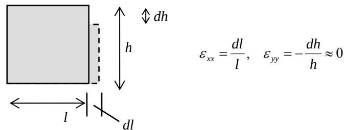
Figure 4.6.20: transverse strain is neglected in the elementary beam theory
