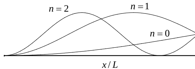
Figure 6.1.5: mode shapes for the fixed-free column
