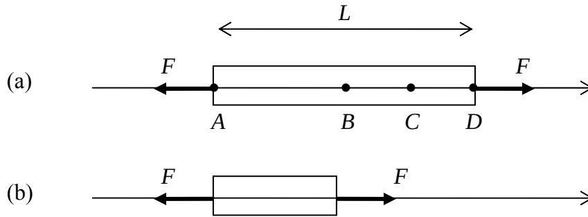
Figure 4.3.4: A uniform axial member; (a) subjected to axial forces F , (b) free-body diagram
