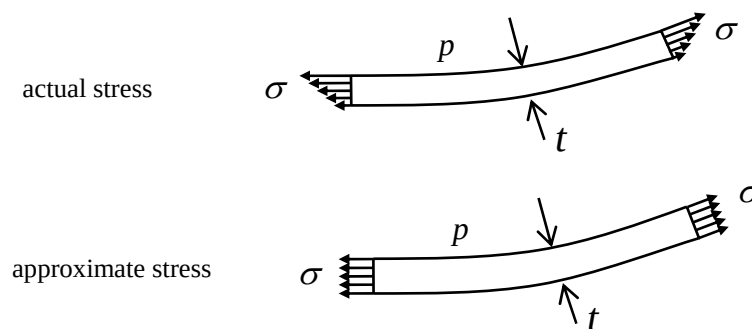
Figure 4.5.2: Approximation to the stress arising in a pressure vessel
