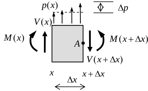
Figure 4.6.18: forces and moments acting on a small element of beam
