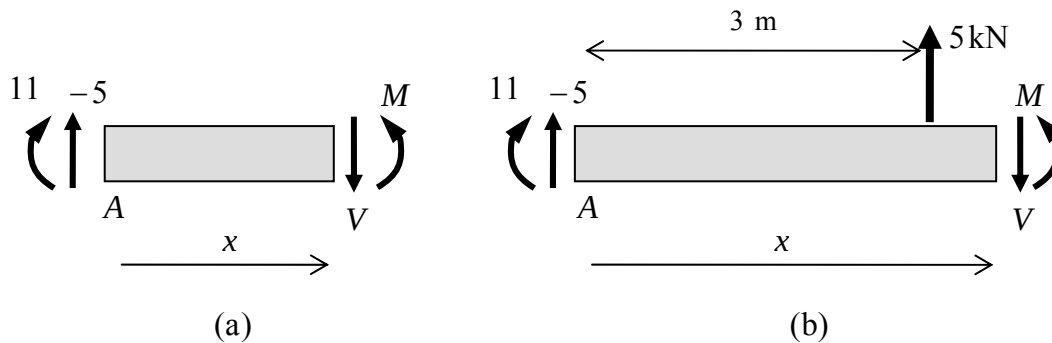
Figure 4.6.11: free body diagrams of sections of a beam
