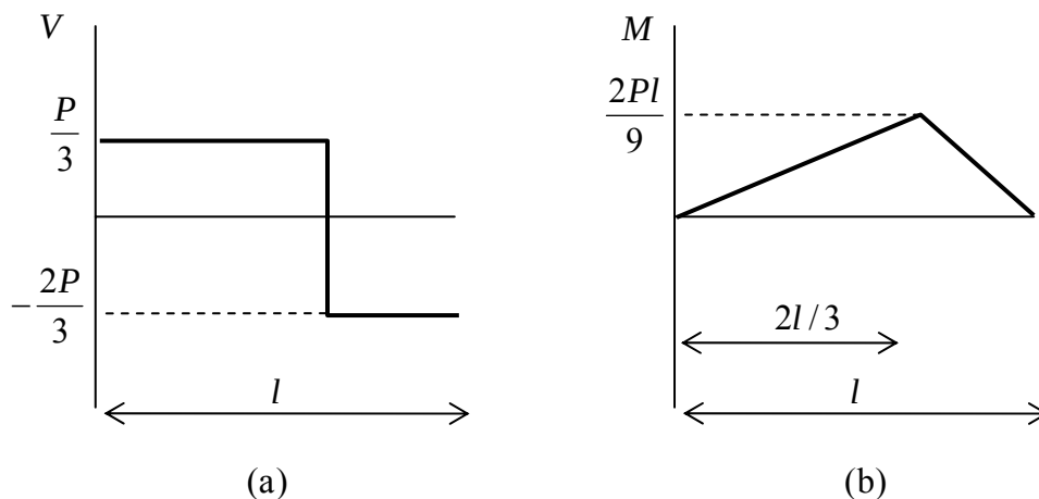
Figure 4.6.9: results of analysis; (a) shear force diagram, (b) bending moment diagram
