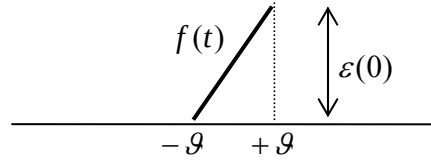
Figure 7.4.2: A function used to approximate the strain for a sudden jump
