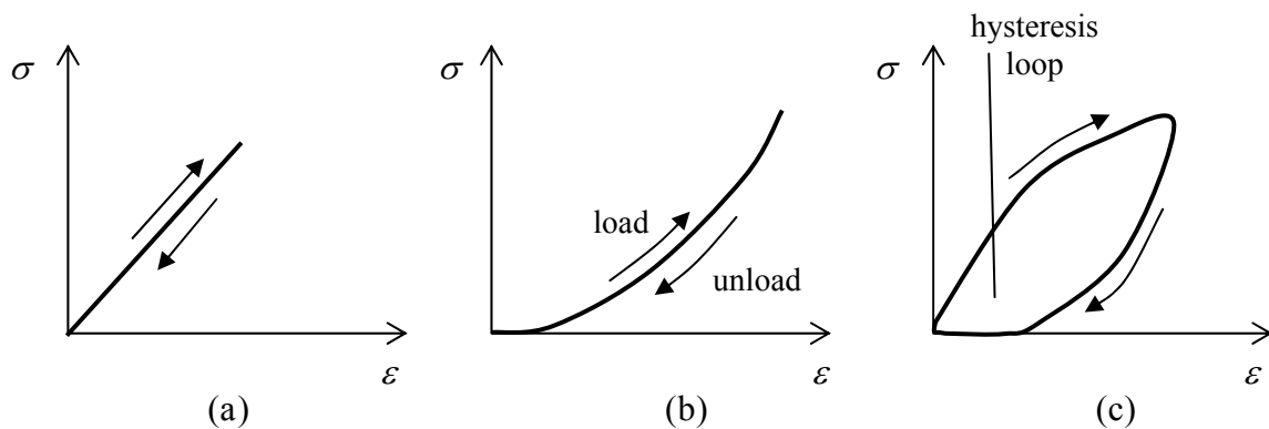
Figure 4.2.3: Different stress-strain relationships; (a) linear elastic, (b) non-linear elastic, (c) viscoelastic/plastic/viscoplastic
