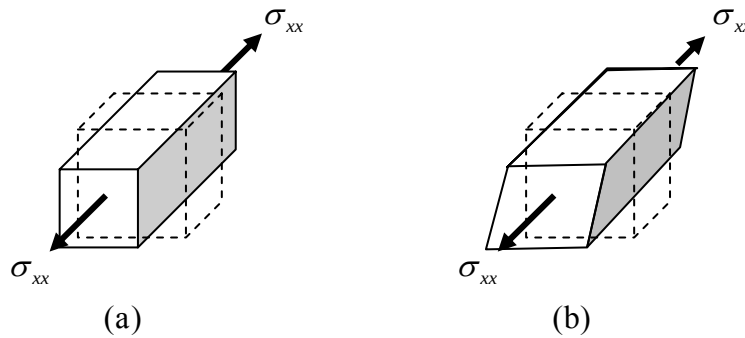
Figure 4.2.5: an element of material subjected to a uniaxial stress; (a) normal strain, (b) shear strain
