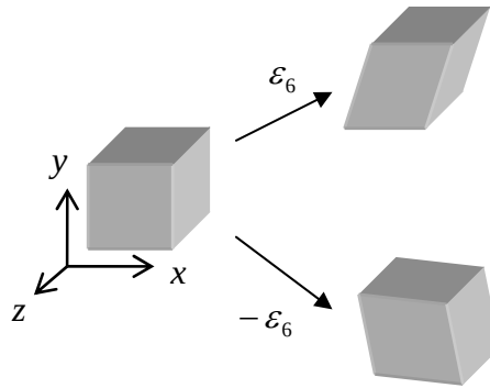
Figure 6.2.3: an element of orthotropic material undergoing shear strain
