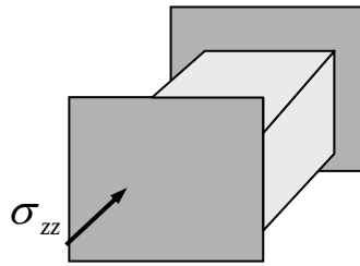
Figure 4.2.10 Plane strain - a thick component constrained in one direction
