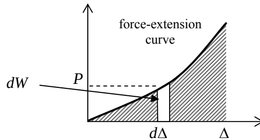
Figure 5.3.1: force-displacement curve for a non-linear material
