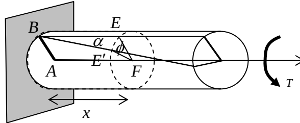
Figure 4.4.2: A section of a twisting cylindrical member
