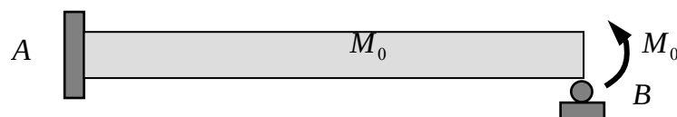
Figure 4.6.35: a statically indeterminate beam
