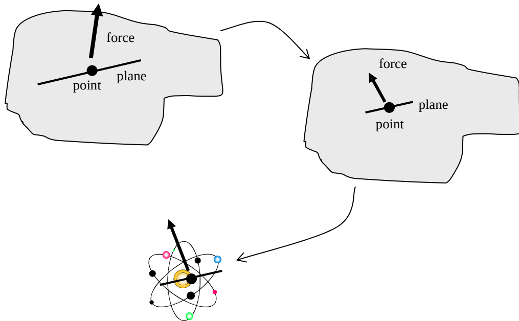
Figure 4.1.1: A force acting on an internal surface
