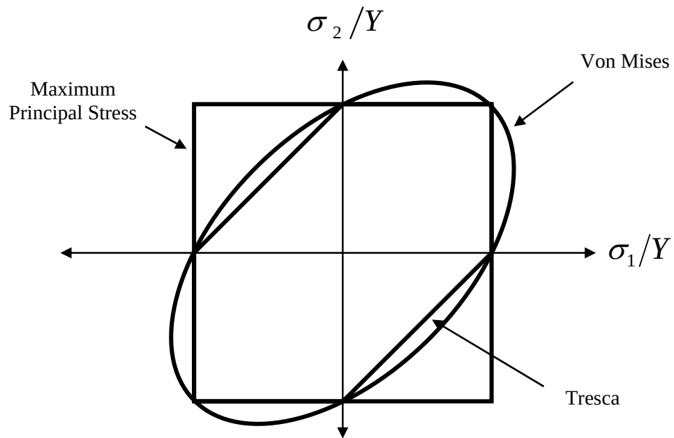
Figure 4.7.1: Failure theories in stress space
