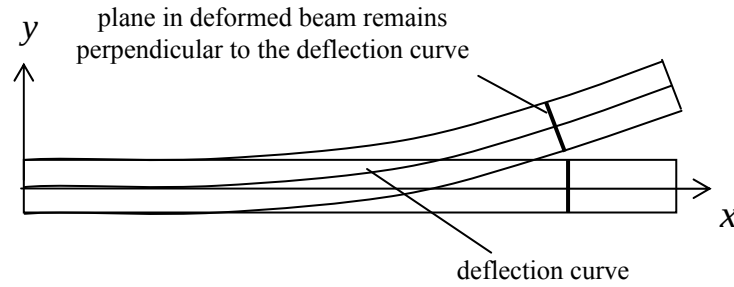
Figure 4.6.19: plane sections remain plane in the elementary beam theory
