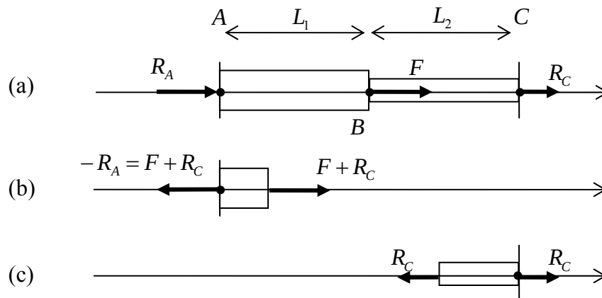
Figure 4.3.6: A two-element structure built-in and both ends; (a) subjected to an axial force F , (b,c) free-body diagrams
