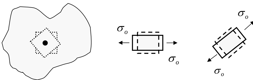
Figure 4.2.4: Illustration of Isotropy
