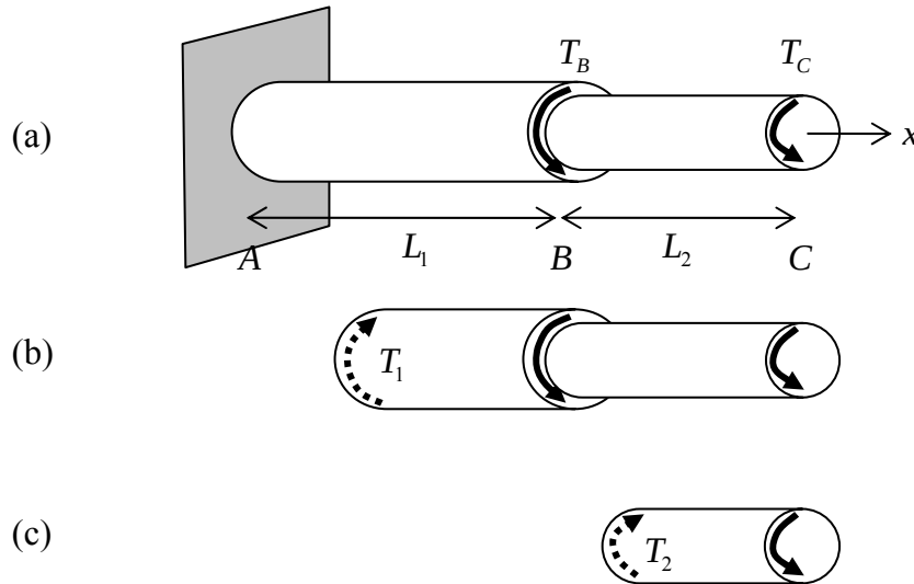
Figure 4.4.4: A structure consisting of two torsion members; (a) subjected to torques T_B and T_C , (b,c) free-body diagrams
