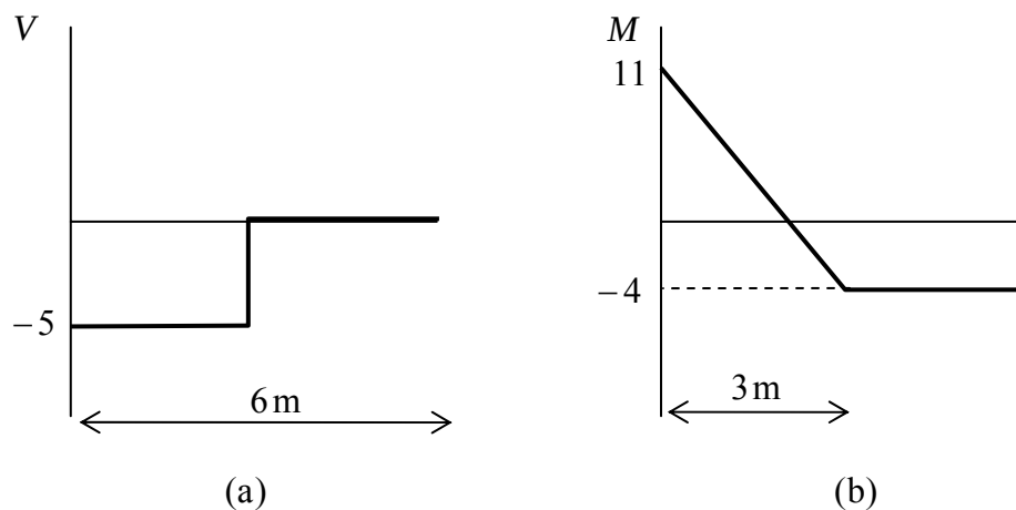
Figure 4.6.12: results of analysis; (a) shear force diagram, (b) bending moment diagram
