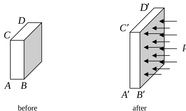
Figure 4.5.6: Strain of an element at the surface of a spherical pressure vessel
