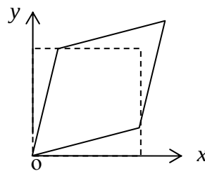
Figure 3.8.3: A block under pure shear
