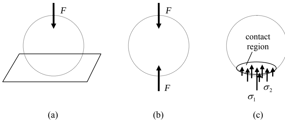
Figure 3.1.2: a ball being forced into a large object, (a) force applied to ball, (b) reaction of object on ball, (c) a non-uniform stress distribution over the contacting surface
