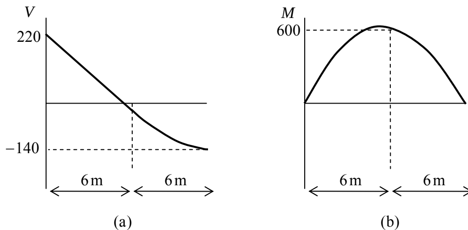
Figure 4.6.17: results of analysis; (a) shear force diagram, (b) bending moment diagram
