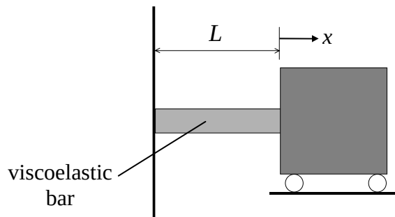
Figure 7.6.5: Vibration
