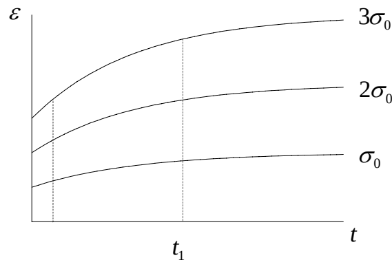
Figure 7.1.2: Strain as a function of time at different loads
