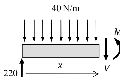
Figure 4.6.15: free body diagram of a section of a beam
