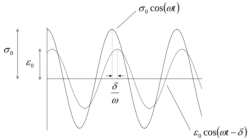
Figure 7.6.1: Oscillatory stress and strain
