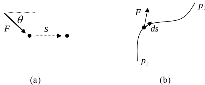
Figure 5.1.1: (a) force acting on a particle, which moves through a displacement s ; (b) a varying force moving a particle along a path
