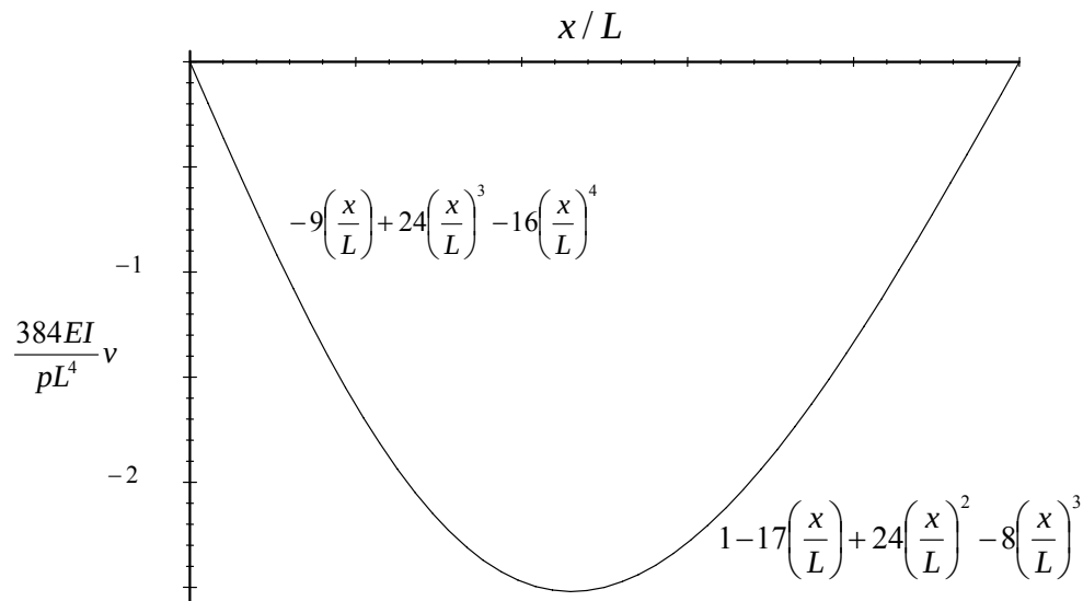
Figure 4.6.32: deflection of a beam ■
