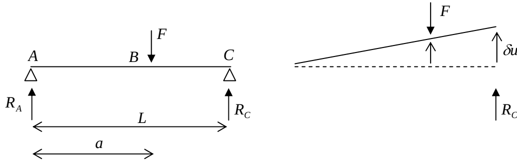
Figure 5.5.3: a loaded rigid bar; (a) bar geometry, (b) a virtual displacement at end C
