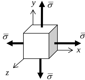
Figure 4.2.7: A block of linear elastic material subjected to an equi-biaxial stress
