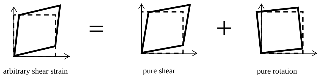
Figure 3.6.10: shear strain decomposed into a pure shear and a pure rotation
