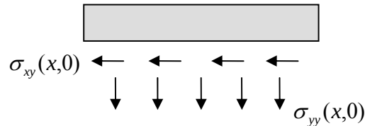
Figure 3.5.8: unknown reaction stresses acting on the lower edge
