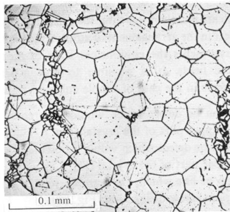
Figure 4.1.3: metal grains
