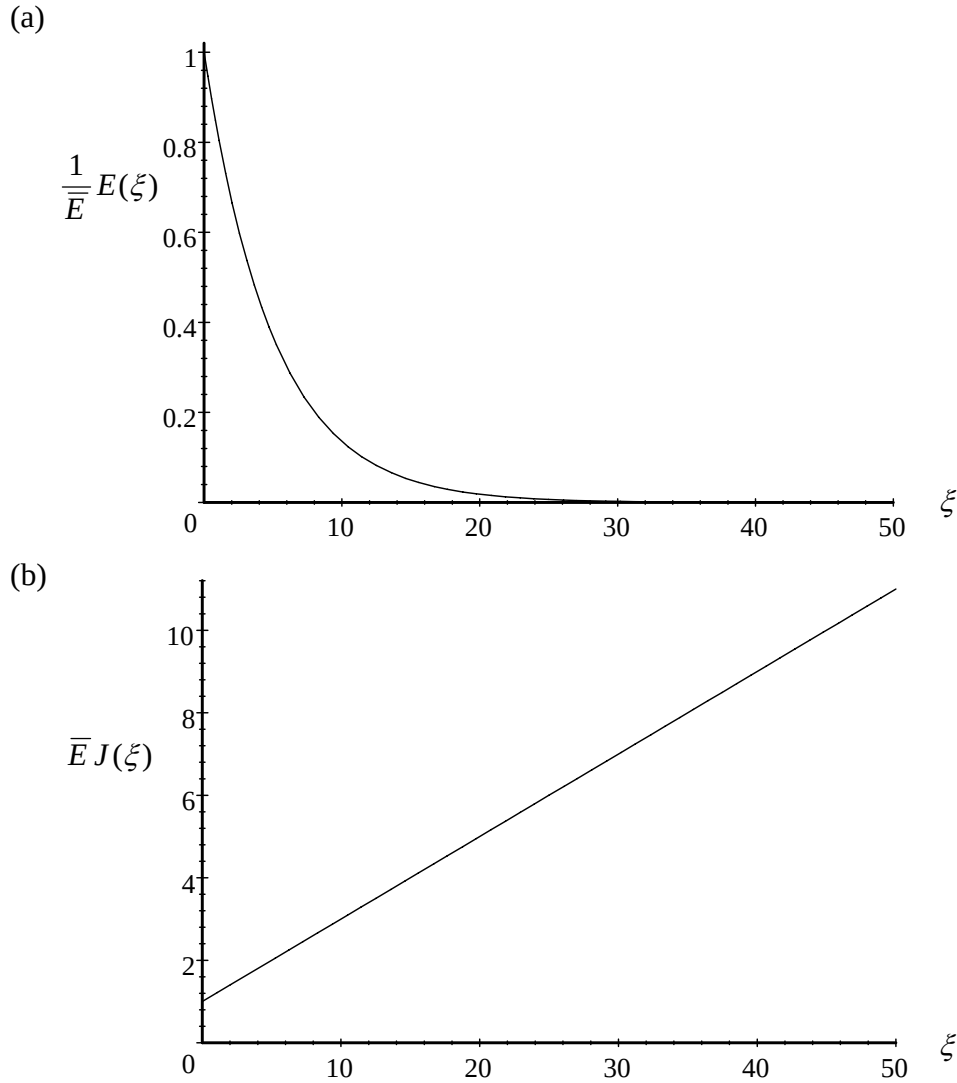
Figure 7.7.3: master curves; (a) relaxation modulus, (b) creep compliance
