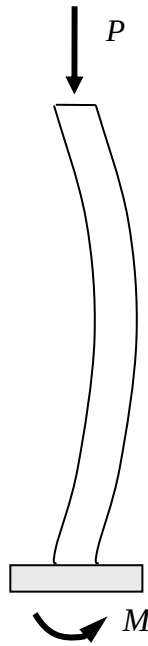
Fig. 6.1.4: a fixed-free column
