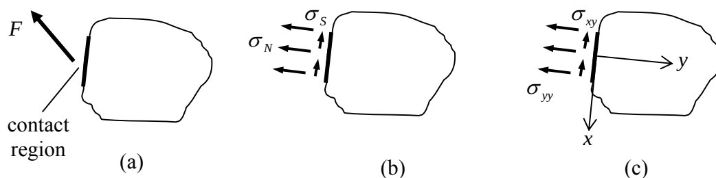
Figure 3.5.1: Stress boundary conditions; (a) force acting on material due to contact with a second material, (b) the resulting normal and shear stress distributions, (c) applied stresses as stress components in a given coordinate system
