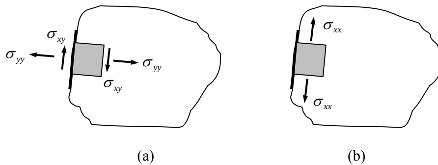
Figure 3.5.2: Stresses acting on a material element at the boundary, (a) normal and shear stresses, (b) tangential stresses
