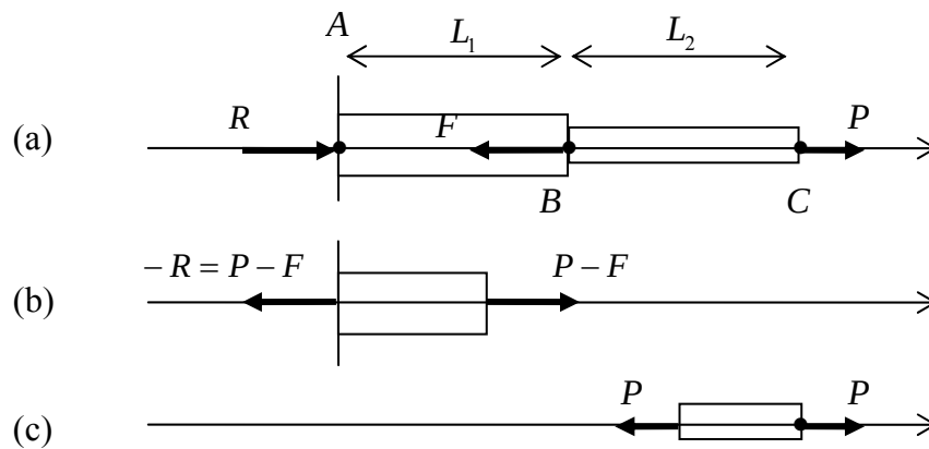
Figure 4.3.5: A two-element structure (a) subjected to axial forces F and P , (b,c) free-body diagrams
