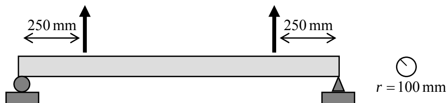
Figure 4.6.23: a loaded beam with circular cross-section
