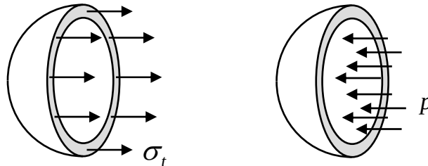
Figure 4.5.4: a free body diagram of one half of the spherical pressure vessel
