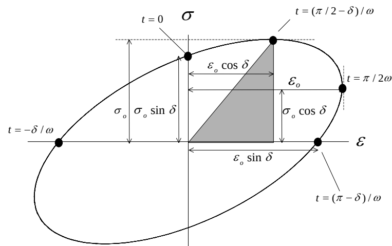
Figure 7.6.3: Elliptic Stress-Strain Hysteresis Loop
