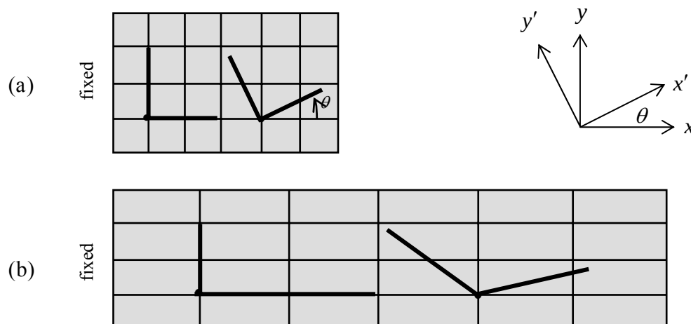
Figure 3.8.2: A block with strain measured in two different coordinate systems
