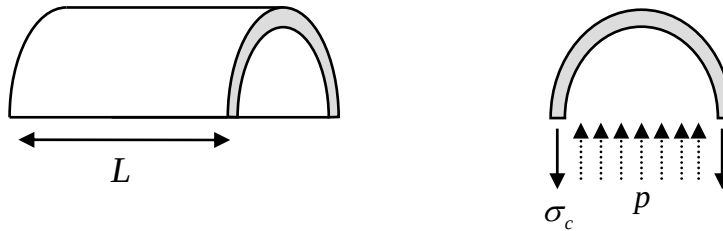
Figure 4.5.10: free body diagram of a cylindrical pressure vessel
