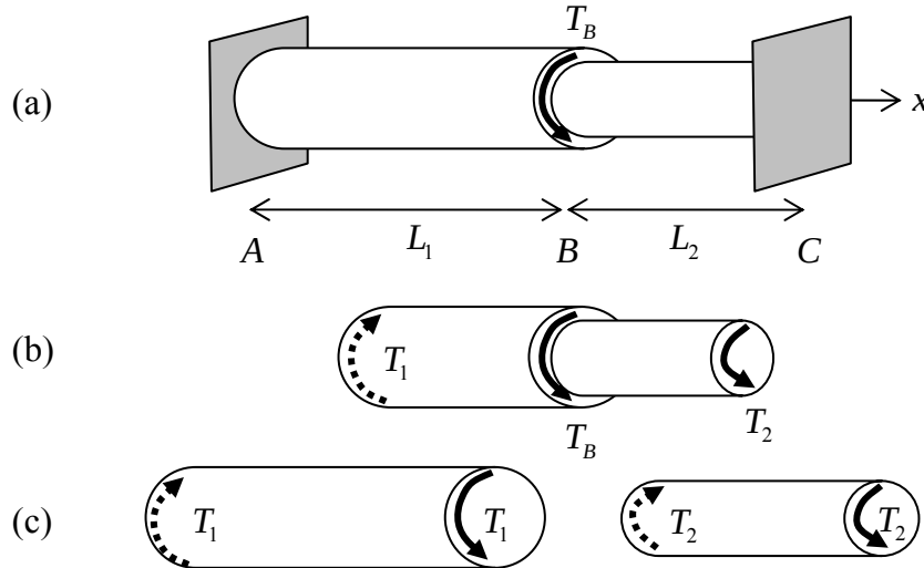
Figure 4.4.5: A structure consisting of two torsion members; (a) subjected to a Torque T_B , (b) free-body diagram, (c) separate elements
