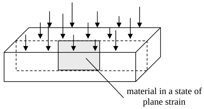
Figure 3.7.5: material in an approximate state of plane strain
