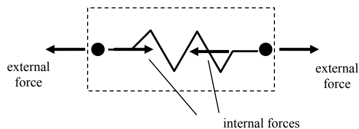
Figure 5.1.6: external force pulling two molecules/particles apart
