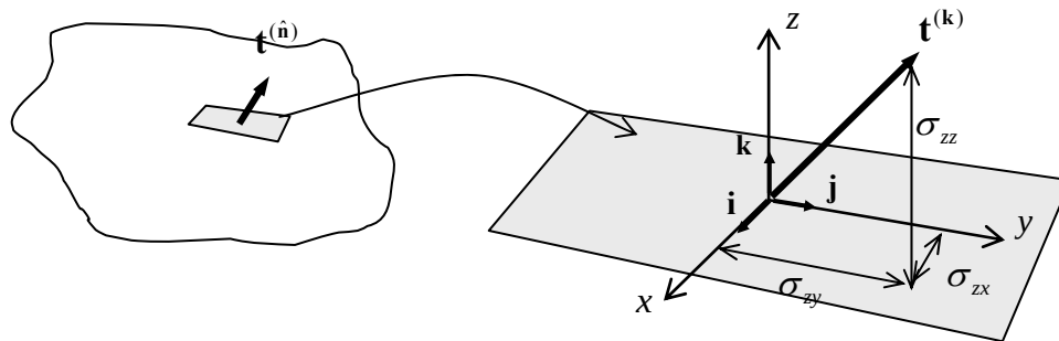
Figure 3.3.7: stress components – the components of the traction vector
