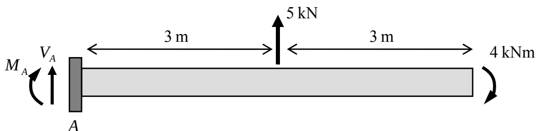
Figure 4.6.10: a cantilevered beam loaded by a force and moment
