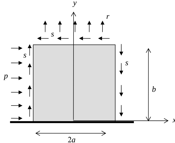
Figure 3.5.7: a plate subjected to stress distributions
