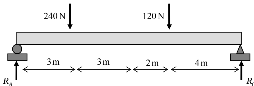
Figure 4.6.14: equivalent forces acting on the beam of Fig. 4.6.13
