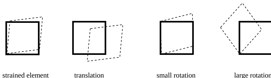
Figure 3.6.11: an element under shear strain; (a) the strained element, (b) the element with an additional translation, (c) with a small rotation, (d) with a large rotation
