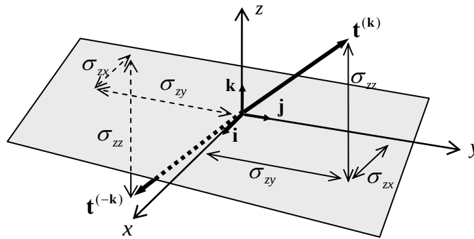
Figure 3.3.8: equal and opposite traction vectors – each with the same stress components
