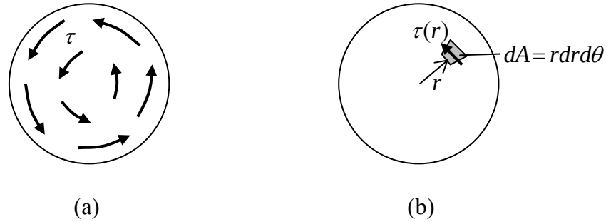
Figure 4.4.3: Shear stresses acting over a cross-section; (a) shear stress, (b) moment for an elemental area
