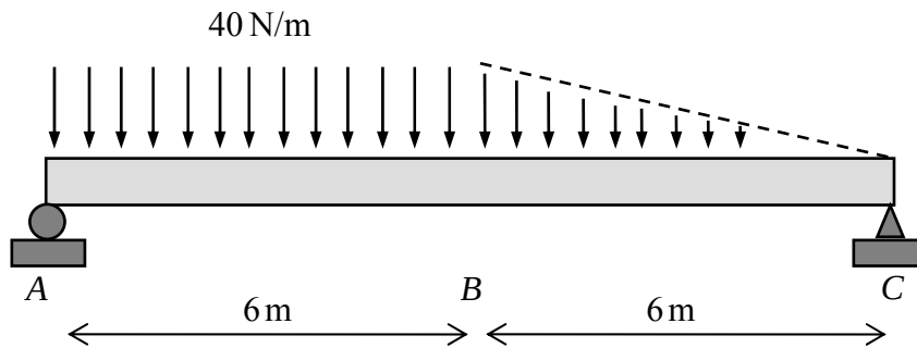
Figure 4.6.13: a beam subjected to a distributed load
