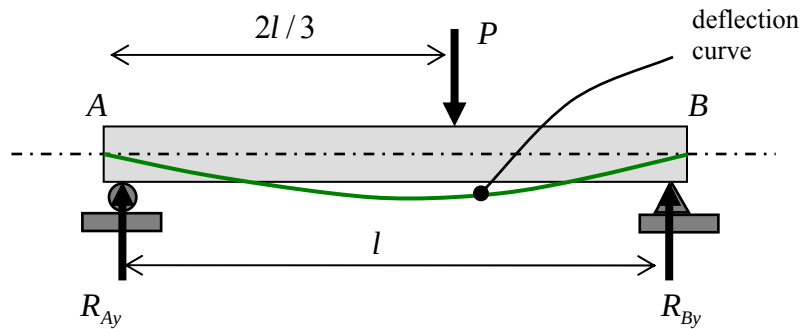
Figure 4.6.7: a simply supported beam
