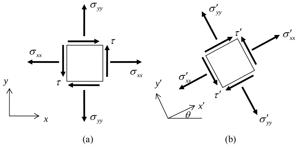
Figure 3.4.5: stress components acting on two different sets of perpendicular surfaces, i.e. in two different coordinate systems; (a) original system, (b) rotated system
