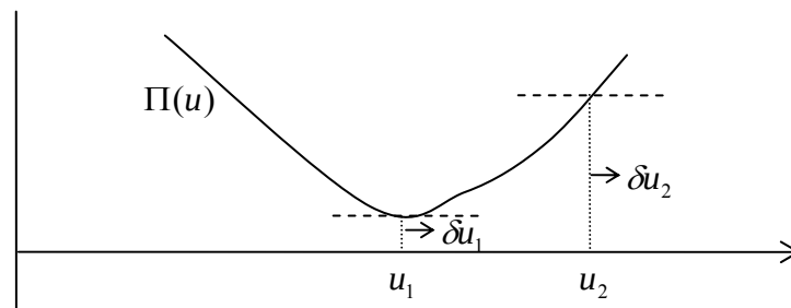
Figure 5.6.1: the total potential energy of a system
