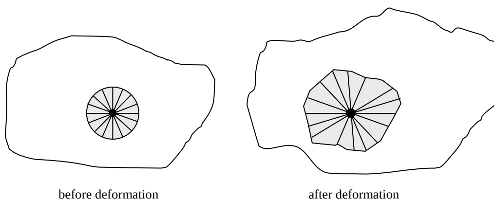
Figure 3.6.1: a deforming material element; original state of line elements and their final position after straining
