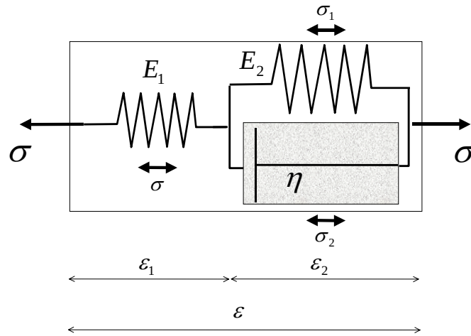
Figure 7.5.1: the standard linear model
