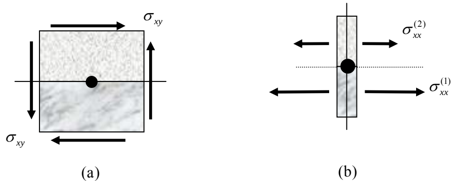
Figure 3.5.4: stresses at an interface; (a) shear stresses continuous across the interface, (b) tangential stresses not necessarily continuous
