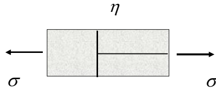
Figure 7.3.2: the linear dash-pot
