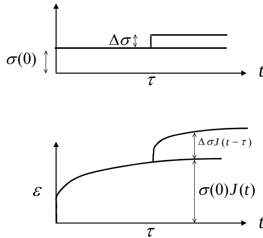
Figure 7.4.3: Superposition of loads
