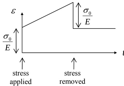
Figure 7.3.5: Creep-Recovery Response of the Maxwell Model
