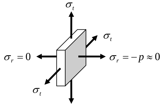
Figure 4.5.5: An element at the surface of a spherical pressure vessel
