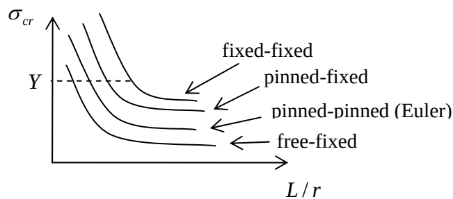
Fig. 6.1.6: critical values of the slenderness ratio for different end-cases
