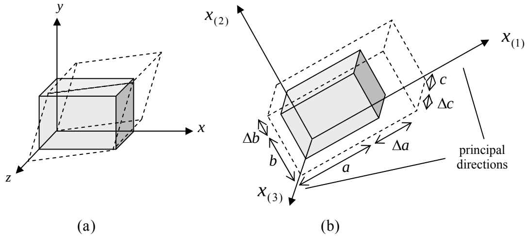
Figure 4.2.8: A block of material subjected to a general strain
