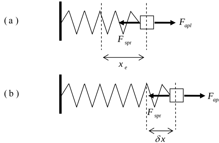
Figure 5.5.1: a force extending an elastic spring; (a) block in equilibrium, (b) block not at its equilibrium position
