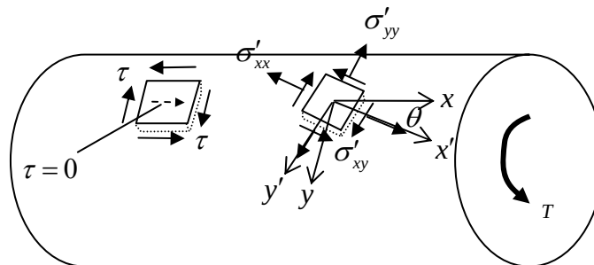
Figure 4.4.6: Stress distribution in a torsion member
