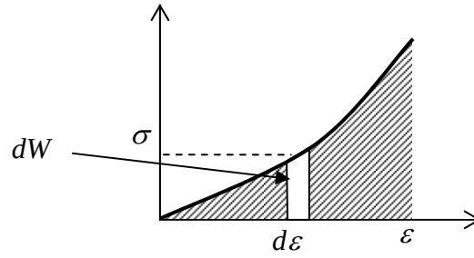
Figure 5.4.2: stress-strain curve for a non-linear material
