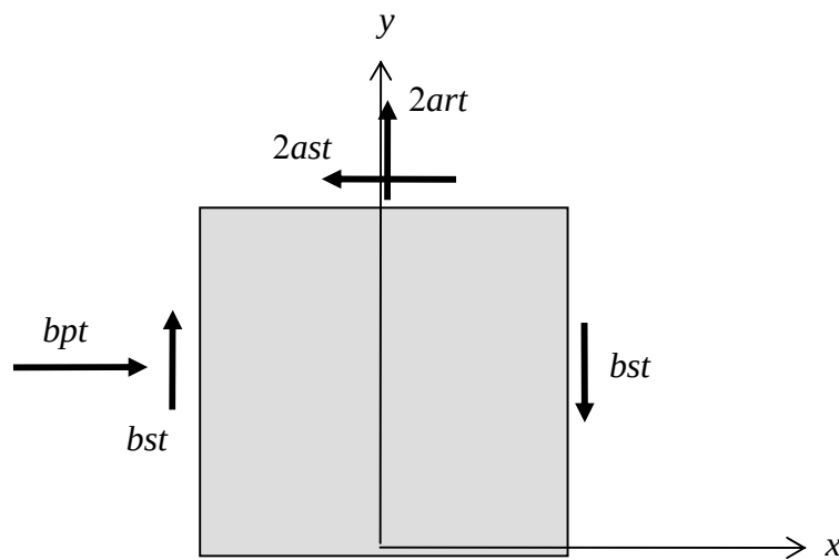
Figure 3.5.9: a free-body diagram of the plate in Fig. 3.5.7 showing the known resultant forces (forces on the lower boundary are not shown)
