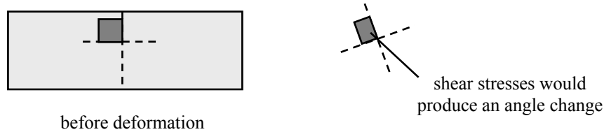
Figure 4.6.24: a section of beam before and after deformation
