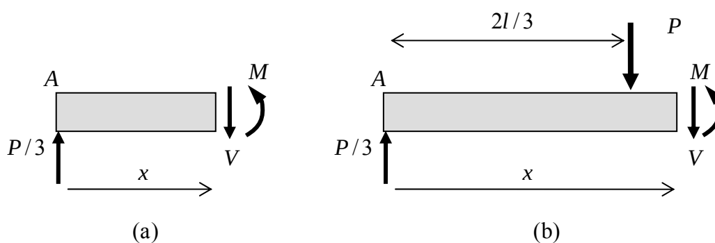
Figure 4.6.8: free body diagrams of sections of a beam
