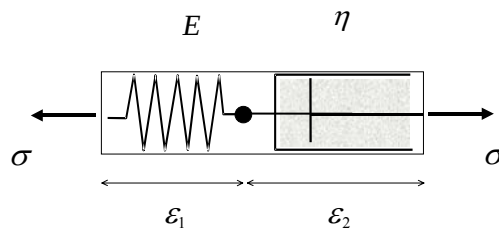
Figure 7.3.4: the Maxwell Model
