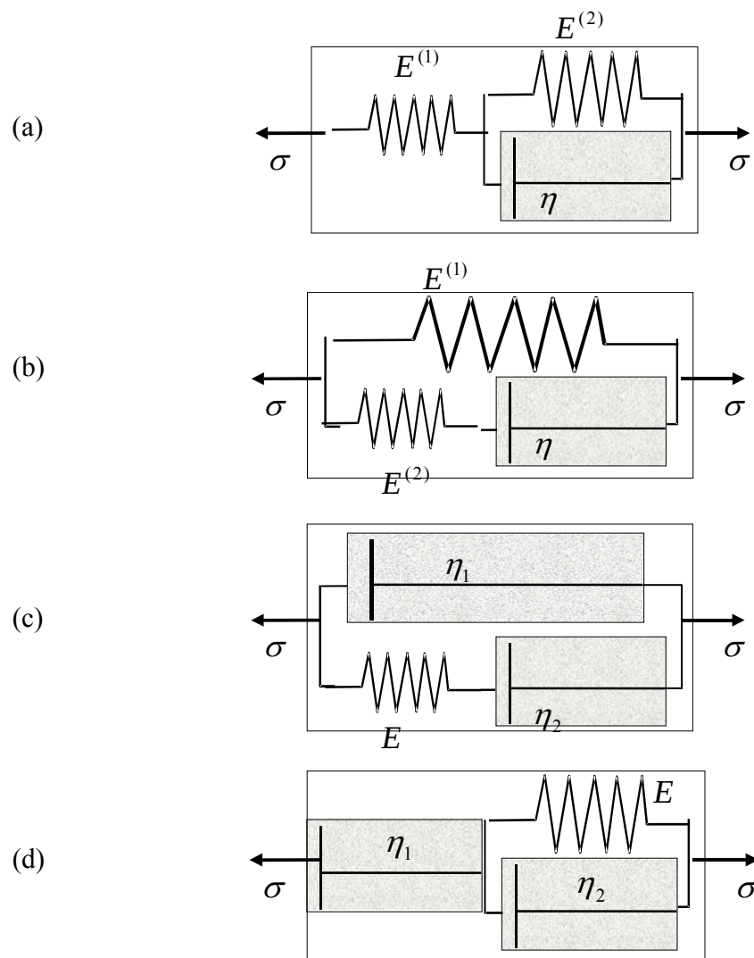
Figure 7.3.8: Three-element Models: (a) Standard Solid I, (b) Standard Solid II, (c) Standard Fluid I, (d) Standard Fluid II
