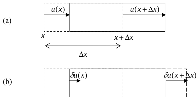
Figure 5.5.4: element undergoing actual and virtual displacements; (a) actual displacements, (b) virtual displacements
