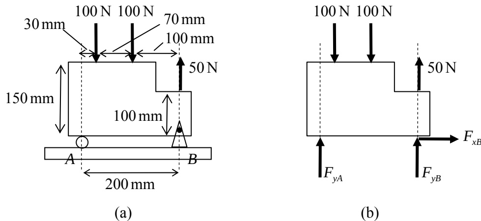
Figure 2.3.10: Equilibrium of a plate; (a) forces acting on the plate, (b) free-body diagram of the plate
