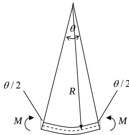
Figure 5.2.5: beam of length L under pure bending
