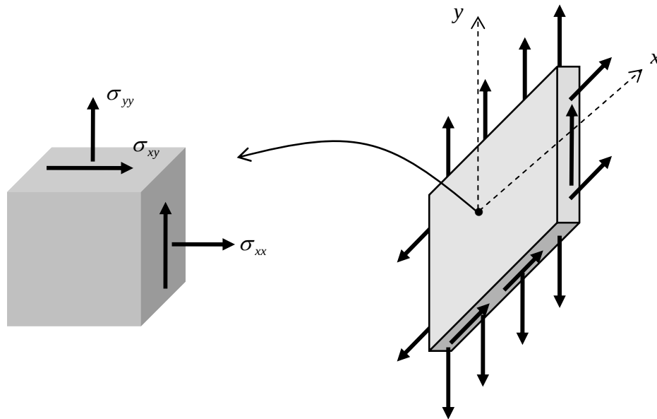
Figure 3.5.11: a thin material loaded in-plane, leading to a state of plane stress
