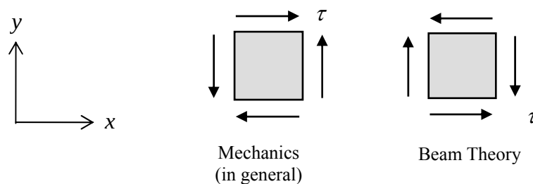
Figure 4.6.6: sign convention for shear stress in beam theory
