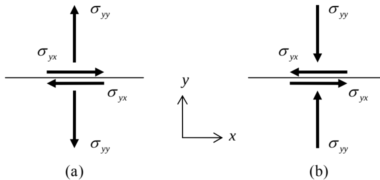
Figure 3.3.9: stresses acting on either side of a material surface: (a) positive stresses, (b) negative stresses
