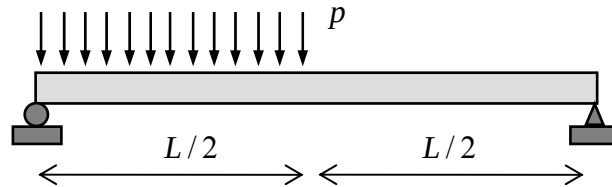
Figure 4.6.31: a simply supported beam subjected to a uniformly distributed load over half its length
