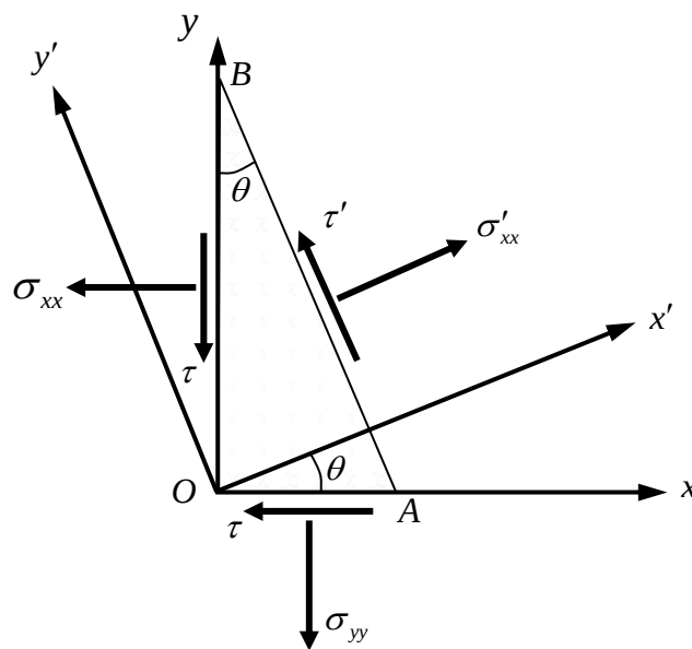
Figure 3.4.6: a free body diagram of a triangular element of material
