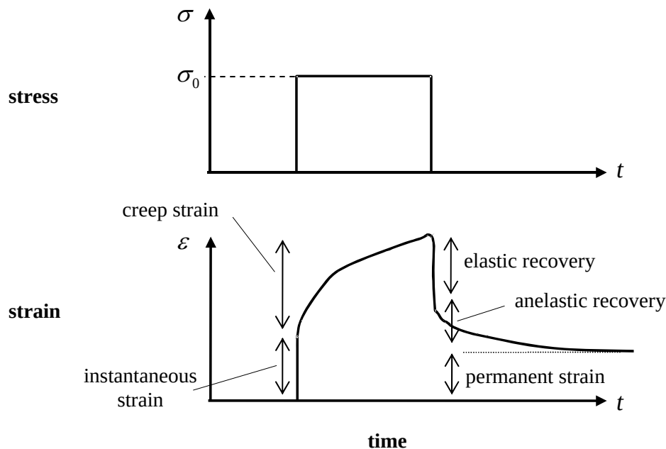
Figure 7.1.3: Strain response to the creep-recovery test
