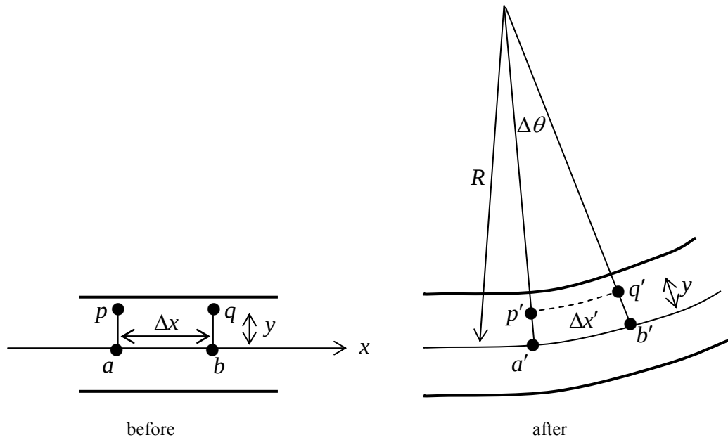
Figure 4.6.21: deformation of material fibres in an element of beam
