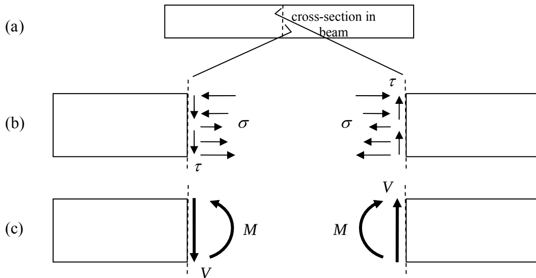
Figure 4.6.4: stresses and moments acting over a cross-section of a beam
