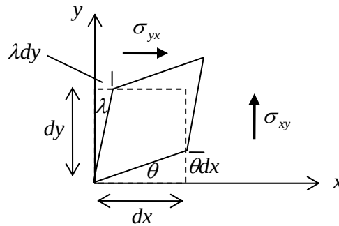
Figure 5.4.1: a volume element under shear stress
