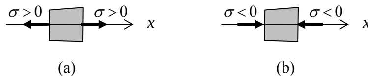
Figure 4.3.3: Stresses arising in the slender component; (a) positive (tensile) stress, (b) negative (compressive) stress
