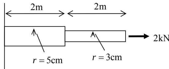
Figure 5.2.6: a loaded bar
