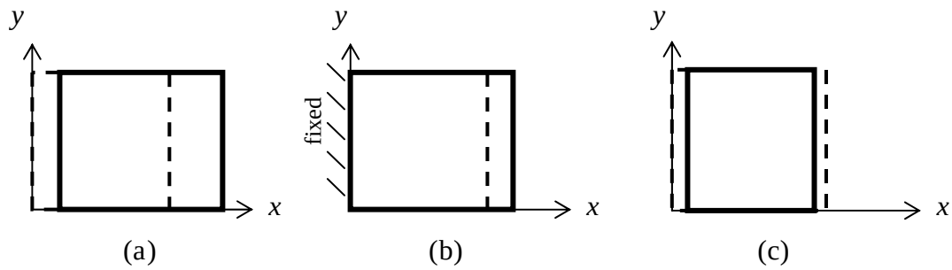
Figure 3.6.8: normal strain; (a) positive normal strain, (b) positive normal strain with the left-hand end fixed in space, (c) negative normal strain
