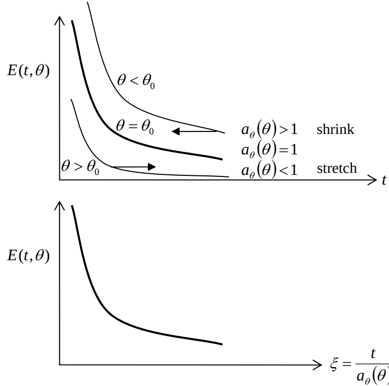
Figure 7.7.4: Relaxation modulus, as a function of (a) time, (b) reduced time
