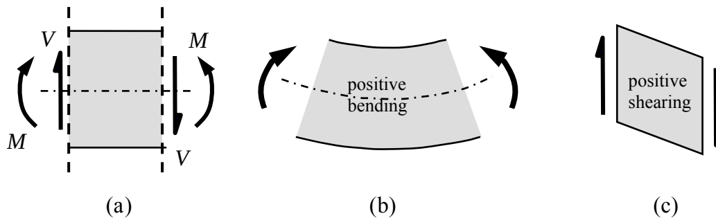
Figure 4.6.5: sign convention for moments and shear forces
