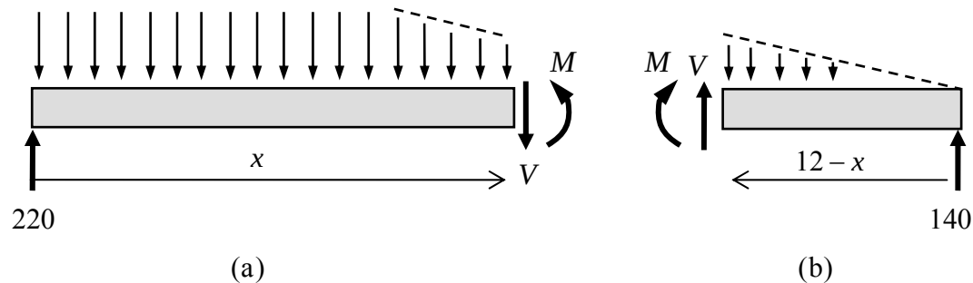
Figure 4.6.16: free body diagrams of sections of a beam
