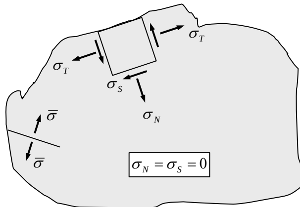
Figure 3.5.5: A free surface - the normal and shear stresses there are zero
