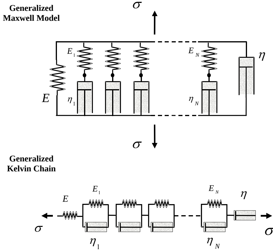
Figure 7.3.9: Generalised Viscoelastic Models
