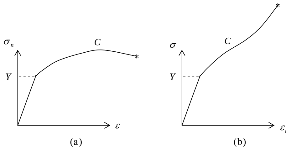
Figure 4.2.2: typical stress-strain curve for an engineering material; (a) engineering stress and strain, (b) true stress and strain
