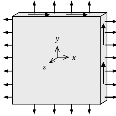
Figure 4.2.9: Plane stress - a thin component loaded in-plane
