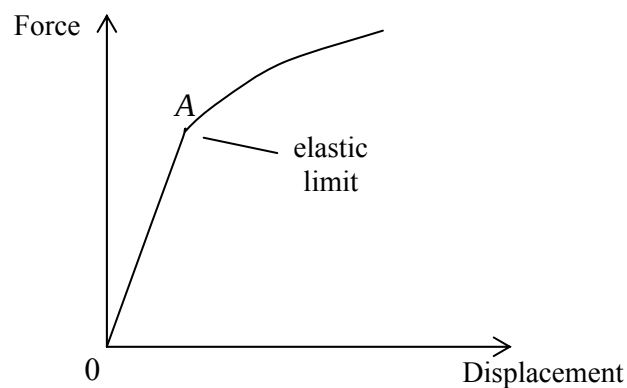
Figure 4.2.1: force/displacement curve for the tension test
