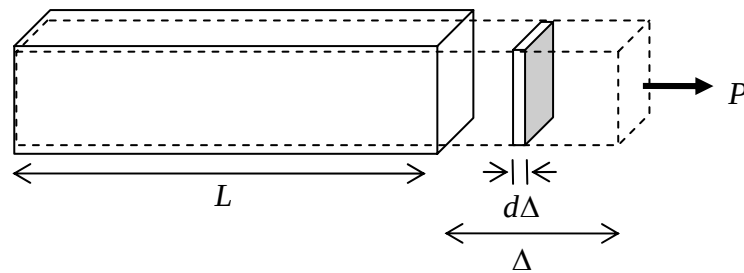
Figure 5.2.1: a bar loaded by a constant stress
