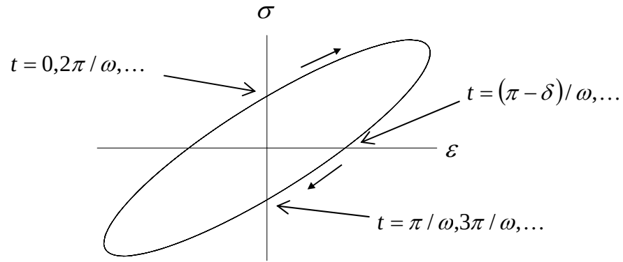
Figure 7.6.2: Elliptic Stress-Strain Hysteresis Loop
