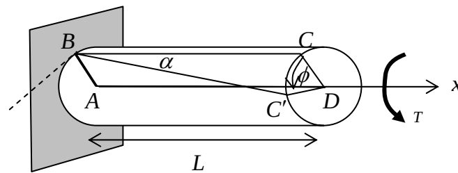
Figure 4.4.1: A cylindrical member under the action of a torque
