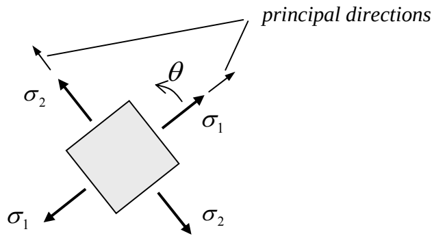
Figure 3.5.16: principal stresses and principal directions
