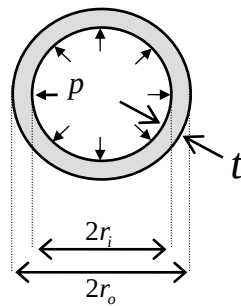
Figure 4.5.1: A pressurised container
