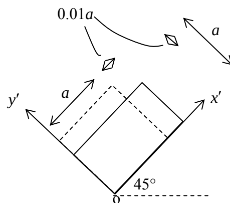
Figure 3.8.4: Principal strains for the block in pure shear
