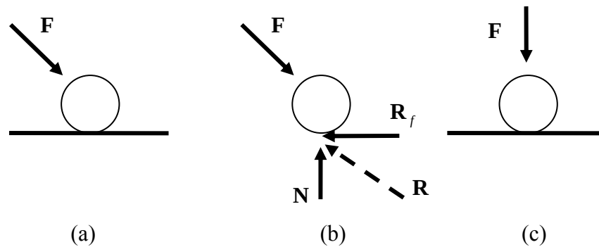
Figure 2.2.4: a particle sitting on a surface; (a) a rough surface, (b) a free-body diagram of (a), (c) a smooth surface
