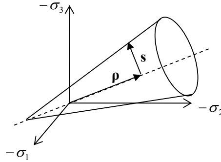
Figure 8.3.14: The Drucker-Prager yield surface
