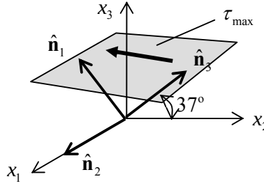
Figure 7.2.15: maximum shear stress
