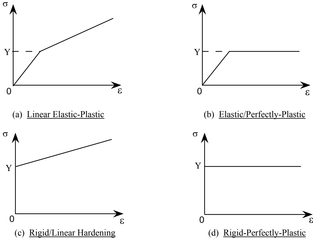
Figure 8.1.4: Simple models of elastic and plastic deformation
