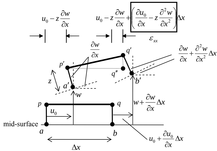
Figure 6.2.8: deformation of material fibres in the x direction
