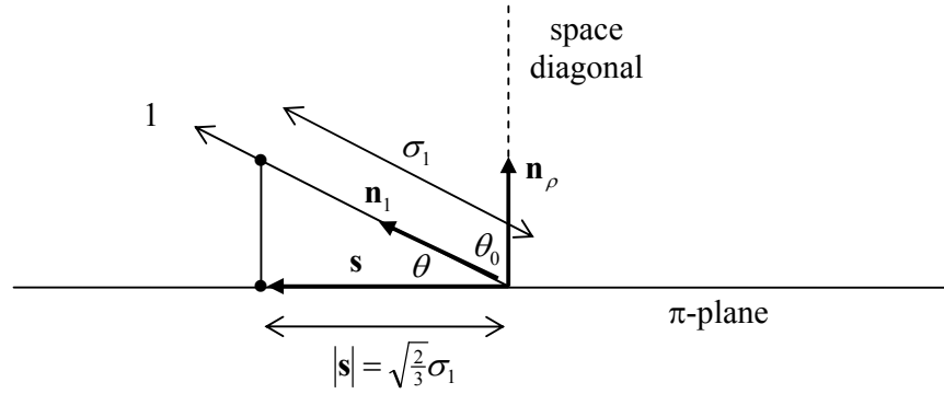
Figure 8.3.7: principal stress projected onto the \pi -plane
