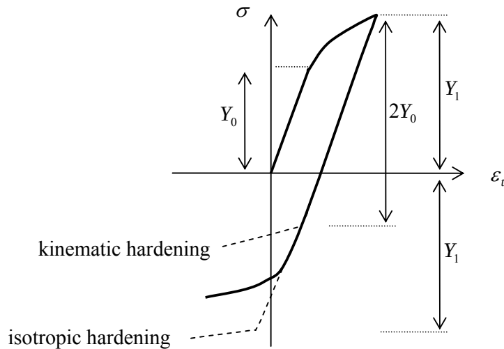
Figure 8.1.3: The Bauschinger effect
