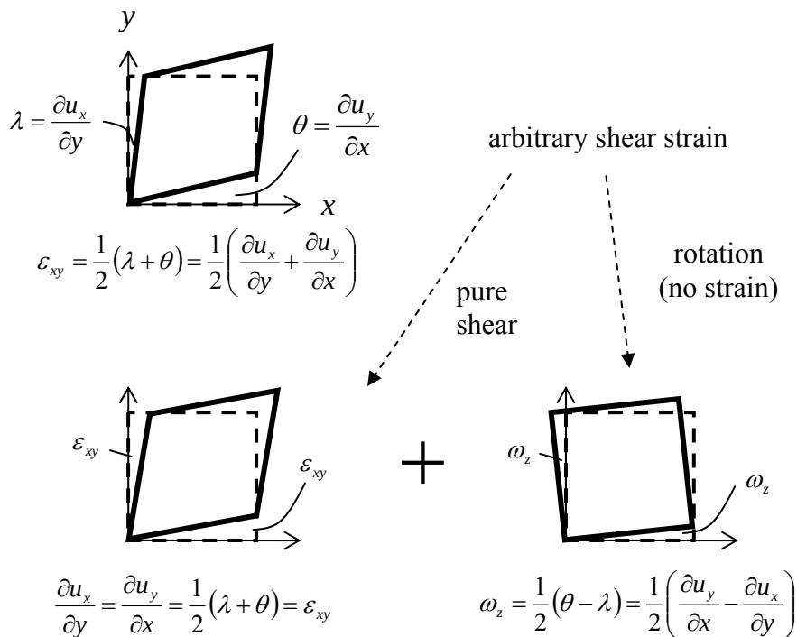
Figure 1.2.7: decomposition of a shear strain into a pure shear and a rotation
