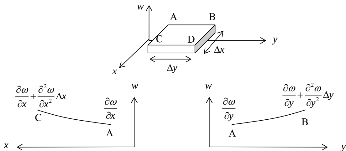
Figure 6.2.3: Physical meaning of the curvatures
