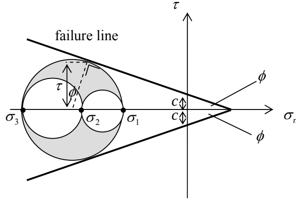
Figure 8.3.17: Mohr-Coulomb failure criterion
