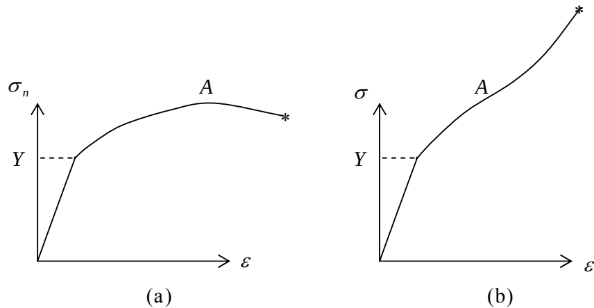
Figure 8.1.2: typical stress/strain curves; (a) engineering stress and strain, (b) true stress and strain
