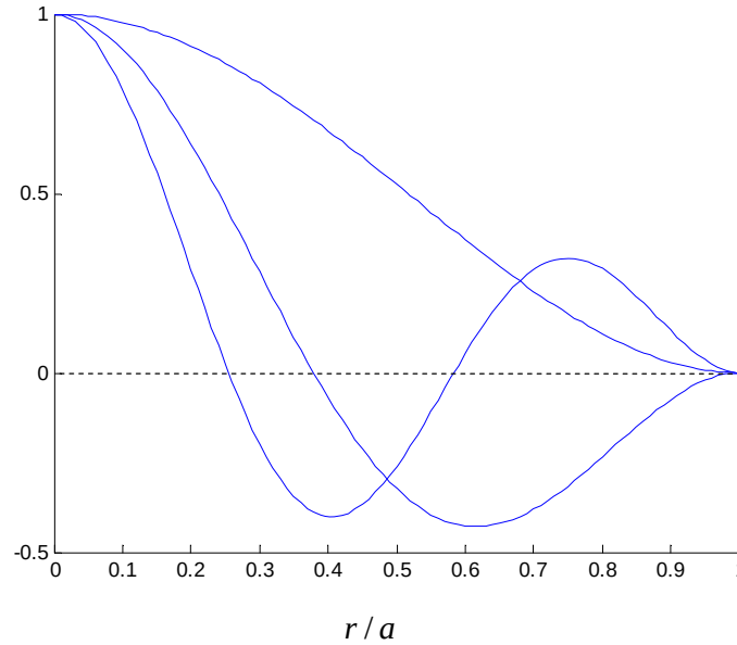
Figure 6.8.3: Mode shapes for the Clamped Circular Plate
