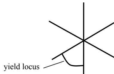
Figure 8.3.16: A typical sector of the yield locus for an isotropic material with different yield behaviour in tension and compression
