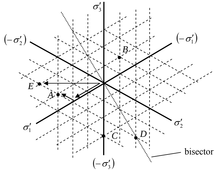
Figure 8.3.6: the \pi -plane
