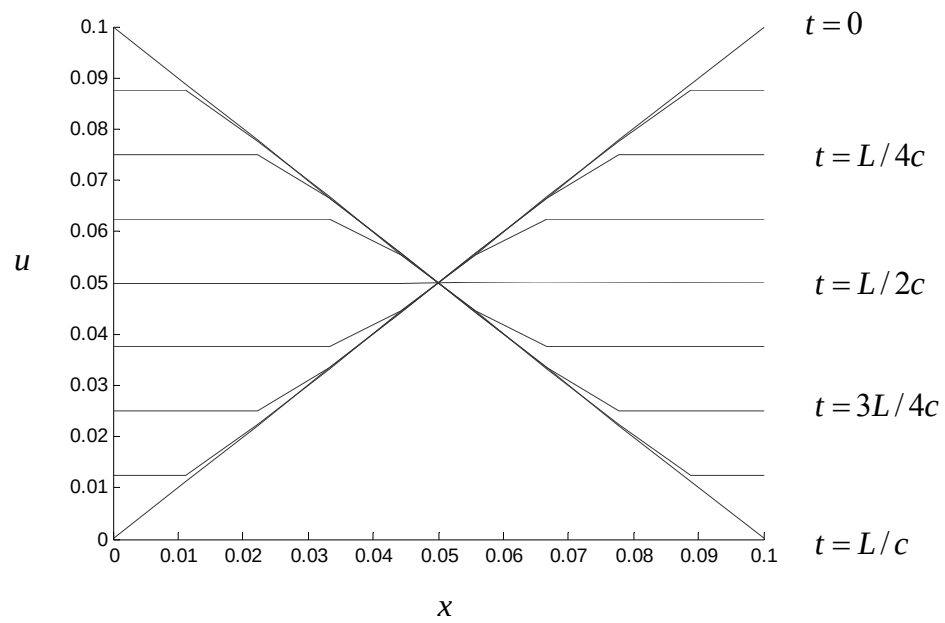
Figure 2.2.12: displacements for free-free example
