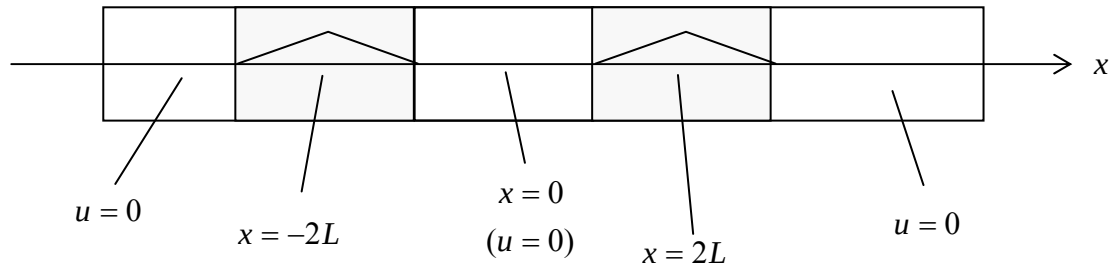
Figure 2.2.4: displacements at time 2L/c
