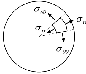
Figure 4.3.4: stress components in plane axisymmetric problems
