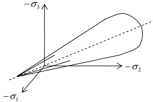
Figure 8.3.21: a capped yield surface
