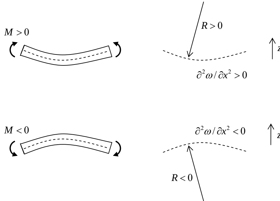
Figure 6.2.11: sign convention for curvatures and moments
