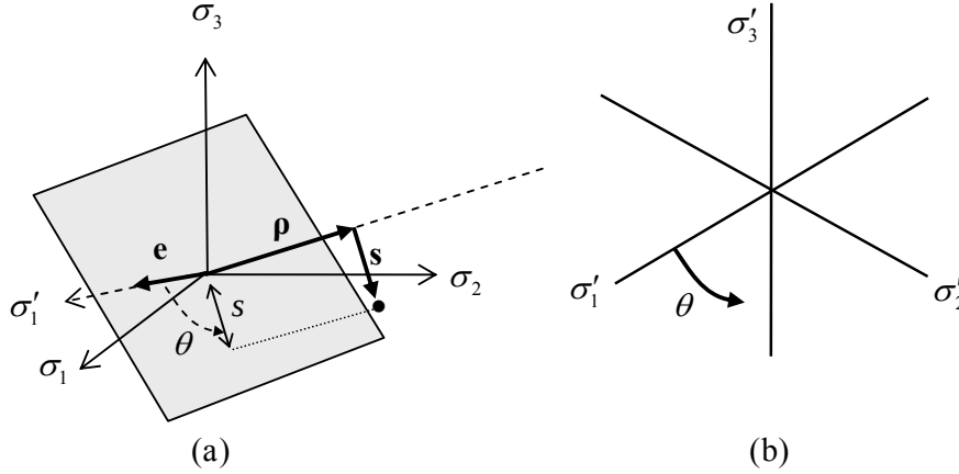
Figure 8.3.12: A point in stress space
