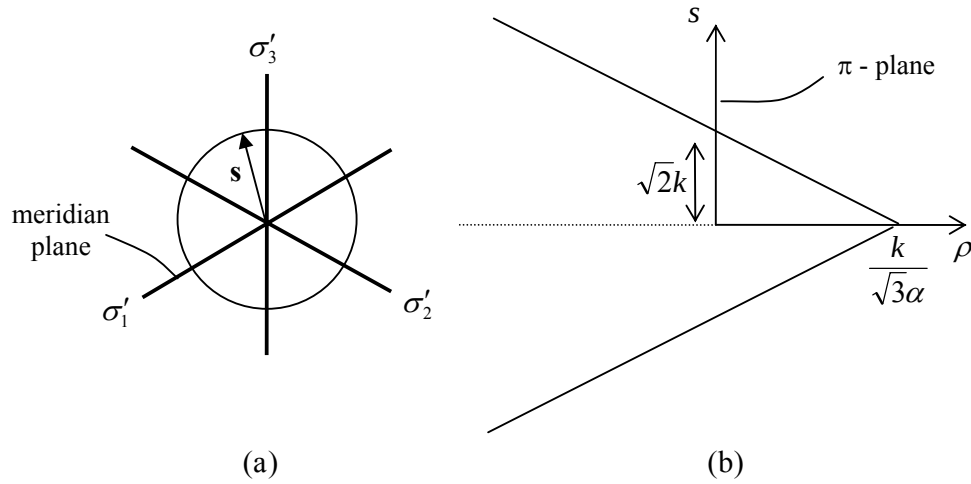
Figure 8.3.13: The Drucker-Prager criterion; (a) the \pi -plane, (b) the Meridian Plane
