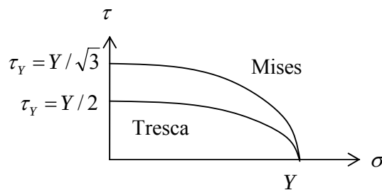
Figure 8.3.2: the yield locus for a thin-walled tube in combined tension and torsion
