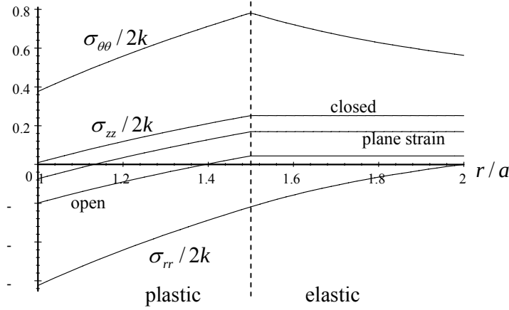
Figure 8.5.2: Stress field in the cylinder for the case of a = 1 , b = 2 , c = 1.5
