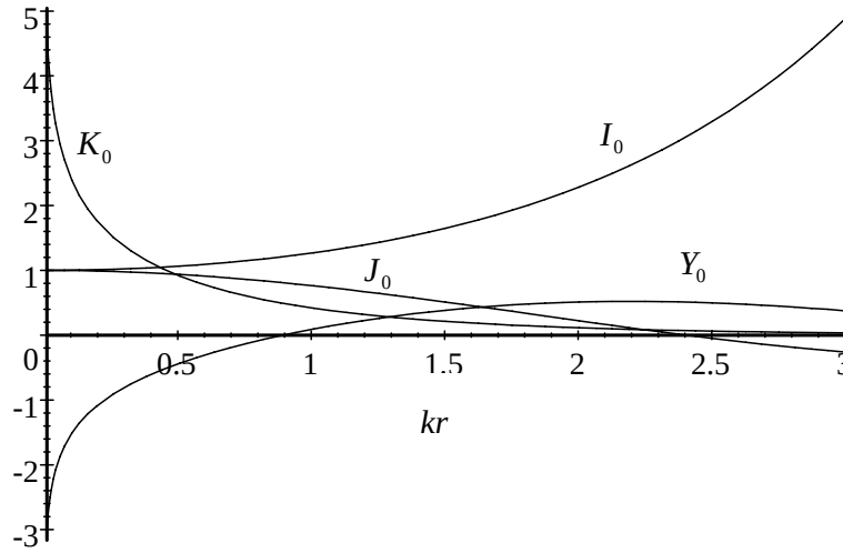
Figure 6.8.1: Bessel Functions
