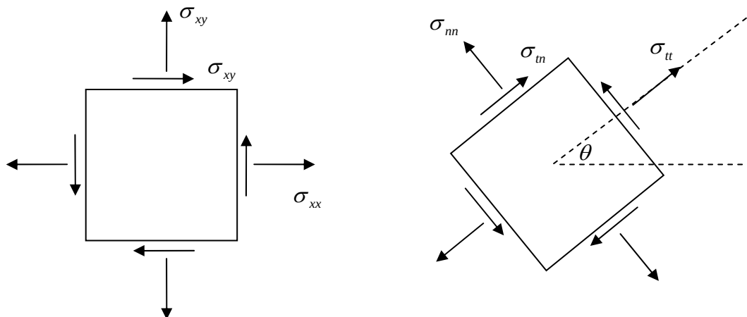
Figure 6.2.12: Plate Element; (a) stresses acting on element, (b) rotated element
