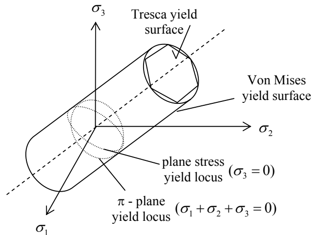
Figure 8.3.11: The Von Mises and Tresca yield surfaces
