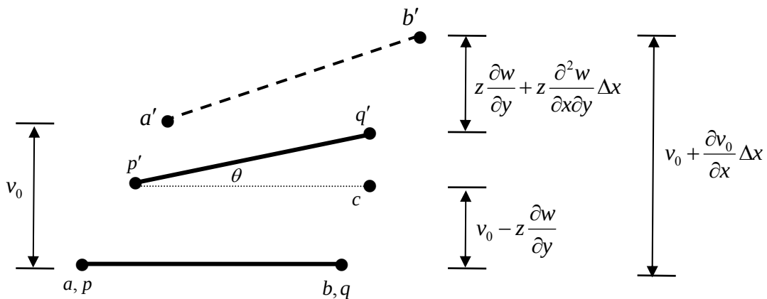
Figure 6.2.9: the deformation of 6.2.8 viewed “from above”; a', b' are the deformed positions of the mid-surface points a, b
