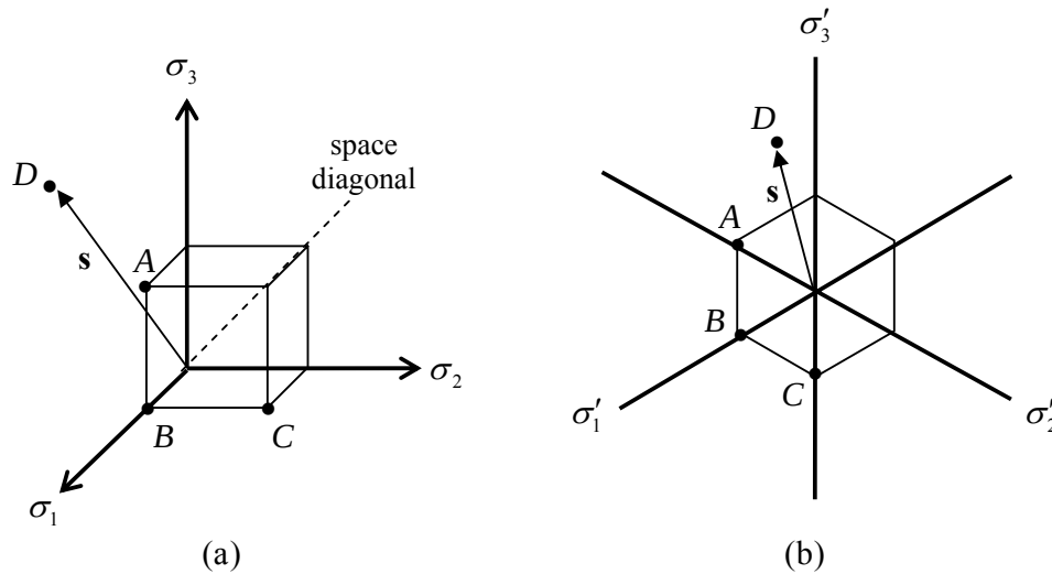
Figure 8.3.5: Stress space; (a) principal stress space, (b) the \pi – plane
