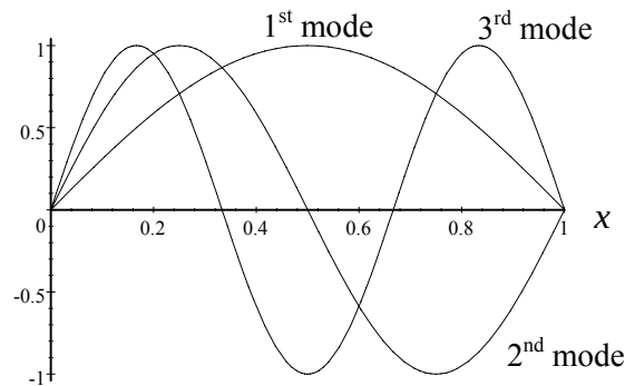
Figure 2.2.5: mode shapes for a vibrating elastic rod
