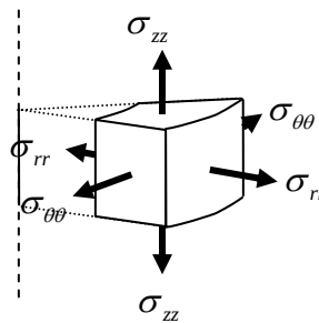
Figure 4.3.7: stress components in plane axisymmetric problems
