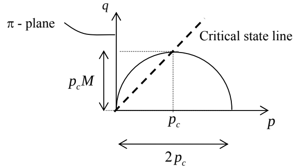
Figure 8.3.22: The modified Cam-Clay criterion in the Meridian Plane
