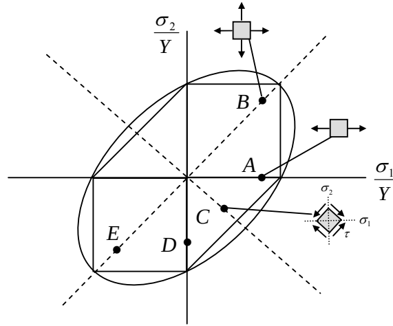
Figure 8.3.3: yield loci in 2D principal stress space
