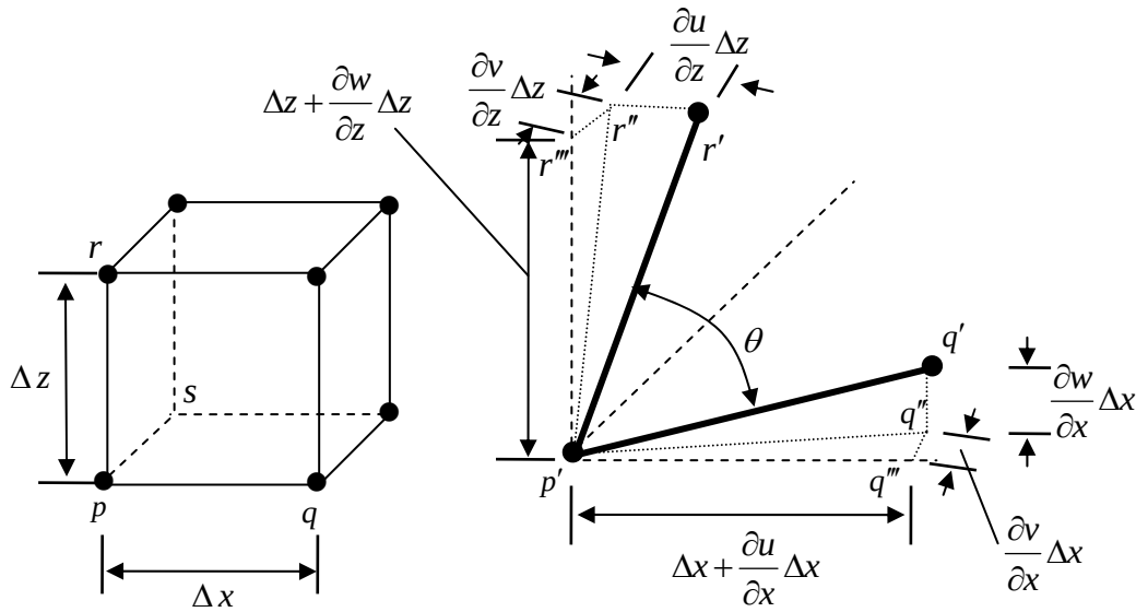
Figure 6.2.7: the deformation of Fig. 6.2.6, showing shear strains
