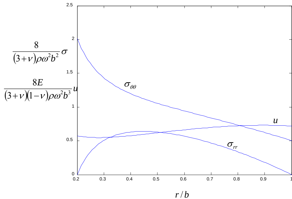
Figure 4.4.3: stresses and displacements in the hollow rotating disc
