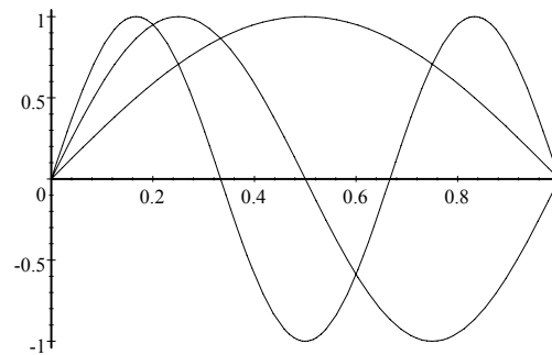
Figure 2.2.7: first three mode shapes for fixed-fixed
