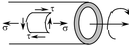
Figure 8.3.1: combined tension and torsion of a thin-walled tube
