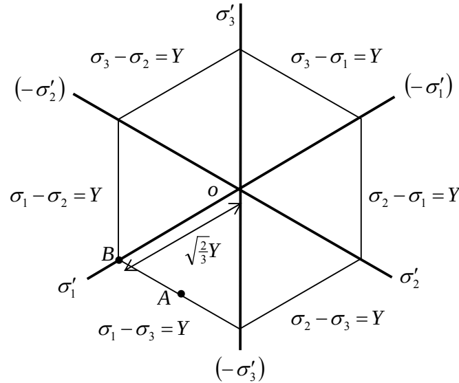
Figure 8.3.9: The Tresca criterion in the \pi -plane
