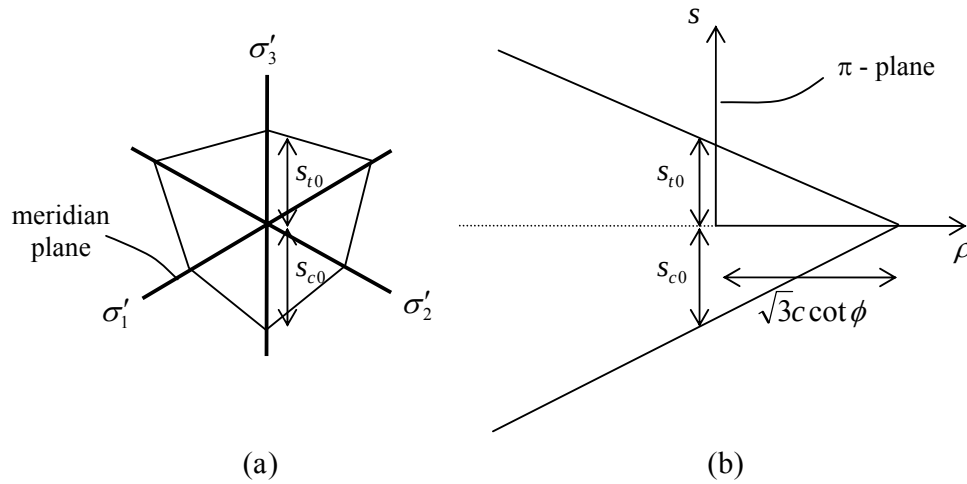
Figure 8.3.18: The Mohr-Coulomb criterion; (a) the \pi -plane, (b) the Meridian Plane
