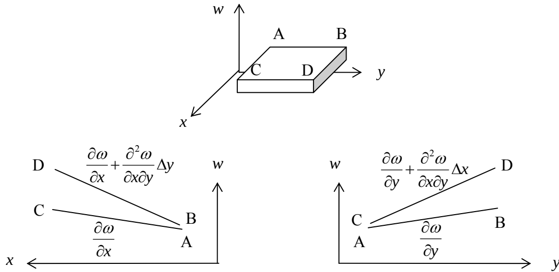
Figure 6.2.4: Physical meaning of the twist
