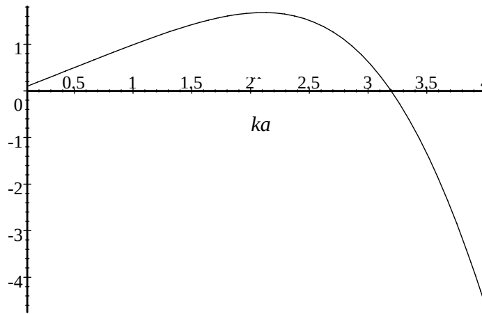
Figure 6.8.2: The Function 6.8.12
