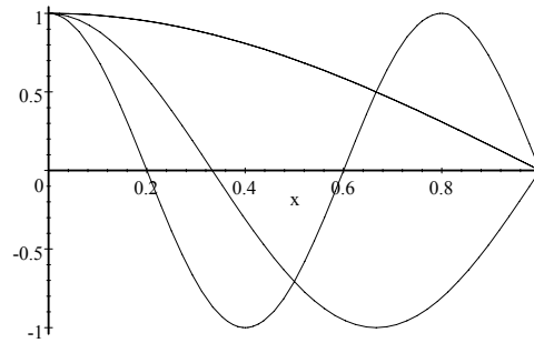
Figure 2.2.10: first three mode shapes for free-fixed
