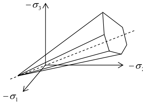
Figure 8.3.19: The Mohr-Coulomb yield surface
