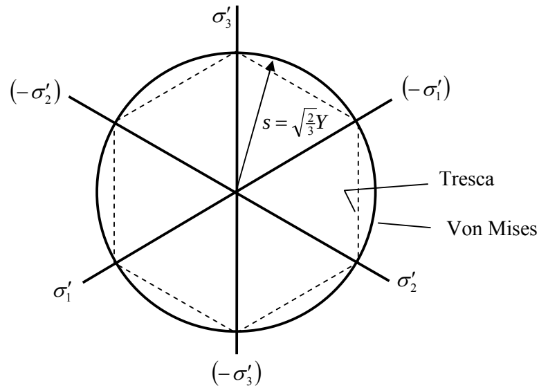
Figure 8.3.10: The Von Mises criterion in the \pi -plane
