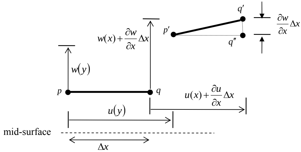
Figure 6.2.6: deformation of a material fibre in the x direction
