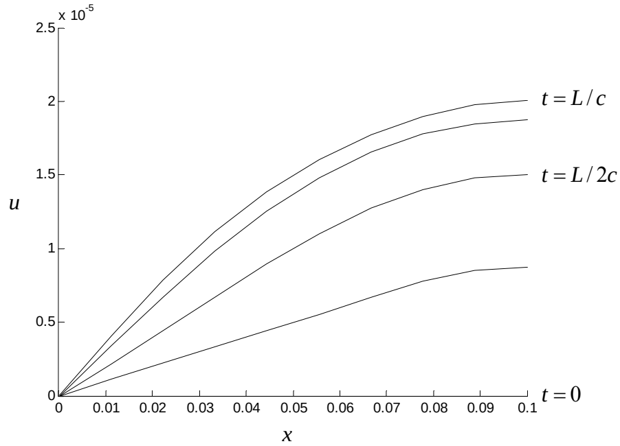
Figure 2.2.11: displacements for fixed-free example
