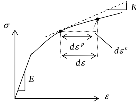
Figure 8.1.5: The tangent modulus
