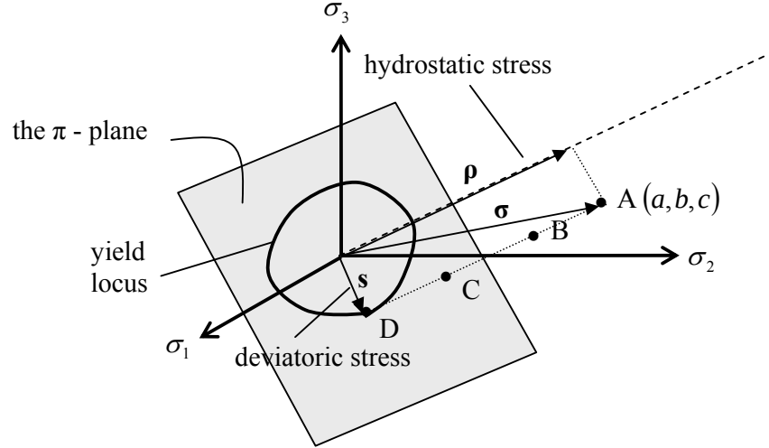
Figure 8.3.4: Yield locus/surface in three dimensional stress-space
