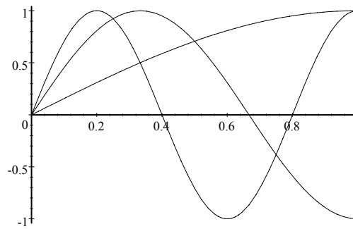
Figure 2.2.9: first three mode shapes for fixed-free
