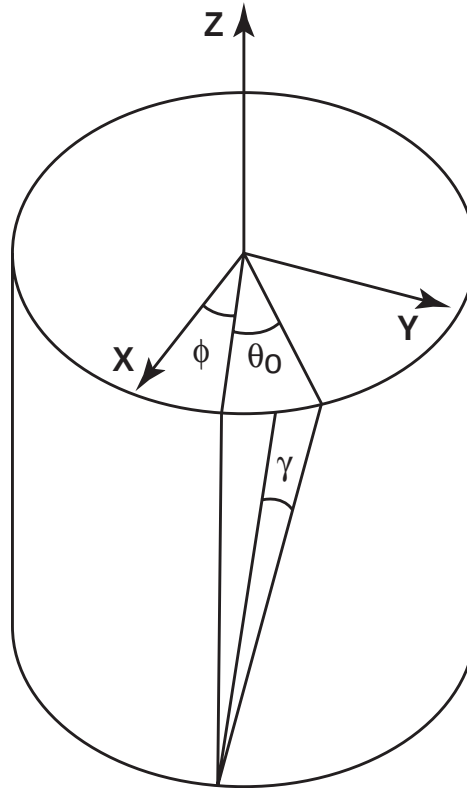
Fig. 7.1. Cylinder in torsion. The angle \gamma = \tan^{-1}(r\theta'_0 / 2Z) proves to be a convenient measure of deformation.
