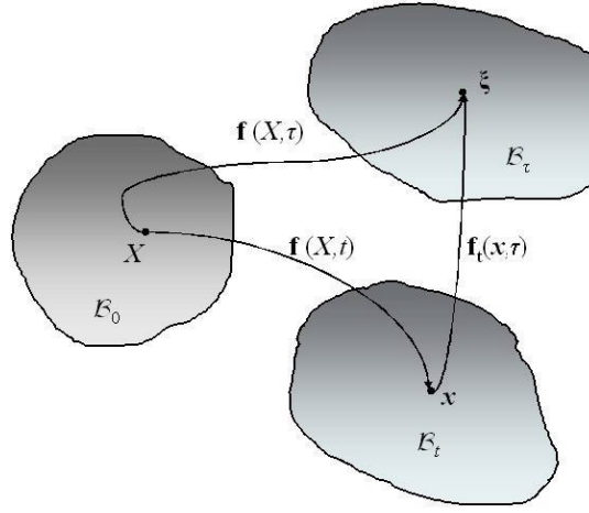
Fig. 2.6: Three configurations yielding Eulerian description
