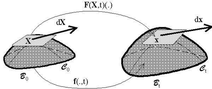
Fig. 2.1: Transformation from the reference configuration B_0 to the current configuration B_t . The function of motion f describes time changes of position of material points X \in B_0 into x \in B_t while the deformation gradient F describes the transformation of material vectors (e.g. a tangent vector dX of the curve C_0 into a tangent vector dx of the curve C_t )
