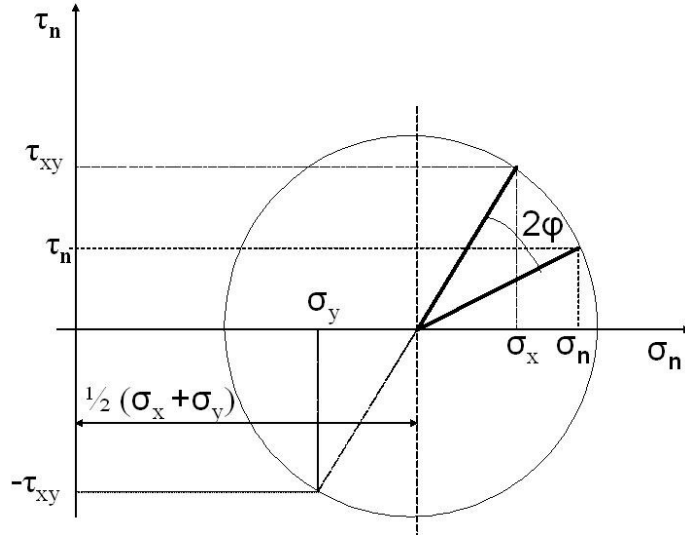
Fig. 3.5: Mohr's circle
