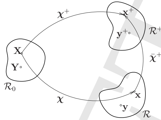
Figure 3.18: Configurations associated with motions \chi and \chi^+ differing by a superposed rigid motion \bar{\chi}^+ .
