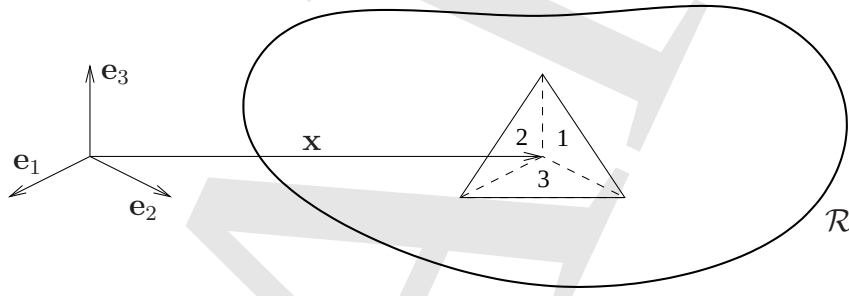
Figure 4.5: The Cauchy tetrahedron.
