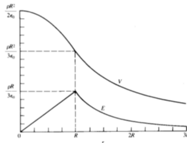
Fig. 3-6. The potential V and the electric field strength E as functions of the radial distance r from a spherical charge distribution of radius R and volume charge density \rho .
