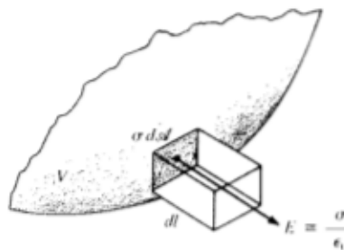
Fig. 10-7. Thought experiment for calculating the energy stored in an electric field in the presence of dielectrics. The shaded volume of area \mathcal{A} is a conductor that expands slowly, from one equipotential surface to the next. The surface charge density is \sigma . The element of area d\mathcal{A} moves out by a distance d\mathbf{l} .
