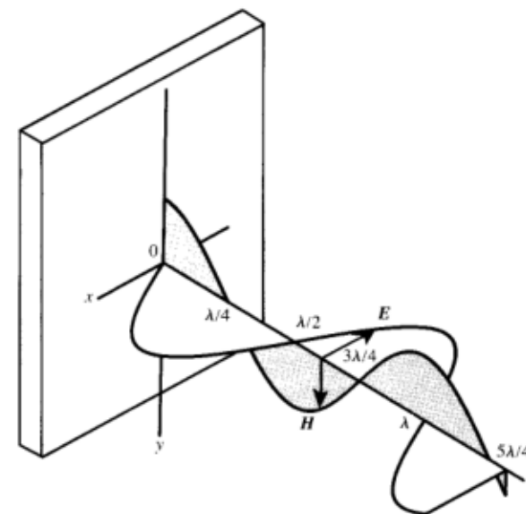
Fig. 32-4. The standing wave pattern for reflection at normal incidence on a good conductor, at a particular time. Nodes of \mathbf{E} and of \mathbf{H} are spaced \lambda/4 apart.
