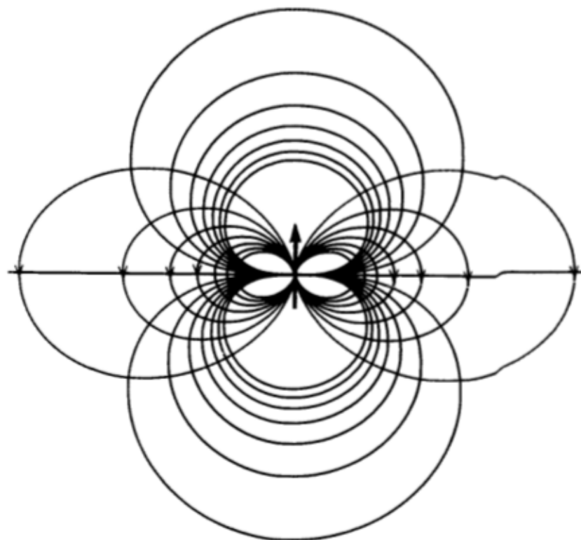
Fig. 5-2. Lines of \mathbf{E} , shown with arrows, and equipotential lines for the electric dipole of Fig. 5-1. In the central region the lines become too close together to be shown. The central arrow is the vector \mathbf{p} .
