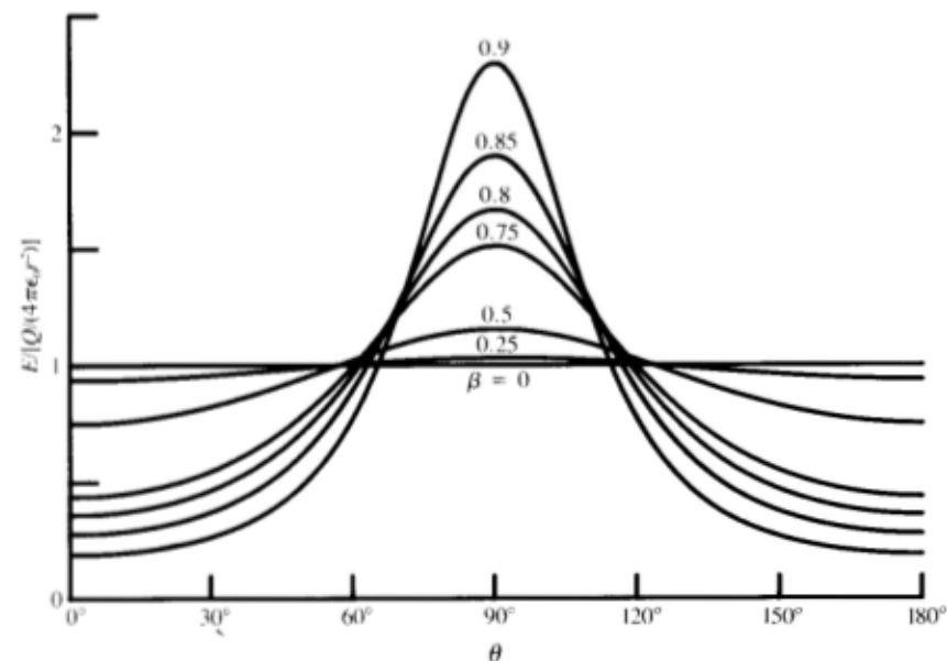
Fig. 16-6. The E of a moving point charge as a function of the polar angle \theta of Figs. 16-3 and 16-5, for seven values of \beta = v/c . The observer is stationary and sees the charge moving at the uniform speed v . For \beta = 0 the field is isotropic. It is hardly disturbed at \beta = 0.25 . As the speed increases, the field increases near \theta = 90^\circ and decreases both ahead of the charge (near \theta = 0 ) and behind it (near \theta = 180^\circ ). At extremely high velocities, most of the electric field concentrates near \theta = 90^\circ . These curves explain qualitatively the validity of Gauss's law for moving charges: as the speed increases, the flux of E shifts from the region where \theta = 0 and \theta = 180^\circ to \theta \approx 90^\circ , and the total flux of E remains constant. (Then why are the areas under the curves not equal?) Note that the electric field is symmetric about 90^\circ . Thus there is no way of telling from the shape of the field whether the charge is moving to the right or to the left.
