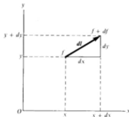
Fig. 1-3. A scalar-point function changes from f to f + df over the distance dl .
