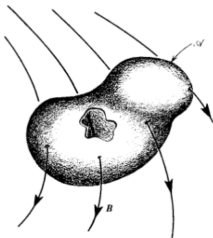
Fig. 27-2. Lines of B passing through a closed surface. The net outward flux of B is equal to zero.
