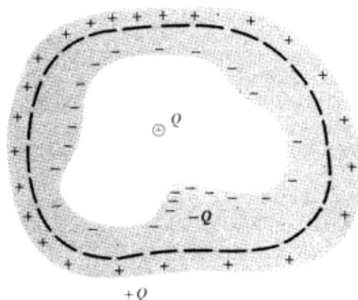
Fig. 4-4. Section through a hollow conductor enclosing a body that carries a net charge Q . The dashed line is a section through a Gaussian surface lying entirely in the conducting material, where E = 0 .
