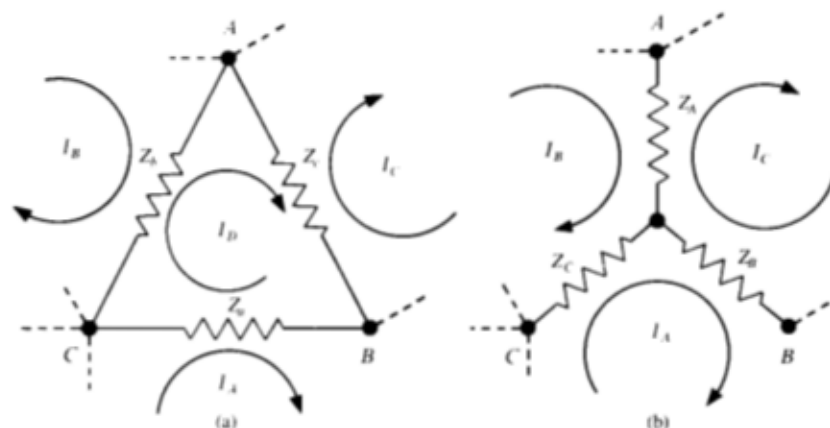
Fig. 8-15. The three nodes A , B , C are part of a larger circuit. (a) The three nodes are delta-connected. (b) The nodes are star-connected. Under certain conditions the delta is completely equivalent to the star, but only at a given frequency. If the six Z 's are all resistances, then the equivalence is valid at all frequencies.
