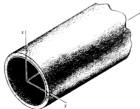
Fig. 33-1. Hollow conducting waveguide.
