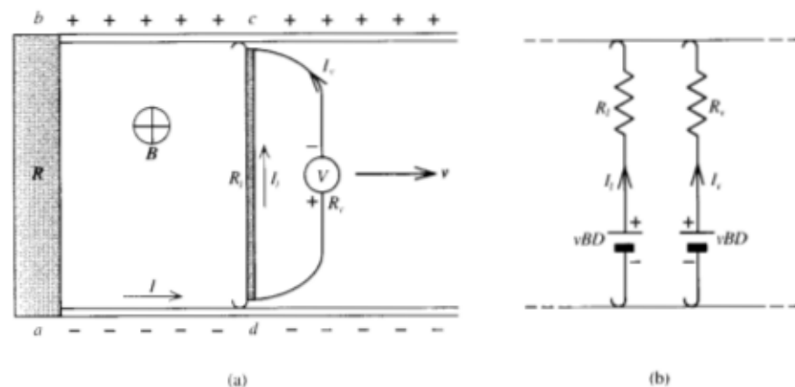
Fig. 23-4. (a) Voltmeter V connected across the link in the generator of Fig. 23-3. (b) Equivalent circuit.
