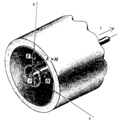
Fig. 33-4. The E , H , and E \times H vectors inside a coaxial line.
