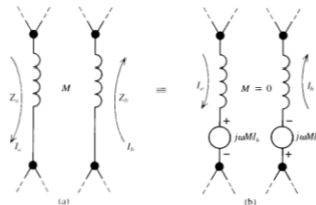
Fig. 25-5. (a) Part of a circuit in which there exists a mutual inductance M between two branches. (b) Equivalent circuit.
