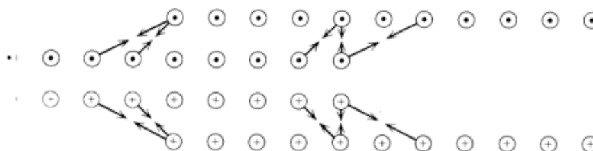
Fig. 26-6. Section through part of the solenoids of Fig. 26-5. There is a force of attraction at the ends of the solenoids.
