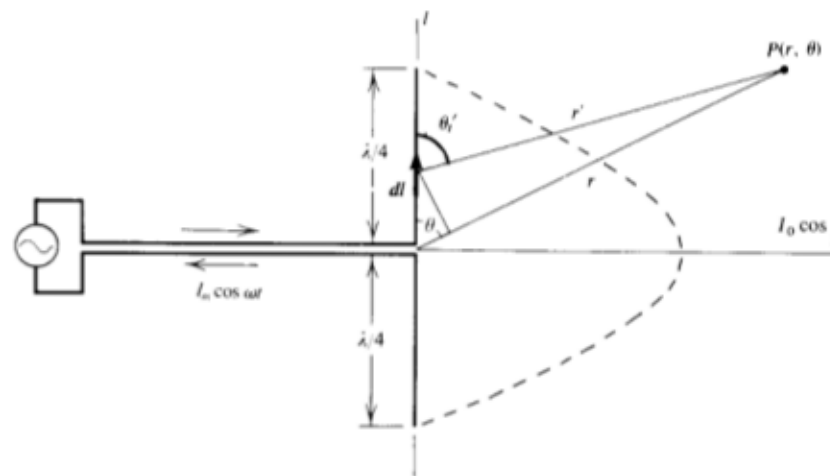
Fig. 39-1. Half-wave antenna. The broken line shows the standing wave of current at \cos \omega t = 1 .
