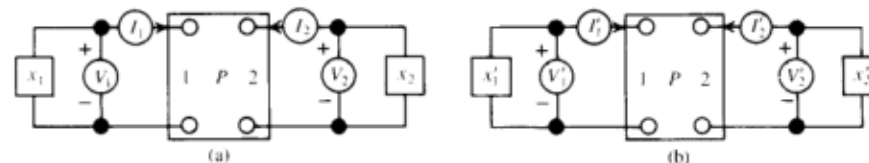
Fig. 8-9. Identical passive and linear circuits P connected to external elements in two different ways. As usual, a circled V represents an infinite-resistance voltmeter, and a circled I a zero-resistance ammeter. The signs and the arrows show which directions are taken to be positive.
