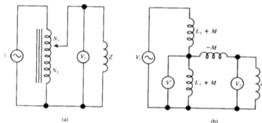
Fig. 25-10. (a) Schematic diagram of an autotransformer. (b) The equivalent circuit.
