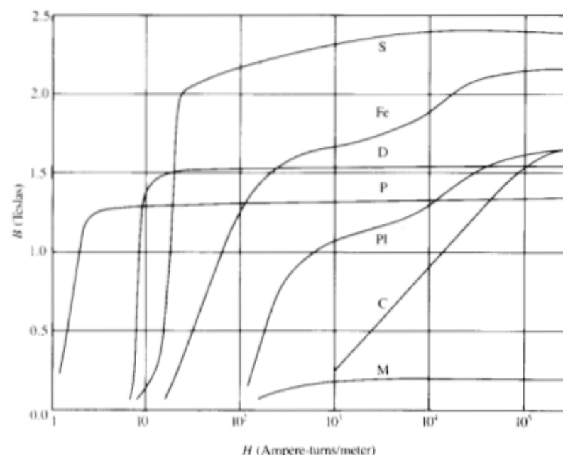
Fig. 20-5. Magnetization curves for various materials: S, Supermendur; Fe, annealed pure iron; D, Deltamax; P, Permalloy; PI, powdered iron; C, gray cast iron; M, Monel.
