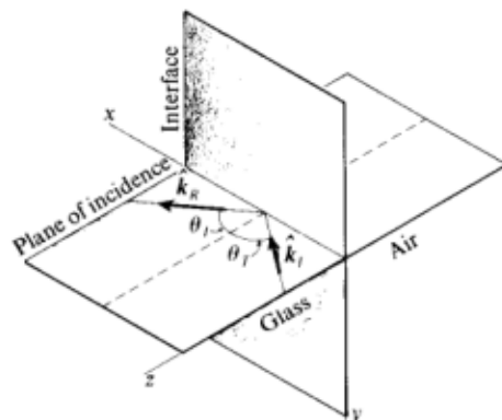
Fig. 31-1. For angles of incidence \theta_i larger than the critical angle \theta_c , the interface acts as a perfect mirror. This is total reflection.
