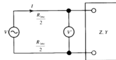
Fig. 24-9. A load impedance Z = R_{\text{load}} + jX , or an admittance Y = G_{\text{load}} + jB , connected to a source through a line of resistance R_{\text{line}} . The line resistance is equal to twice the resistance of one wire.
