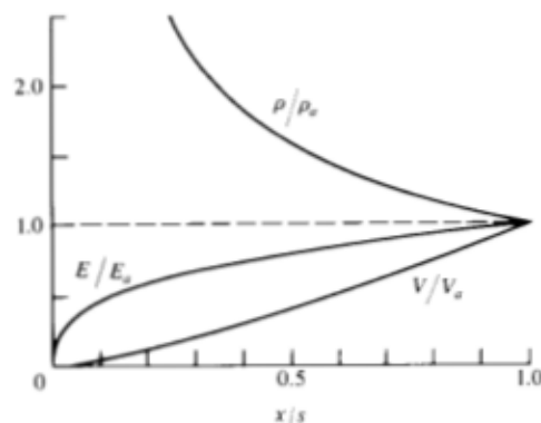
Fig. 4-2. The space charge density \rho , the electric field strength E , and the potential V as functions of the distance x from the cathode of a plane-parallel diode. The subscript a refers to the value of the variable at the anode.
