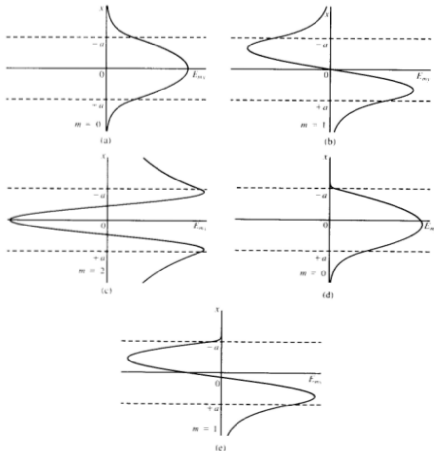
Fig. 36-3. (a), (b), (c) Curves of E_{my} as a function of x for the symmetric guide of Table 36-1. (d), (e) Curves of E_{my} for the asymmetric guide of Table 36-2.
