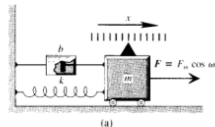
Fig. 2-3. Mass m subjected to a force F = F_m \cos \omega t , to a restoring force -kx exerted by a spring, and to a damping force -b dx/dt exerted by a dashpot. At rest, x = 0 .
