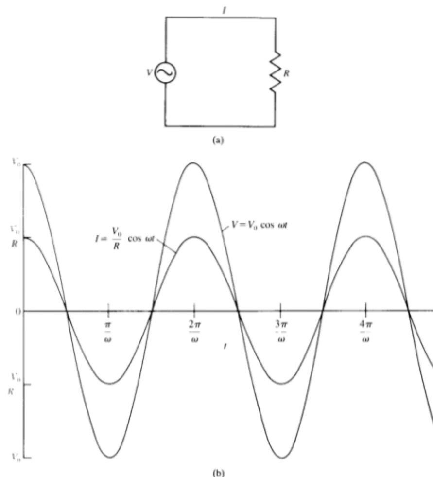
Fig. 7-11. (a) Resistor R connected to a source supplying a voltage V and a current I . (b) V and I plotted as functions of t for a resistor.
