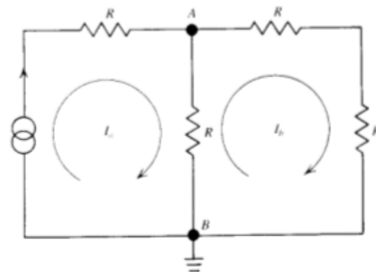
Fig. 7-6. Two-mesh resistive circuit fed by a source supplying a steady current I_a .
