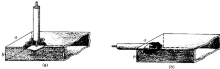
Fig. 34-1. Rectangular metallic waveguides fed by a coaxial line. (a) A quarter-wave antenna injects an electric field at a distance of \lambda_z/4 from the closed end of the guide. (b) A small loop antenna injects a magnetic field.
