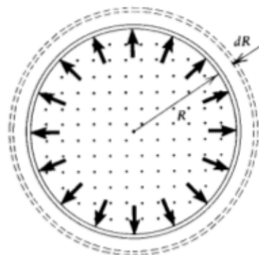
Fig. 26-9. End view of a solenoid. The dots represent lines of B , normal to the paper. The arrows show how the magnetic pressure pushes the winding away from the field.
