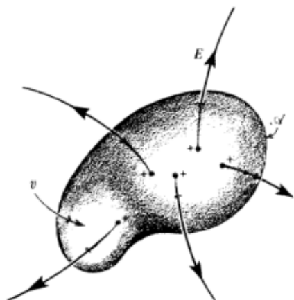
Fig. 27-1. Lines of E emerging from a volume containing a net charge Q . The outward flux of E is equal to Q/\epsilon_0 .
