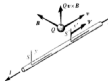
Fig. 16-8. A positive charge moves at a velocity v parallel to a straight wire carrying a current I . The magnetic force Q\mathbf{v} \times \mathbf{B} is in the direction shown because, for the charge Q , the wire is positively charged. If Q is positive, the force is repulsive.
