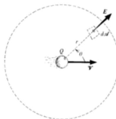
Fig. 17-1. Gauss's law applies to a moving charge: the surface integral of the normal component of the E field of a moving charge Q , evaluated over a fixed sphere, is equal to Q/\epsilon_0 , as if the charge were stationary. The excess field near \theta = \pi/2 just compensates the weak field near \theta = 0 and \theta = \pi . See Figs. 16-5 and 16-6.
