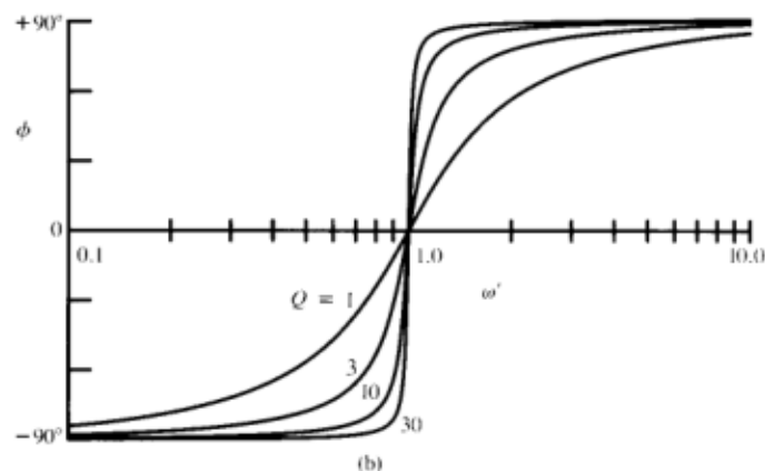
Fig. 25-2. (a) R/|Z| as a function of \omega' = \omega/\omega_0 for the circuit of Fig. 25-1 and for various values of Q . (b) The phase \phi of Z as a function of \omega' for the same values of Q .
