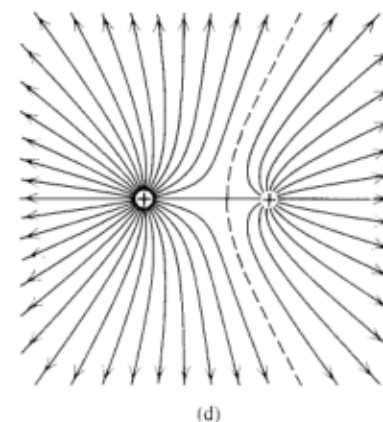
Fig. 6-6. Lines of \mathbf{E} between pairs of line charges. It is useful to visualize attractive electric forces as being caused by a tension in the lines of \mathbf{E} , as in (a) and (c). Similarly, repulsive electric forces may be thought of as being caused by a lateral repulsion between lines of \mathbf{E} , as in (b) and (d). In (c) and (d) the charge on the left is twice as large as the other.
