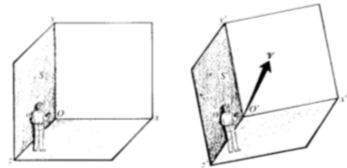
Fig. 13-1. Reference frames S and S' , with S' moving at some arbitrary constant velocity \mathbf{V} with respect to S , without rotation. Observers o and o' perform various experiments, each one in his or her own frame.
