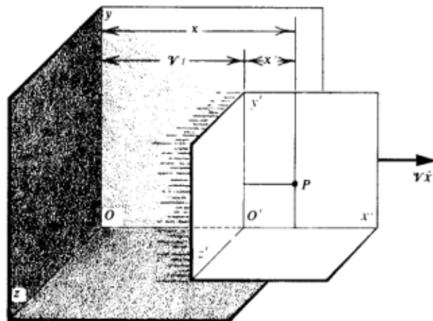
Fig. 13-2. The reference frame S' moves at a velocity V\hat{x} with respect to S .
