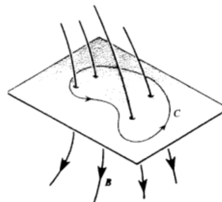
Fig. 27-3. If the magnetic flux linking C increases, it induces an electromotive around C in the direction of the arrow. The electromotive points in the same direction if B points upward and decreases.
