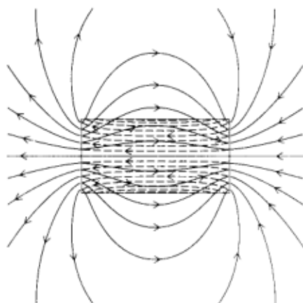
Fig. 21-3. Lines of H (solid) for a uniformly magnetized cylinder, with M uniform, parallel to the axis, and pointing to the left. Lines of B are shown broken inside the magnet; outside they follow the lines of H . This figure is identical to Fig. 9-4.
