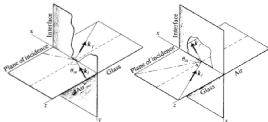
Fig. 30-7. If the angle of incidence is equal to the Brewster angle and if \mathbf{E} lies in the plane of incidence, there is no reflected wave. The position of the missing reflected ray is at 90^\circ to the transmitted ray.
