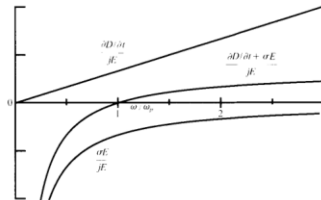
Fig. 29-3. The current densities \partial \mathbf{D} / \partial t , \sigma \mathbf{E} , and their sum, as functions of \omega / \omega_p in a plasma.
