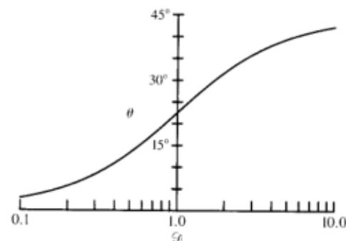
Fig. 28-4. The phase of E with respect to H as a function of \mathcal{D} in a wave traveling through a conducting medium.
