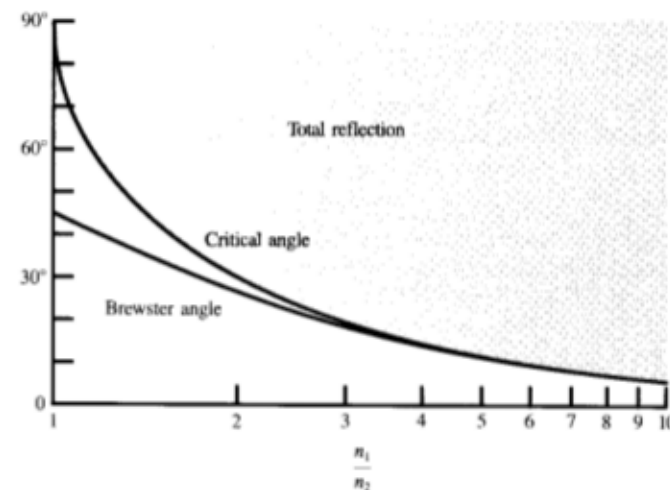
Fig. 31-9. The critical angle and the Brewster angle as functions of the ratio n_1/n_2 . The incident wave is linearly polarized with the \mathbf{E} vector parallel to the plane of incidence for the Brewster angle curve.
