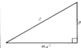
Fig. 15-5. The relativistic energy \mathcal{E} is related to the rest energy m_0c^2 and to the relativistic momentum p as in this right-angled triangle.
