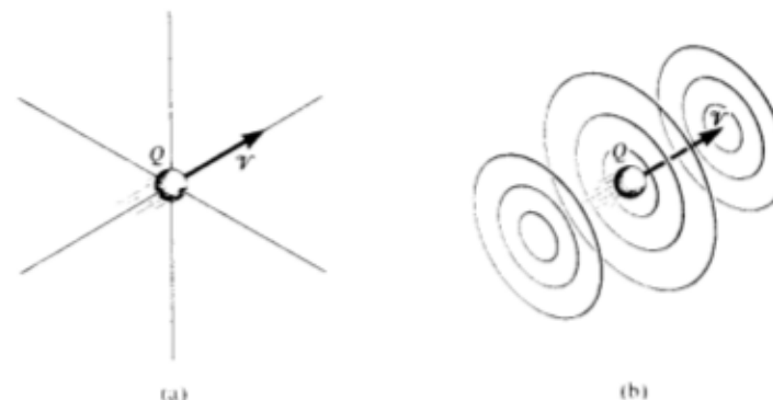
Fig. 16-4. (a) Lines of \mathbf{E} and (b) lines of \mathbf{B} for a positive charge Q moving at a constant velocity \mathbf{V} , as seen by a stationary observer.
