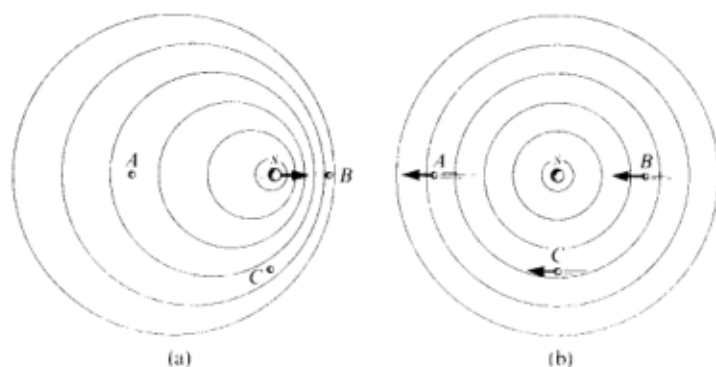
Fig. 14-5. The Doppler effect. (a) Source S moves to the right with respect to stationary receivers A , B , C . (b) The source is stationary, and the receivers all move to the left. The frequency shifts are the same in the two figures. The measured frequency is lower than the proper frequency at A , and higher at B . At C , the measured frequency is either lower or higher than the proper frequency, as in Prob. 14-7.
