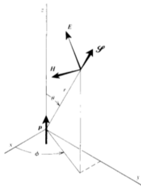
Fig. 38-7. The \mathbf{E} , \mathbf{H} , and \mathcal{S} = \mathbf{E} \times \mathbf{H} vectors for an oscillating electric dipole for r \gg \lambda and \omega[t] = 0 .
