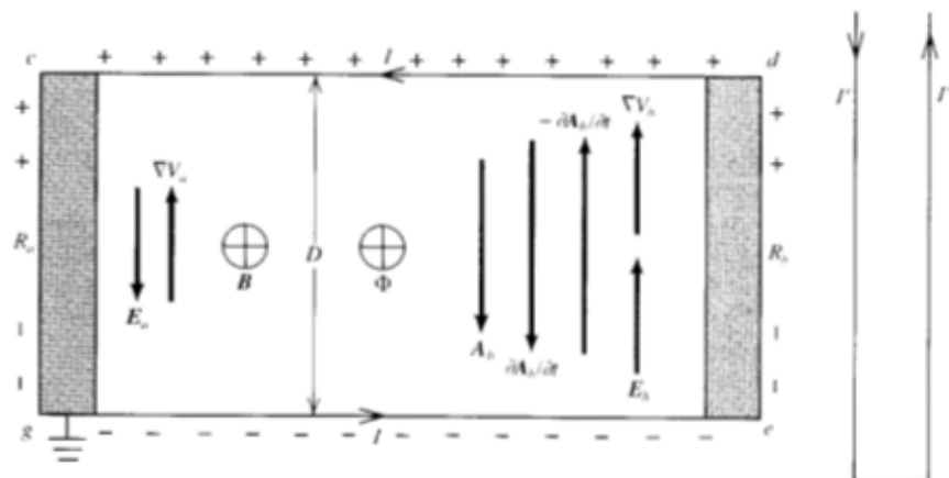
Fig. 23-8. Rigid circuit gcde terminated by resistances R_a and R_b and situated near a pair of wires carrying a current I' . The lengths of the arrows show the relative magnitudes of E , \nabla V , and \partial\mathbf{A}/\partial t , with R_a = R_b .
