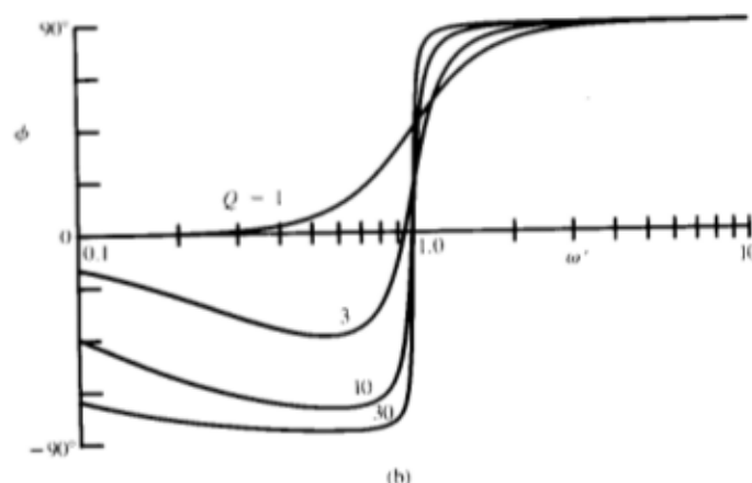
Fig. 25-4. (a) |Z|/R as a function of \omega' for the circuit of Fig. 25-3 for various values of Q . (b) The phase \phi of Z as a function of \omega' for the same values of Q .
