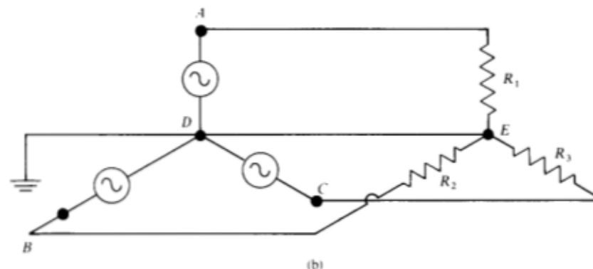
Fig. 7-10. (a) Three identical sources of alternating current, with phase differences of 120^\circ , feeding three resistors R_1 , R_2 , R_3 . (b) Three-phase supply. If the resistances are equal, the connection DE is unnecessary.
