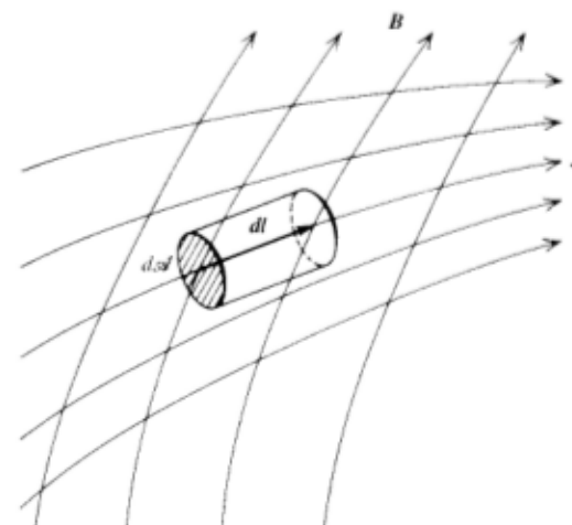
Fig. 22-9. Element of volume dv = dl da in a current distribution \mathbf{J} .
