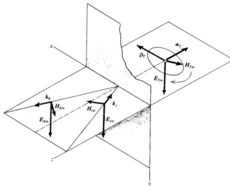
Fig. 31-6. The \mathbf{H} vector of the transmitted wave rotates in the direction shown. The transmitted wave travels to the left, and the rotation is the reverse of that of a wheel rolling on the interface.
