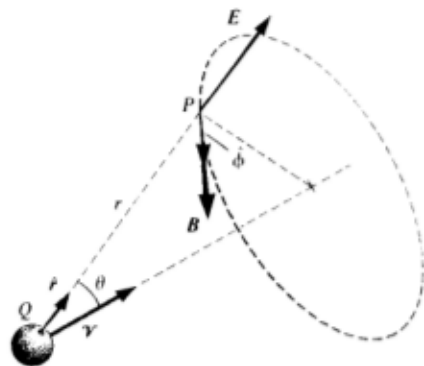
Fig. 16-3. The \mathbf{E} and \mathbf{B} vectors at a point P in the field of a charge Q moving at a constant velocity \mathbf{V} with respect to a reference frame S . The distance r and the angle \theta are both measured in S .
