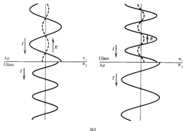
Fig. 30-4. (a) The relative phases, at the interface, of the E 's in the reflected and transmitted waves for n_1 < n_2 and for n_1 > n_2 , with E_{lm} normal to the plane of incidence. On the left, the reflected wave is \pi radians out of phase with respect to the incident wave. The transmitted wave is in phase, in both instances. (b) "Crests" of the field E at some particular time. The crests are one wavelength apart and travel in the directions of the arrows. Note the phase shift of \pi upon reflection from a glass surface. Note also the interference pattern that results from the superposition of the incident and reflected waves. (c) The E vectors at a given instant in the incident, reflected, and transmitted waves at normal incidence on a glass-air interface. On the right, E_{Tm} is larger than E_{Im} . However, conservation of energy still applies.
