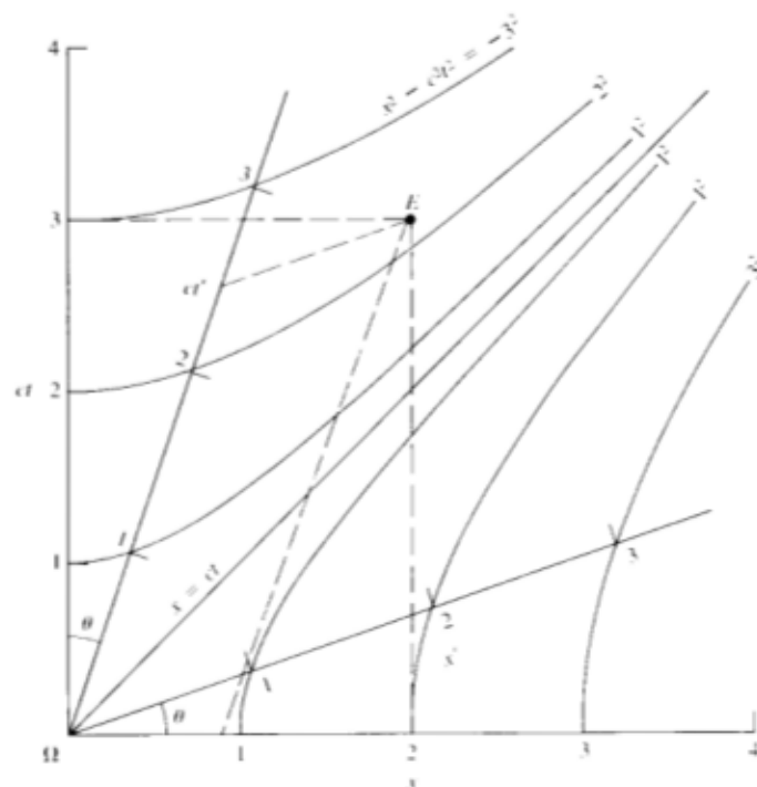
Fig. 13-4. The (x, ct) plane of reference frame S and, superimposed, x' - and ct' -axes for a reference frame S' that travels at a velocity 0.364c with respect to S . Thus \theta = 20.0^\circ and \gamma = 1.074 . The origins x = 0, t = 0 and x' = 0, t' = 0 coincide at O . Event E occurs at x = 2, ct = 3 , or at x' = 0.975, ct' = 2.44 . The curves are parabolas x^2 - c^2t^2 = \pm a^2 . This is a Minkowski diagram.
