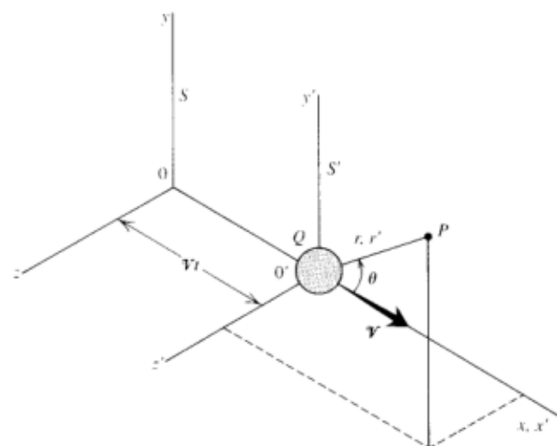
Fig. 17-2. The charge Q moves to the right at a velocity \mathbf{V} . We calculate \mathbf{A} and V at the point P . The distance QP is r in the fixed reference frame S , and it is r' in S' .
