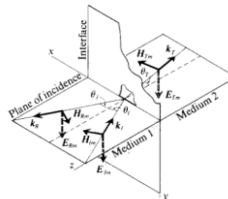
Fig. 30-2. The incident, reflected, and transmitted waves for an incident wave polarized with its E field normal to the plane of incidence. The arrows show the directions in which the vectors are taken to be positive at the interface. The vectors E \times H point everywhere in the direction of propagation.
