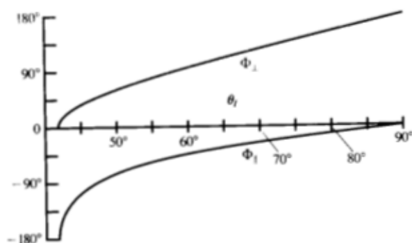
Fig. 31-2. The phases \Phi_{\perp} and \Phi_{\parallel} of the reflected wave with respect to the incident wave at a point on the interface, for total reflection when the E of the incident wave is normal and parallel to the plane of incidence. The ratio n_1/n_2 is equal to 1.50.
