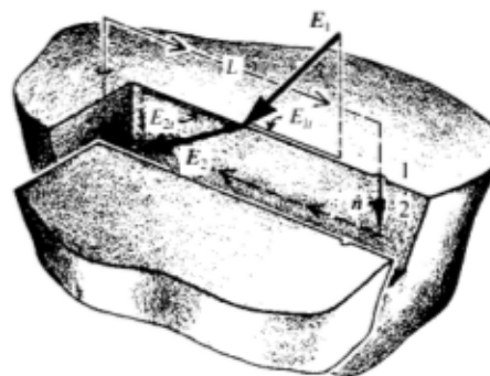
Fig. 10-5. Closed path of integration spanning the interface between media 1 and 2. The tangential components of \mathbf{E} are equal: E_{1t} = E_{2t} .
