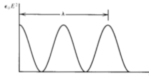
Fig. 28-3. The energy density \epsilon_0 E^2 , or \mu_0 H^2 , as a function of z , at t = 0 , for a plane wave travelling along the z -axis in free space.
