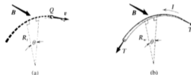
Fig. 22-6. (a) A positive charge Q moving at a velocity \mathbf{v} in a magnetic field \mathbf{B} . The radius of curvature of the trajectory is R_t . (b) Light wire carrying a current I in the opposite direction in the same magnetic field. The tension in the wire is T , and the radius of curvature is R_w . The two radii are equal if mv/Q is equal to T/I .
