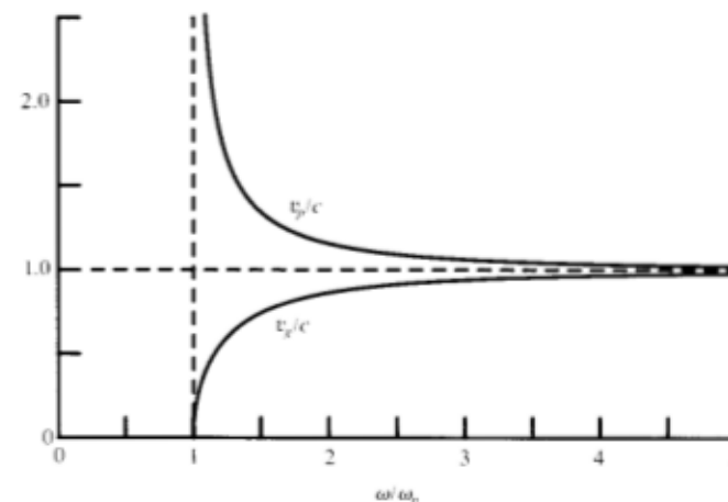
Fig. 29-4. The phase and group velocities v_p and v_g of an electromagnetic wave in a plasma.
