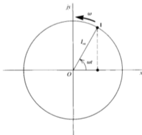
Fig. 2-2. Point I in the complex plane describes a circle of radius I_m about the origin O . It represents the phasor I_m \exp j\omega t . Its projection on the x -axis is I_m \cos \omega t .
