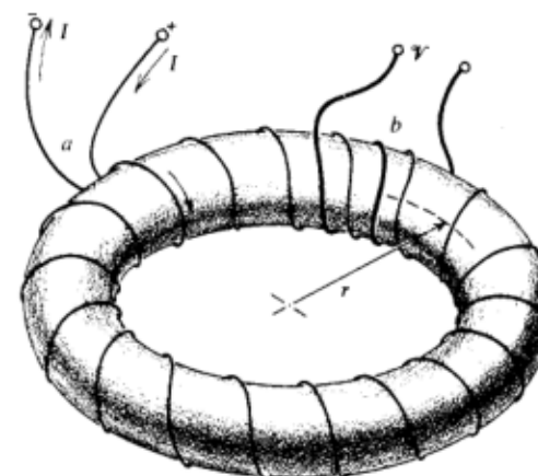
Fig. 21-1. Rowland ring for measuring B as a function of H in a ferromagnetic material. Winding a applies a uniform H . The voltage V across winding b gives B as in the first example in Sec. 23.4.2.
