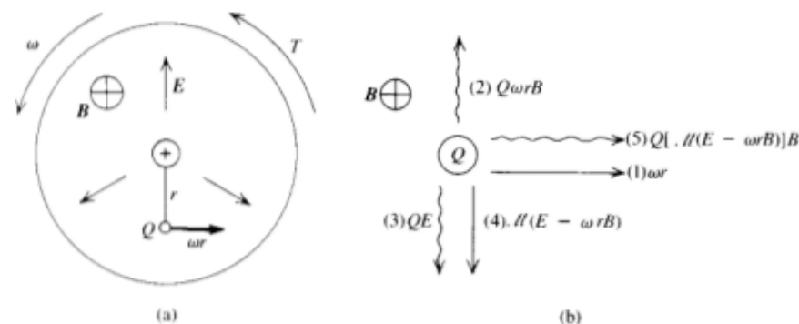
Fig. 22-11. (a) The rotor of a homopolar motor. The electric field is radial, while the magnetic field is axial. A charge carrier Q has an azimuthal velocity \omega r . (b) The velocity components of Q (straight arrows) and the various forces exerted on Q (wavy arrows).
