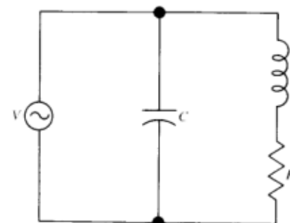
Fig. 25-3. Parallel-resonant circuit.
