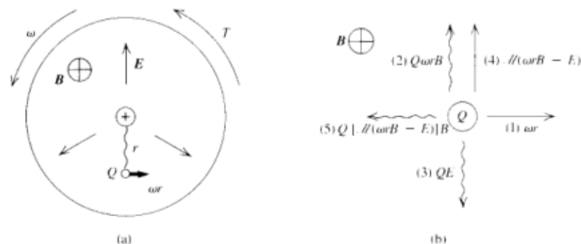
Fig. 22-12. This figure is similar to Fig. 22-11, except that it applies to a homopolar generator. (a) With \omega and B in the same directions as for the motor, the axle is positive and E is also in the same direction. (b) The product \omega r B is larger than E , and there is now a braking force (5).
