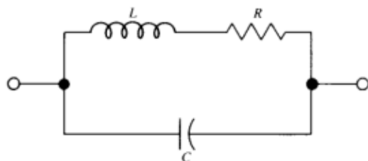
Fig. 24-6. The equivalent circuit of a real inductor. The parameters R , L , and C depend on the geometry and on the nature of the materials.
