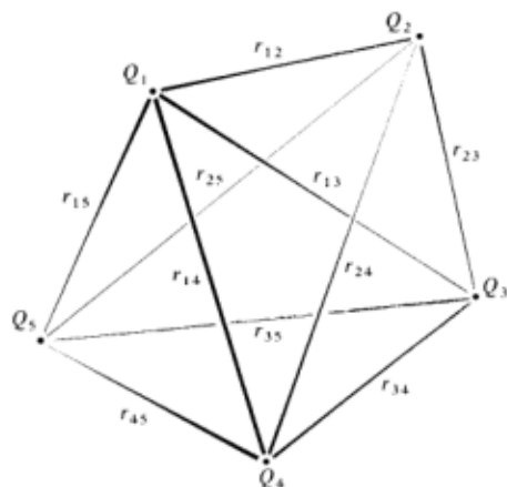
Fig. 6-1. Set of point charges Q_1, Q_2, Q_3, \dots separated by distances r_{12}, r_{13}, r_{14}, \dots .
