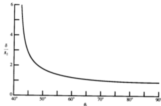
Fig. 31-3. The ratio \delta/\lambda_2 , where \delta is the depth of penetration for the transmitted wave and \lambda_2 is the wavelength in medium 2 divided by 2\pi , as a function of the angle of incidence \theta_i .
