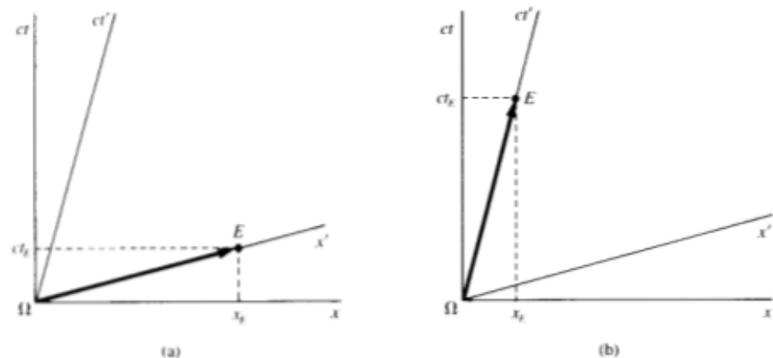
Fig. 15-2. (a) Event E occurs at y_E = 0 , z_E = 0 , and x_E > ct_E . It occurs at t' = 0 in a certain frame S' . (b) Event E occurs at y_E = 0 , z_E = 0 , and x_E < ct_E . It occurs at x' = 0 in some other frame S' .
