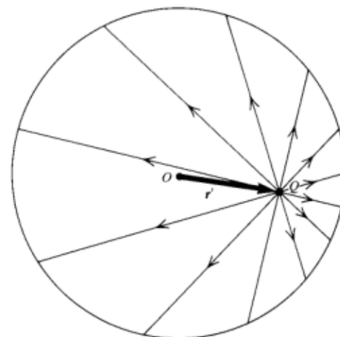
Fig. 3-9. Positive charge Q situated at r' inside an imaginary sphere. The average field of Q inside the sphere points in the direction opposite to r' .
