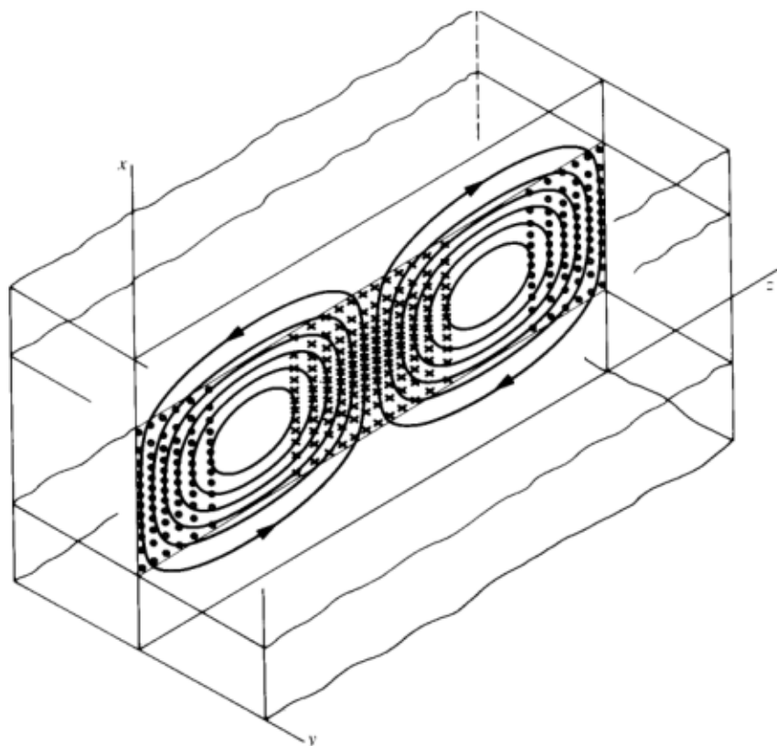
Fig. 36-4. Lines of E (dots and crosses) and of H for the symmetrical optical waveguide of Table 36-1. The wave travels from left to right. The figure does not show lines of E in media 1 and 3 because the electric field there is much weaker than in medium 2. Compare with Fig. 34-4.
