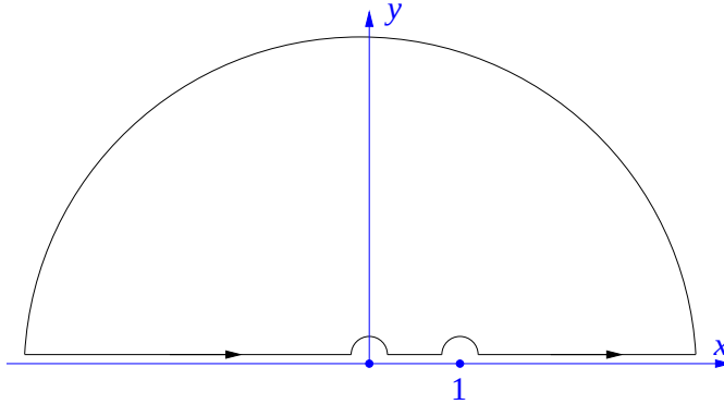
Figure 9.2: The contour \Gamma_1 .
