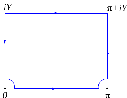
Figure 9.12: Indented rectangle.
