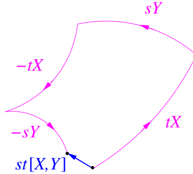
Figure 2.3: The Lie bracket.
