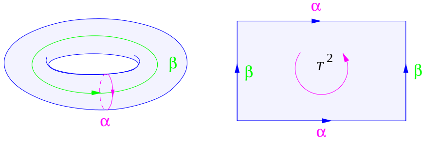
Figure 4.12: Cut-open torus
