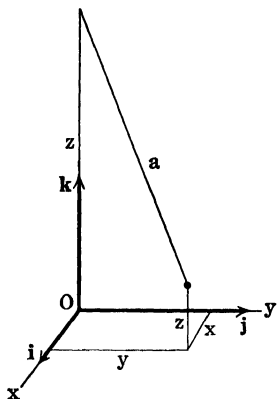
FIG. 134.—Spherical pendulum
