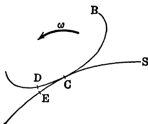
FIG. 63.—The body centroid B rolls on the space centroid S .
