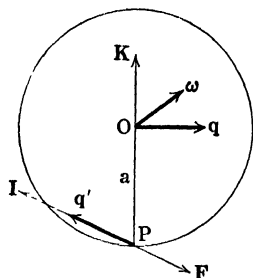
FIG. 157.—Ball slipping on a table.
