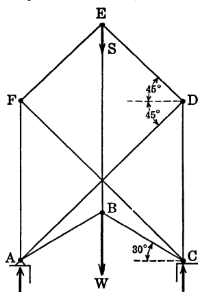
FIG. 56.—A complex frame.
