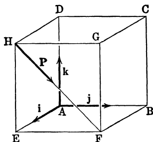
FIG. 104.—The moment of \mathbf{P} about A is required.
