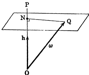
FIG. 145.—The invariable line and the invariable plane.
