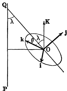
FIG. 156.—Vector diagram for gyrocompass.
