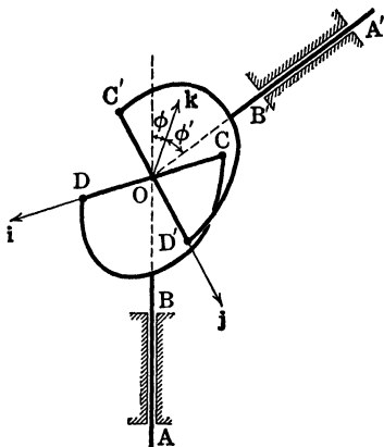
FIG. 119.—Hooke's joint.
