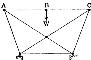
FIG. 57.—A critical form.
