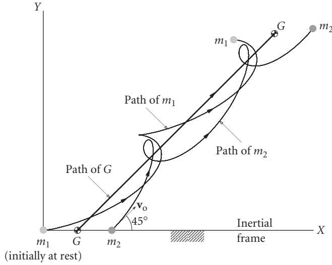
Figure 2.3 The motion of two identical bodies acted on only by their mutual gravitational attraction, as viewed from the inertial frame of reference.
