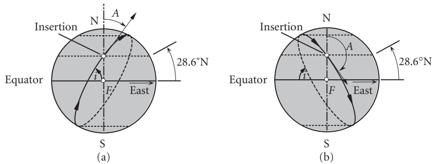
Figure 6.27 (a) Northeasterly launch ( 0^\circ < A < 270^\circ ) from a latitude of 28.6^\circ\text{N} . (b) Southeasterly launch ( 90^\circ < A < 270^\circ ).
