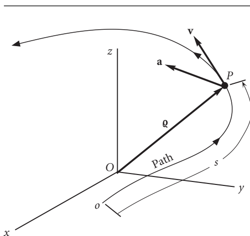
Figure 1.1 Position, velocity and acceleration vectors.
