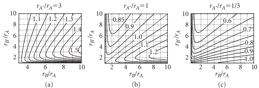
Figure 6.5 Contour plots of \Delta v_{\text{total}}^{(3)}/\Delta v_{\text{total}}^{(3)} for different relative sizes of the ellipses in Figure 6.4. Note that r_B > r_{A'} and r_B' > r_A .
