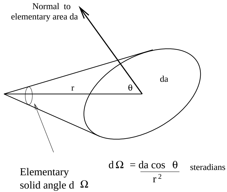
Figure 2.2: Solid angle.
