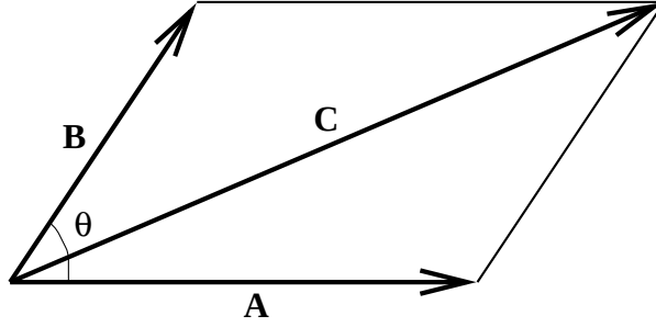
Figure 2.3: Vector addition.
