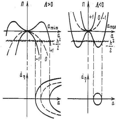
Fig. 5.4. – a) \Lambda > 0 , b) \Lambda < 0 . At the top, the potential energy (5.69); a_{\text{mim}} = \sqrt{3/\Lambda} , a_{\text{mam}} = \sqrt{6/|\Lambda|} ; the numbers of the curves indicate the type of space, k = -1, 0, 1 . At the bottom, the phase plane of Eq. (5.66).
